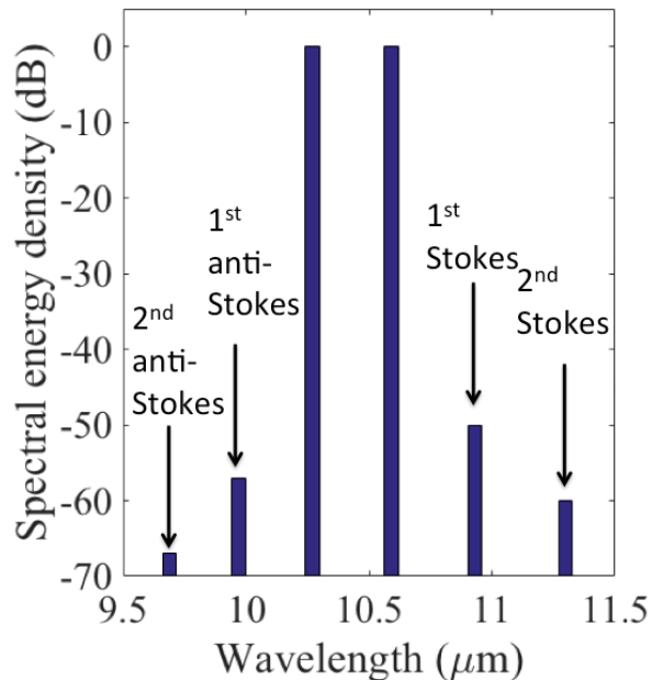
Figure 7: A typical FWM spectrum obtained in 380 torr of laboratory air.
