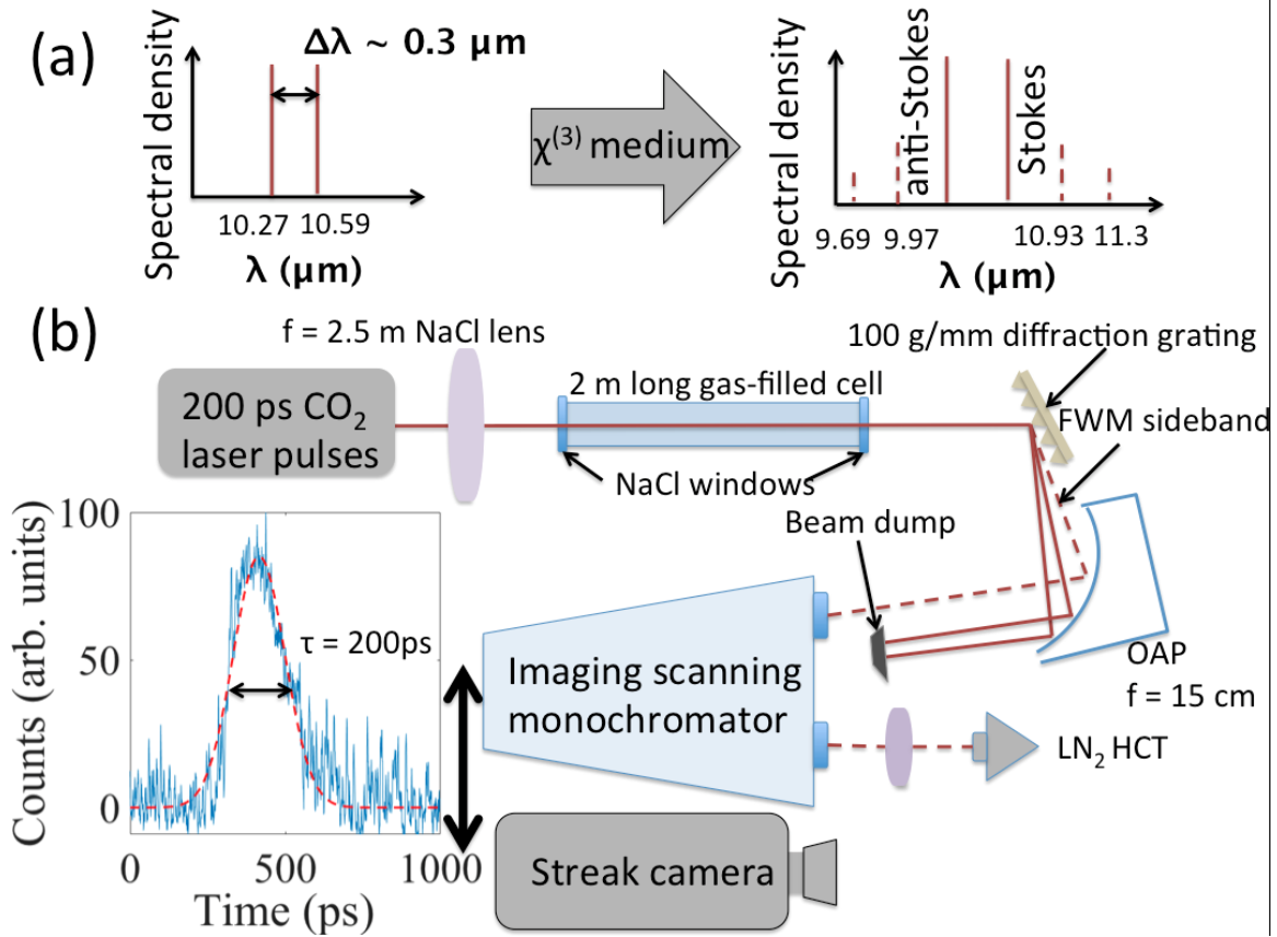
Figure 1: (a) A dual-wavelength laser pulse is transformed into a family of sidebands by FWM in a nonlinear medium. (b) Experimental set-up for nonlinear refractive index measurements of gases. The inset shows a representative temporal pulse profile used for nonlinear refractive index measurements. OAP stands for off-axis parabolic mirror and HCT stands for HgCdTe detector.
