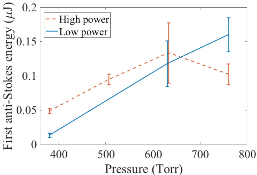
Figure 3: Energy of the first anti-Stokes sideband as a function of pressure in laboratory air. The dashed and solid lines were produced using 200 and 130 MW, respectively.
