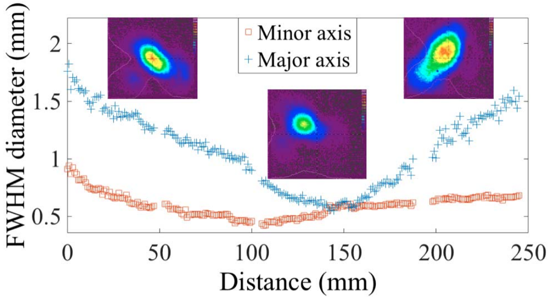
Figure 2: The evolution of the major and minor diameters of the elliptical beam used for nonlinear refractive index measurements in gases. The insets of the figure show example images of the beam as measured with a pyroelectric camera.
