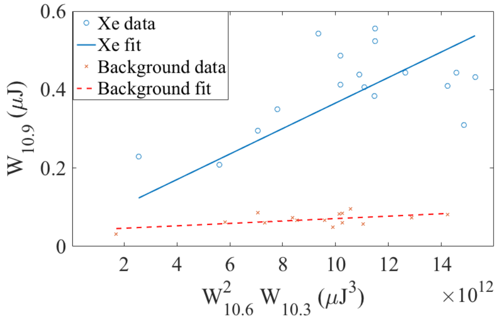
Figure 5: Energy in the first Stokes sideband plotted as a function of the energy of the 10.6 \mu\text{m} pump squared times the energy in the 10.3 \mu\text{m} pump for 380 torr of Xenon gas. Note that W_{10.6}^2 W_{10.3} is the energy of the laser pulse.
