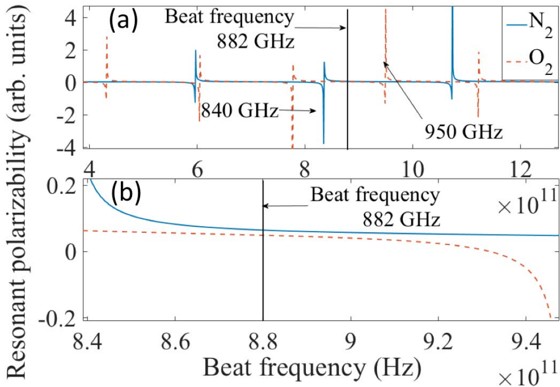
Figure 8: (a) The resonant third-order polarizability of N_2 and O_2 in the range of 400 to 1200 GHz and (b) zoomed in the vicinity of the 882 GHz beat-frequency used for nonlinear refractive index measurements.
