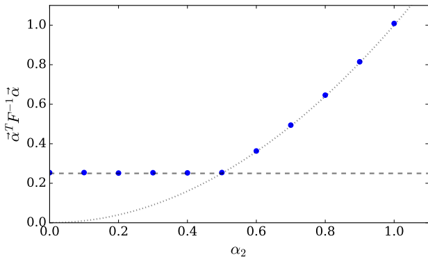
FIG. 2. Numerical optimization of \alpha^T F_Q^{-1} \alpha for two qubits with \alpha_1 = 1 compared to the bound predicted by our analytic result. Each point is generated by running a gradient descent algorithm until convergence; the control parameters begin at small random values. The dashed (dotted) line is the analytic bound derived from the first (second) qubit. As \alpha_2 increases, the second qubit becomes the source of the relevant bound.
