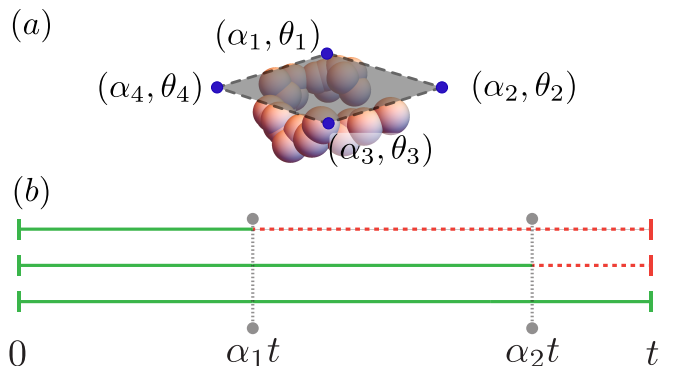
FIG. 1. (a) An illustration of the network setup in a nanoscale NMR setting. Nodes, located at different points relative to a large molecule, share an entangled state; at each node there is both an unknown parameter \theta_i and a known relative weight \alpha_i . We are concerned with estimating \alpha \cdot \theta . (b) Illustration of the partial time evolution protocol for three qubits. Solid green segments of the timeline represent periods when a qubit is evolving due to coupling to the local parameter \theta_i , while dashed red segments represent periods after the qubit stops evolving. The switches occur at times corresponding to the qubits’ weights in the final linear combination. The weight of the last qubit is \alpha_3 = 1 .
