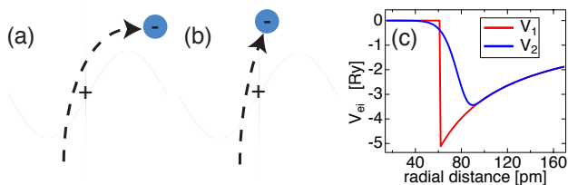
FIG. 6. An electron absorbing energy from an optical field in the presence of ion represented by a pseudo-potential of the nucleus and bound electrons with a small (a), and large (b) cut-off radius. Shielding of the nucleus by the bound electrons is represented by the cutoff radius, r_c , which determines the range of potentials the electron can interact with. The pseudo-potential approach to treating the electron-ion potential near the bound (core) electrons, for a sharp cut-off radius V_1 (sharp red), and a soft cut-off V_2 (smooth blue) according to Eq. 3 is shown in (c).
