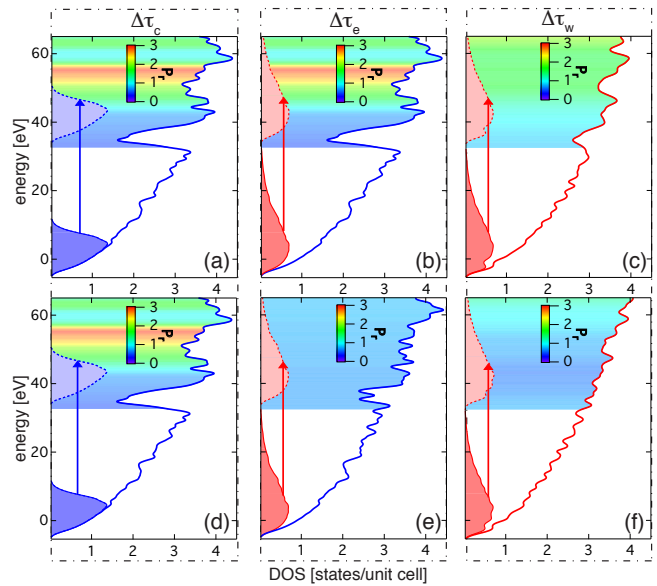
FIG. 8. DFT calculations of the density of states (DOS) (solid lines), electron transitions for 39 eV photons (arrows) and transition probabilities, P_r (colour-scale shading). The calculations correspond to the three temporal regions of interest ( \Delta\tau_c , \Delta\tau_e and \Delta\tau_w ) shown in 7 (top arrows). The \Delta\tau_c region corresponds to cold electrons in a cold lattice, the \Delta\tau_e phase corresponds to T_e=6 eV in a cold lattice, and \Delta\tau_w corresponds to T_e = 6 eV and T_i = 2 eV. Standard DFT calculations are shown in a, b and c that correspond to the DFT points in Fig. 7. The DFT+ U calculations are shown in d, e and f correspond to the DFT+ U points in Figs. 5 and 7 and .
