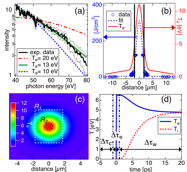
FIG. 2. The smoothed time integrated XUV plasma emission measurement (solid noisy black line) with error bars (dashed light black lines), and the best fit with a peak electron temperature of T_e = 13 \pm 3.25 eV (solid green line) (a). The measured fluence profile of the XFEL spot on target (blue circles) and fit (dashed blue line) which is used in the TTM to calculate the temperature profile across the target (solid red line, a 0.5 \mu\text{m} width line-out) (b). The solid black lines indicate the borders of the probed region R_1 in (c). The calculated 2D peak electron temperature profile using the measured beam fluence profile (c). The dashed lines in (c) enclose the area probed by the XUV pulse R_1 , and the area that dominates the XUV emission spectrum R_2 in (a). The calculated spatial average of the electron (solid blue) and ion (dashed red) temperatures in time of the probed area, R_1 , from the TTM are shown in (d). The three timescales of interest are shown in (d) (arrows and dashed-dot lines); \Delta\tau_c is the cold solid foil, \Delta\tau_e is the timescale of electron heating only, and \Delta\tau_w is the timescale of electron-ion coupling.
