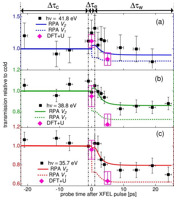
FIG. 5. Spectrally resolved relative transmission through the XFEL heated foil for the three photon energies of 41.8 eV (a), 38.8 eV (b) and 35.7 eV (c) used in this study. The calculated relative transmission for the temperatures in the probed region ( R1 in Fig. 2c) for the electron-ion potential V_1 (dashed line) and V_2 (solid line) is shown for each photon energy. The three timescales of interest are shown (arrows and dashed-dot lines) \Delta\tau_c is the cold solid foil, \Delta\tau_e is the timescale of electron heating only, and \Delta\tau_w is the the timescale of electron-ion coupling. The results of DFT+U calculations are shown for the \Delta\tau_e and \Delta\tau_w timescales of interest and discussed in Section VI.
