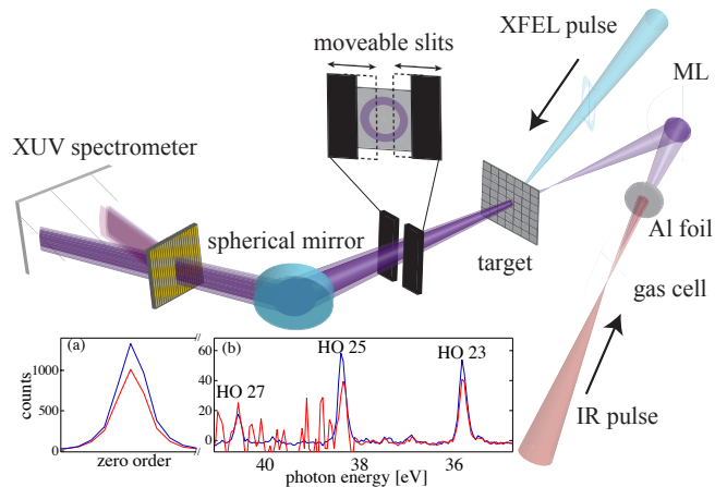
FIG. 1. The experimental arrangement for the measurement of XUV absorption in an XFEL heated aluminium foil. A 40 fs IR pulse at a wavelength of 800 nm and intensity \sim 10^{15} W cm ^{-2} is focussed into a gas cell of 1.5 cm in length and filled with argon (Ar) at a pressure of 30 mbar to generate high-order harmonics in the XUV. The XUV beam is then focussed by a multilayer mirror (ML) near the target plane. The XUV pulse is partially transmitted through the foil, and the remaining XUV light is absorbed. An adjustable slit is placed after the target to block the XUV light that does not pass through the plasma. The absorption of 3 high harmonics through the foil target is measured using an XUV spectrometer. A typical spectrum transmitted through the cold (blue) and heated (noisy red) aluminium foil is shown in the inset. By dividing the red by the blue, we can extract the transmission relative to cold at three photon energies. Spectra transmitted through the foil were measured at different times with respect to the peak of the XFEL. The measured relative transmission time histories are plotted in Figs. 4 and 5. The zero order (a), and spectrally resolved (b), regions are separated for clarity in the inset. The noise in the plasma shot in inset b is due to scattered hard x-rays. The harmonic order (HO) of the three photon energies is shown in the inset b.
