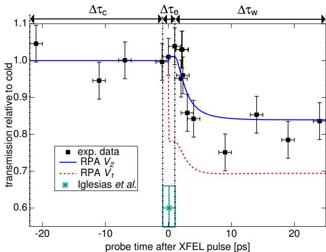
FIG. 4. The experimental transmission of zero order (all harmonics) relative to cold of a 600 nm aluminium foil heated by an XFEL pulse (black squares). The time axis is relative to the peak of the XFEL pulse. Calculated transmission values for the electron-ion potential V_1 (dashed red) and V_2 (solid blue), for the average transmission of the probed region are shown. A delay in electron-ion coupling is incorporated into the TTM to give a heating rate in agreement with other studies (detailed in Section III). A semi analytic model by Iglesias et al. [9] predicting changes due to electron heating is shown in the \Delta\tau_e phase (boxed green star). The three timescales of interest are shown (arrows and dashed-dot lines) \Delta\tau_c is the cold solid foil, \Delta\tau_e is the timescale of electron heating only, and \Delta\tau_w is the timescale of electron-ion coupling.
