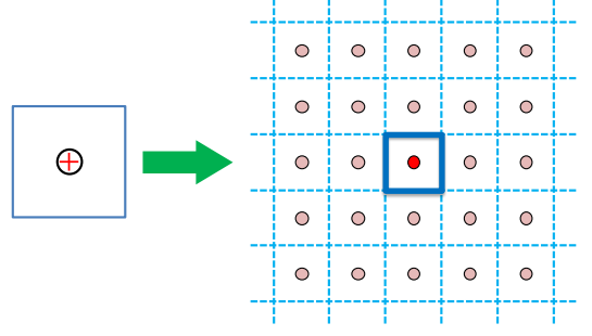
Figure 1. (Color online) Demonstration for the boundary condition of Eq. (17). The influence of the periodic boundary condition can be equivalently replaced by the point “charge” lattice in free space, which is similar like the method of image charges.
