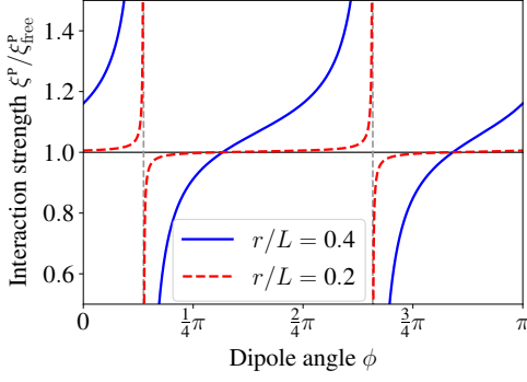
Figure 2. (Color online) Numerical estimation for the dipole-dipole interaction strength in a finite volume [Eq. (19)] comparing with the free space result. Here as an example, we choose \hat{\mathbf{e}}_r = (1, 2, 3)/\sqrt{14} , and set the two dipoles parallel to each other in the direction \hat{\mathbf{e}}_{1,2} = (\cos \phi, 0, \sin \phi) . When r/L is large, the correction from the boundary effect is significant. It turns out Eq. (19) converges quite fast, and only very few “image” terms is needed ( |n_{x,y,z}| \lesssim 2 ) to get a precise enough result, which means only the nearest “image” dipoles are important.
