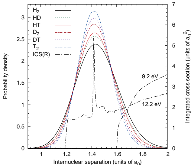
FIG. 8: Probability density functions of the ground vibrational state for \text{H}_2 and its isotopologues. The R -dependent excitation cross sections of the b^3\Sigma_u^+ state at 9.2 and 12.2 eV are also shown.
