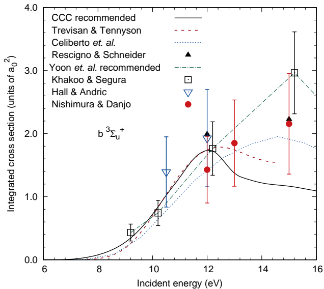
FIG. 4: Electron impact excitation cross section of the b^3\Sigma_u^+ state of H_2 . The recommended CCC cross section is compared with the calculations of Trevisan and Tennyson [16], Celiberto et al. [17], and Rescigno and Schneider [18], the measurements of Khakoo and Segura [7], Nishimura and Danjo [6], and Hall and Andric [8], and the recommended data of Yoon et al. [9].
