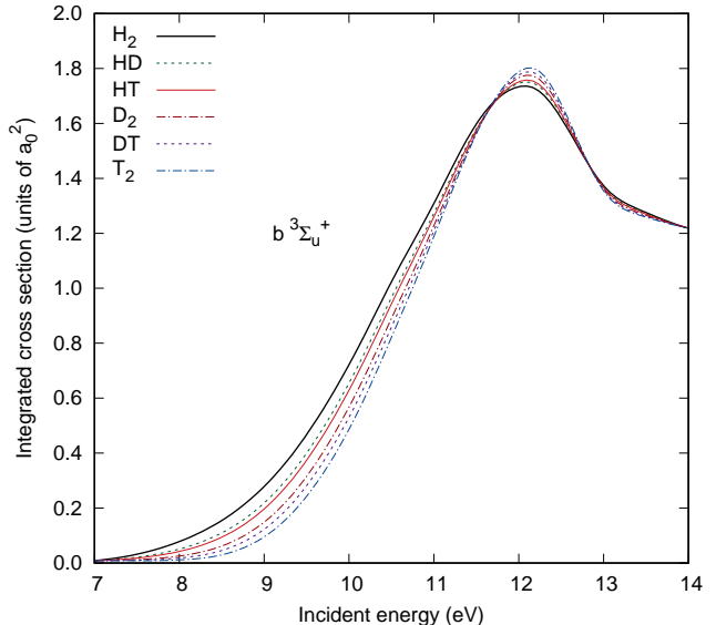
FIG. 9: Electron impact excitation cross section of the b^3\Sigma_u^+ state of \text{H}_2 , \text{D}_2 , \text{T}_2 , \text{HD} , \text{HT} , and \text{DT} , calculated using the AN CC(12) model described in the text.
