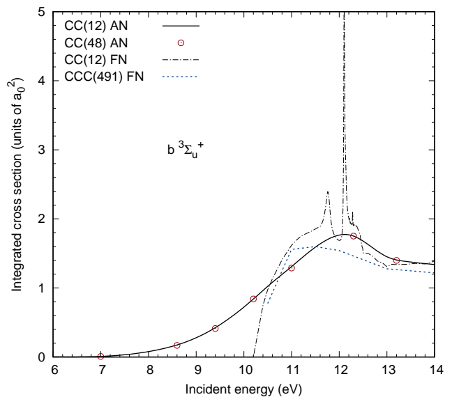
FIG. 2: Electron impact excitation cross section of the b^3\Sigma_u^+ state of H_2 . Convergence is demonstrated for the AN CC(12) and CC(48) models described in the text. The FN CCC(491) and CC(12) calculations performed at R = 1.448 are also presented.
