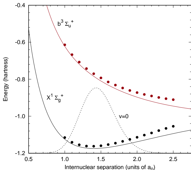
FIG. 1: Potential energy curves of the X^1\Sigma_g^+ and b^3\Sigma_u^+ states of H_2 obtained from structure calculations performed in the present scattering calculation model (points), compared with the accurate calculations (solid lines) of Kolos et al. [37] ( X^1\Sigma_g^+ ) and Staszewska and Wolniewicz [38] ( b^3\Sigma_u^+ ). The ground (electronic and vibrational) wave function of H_2 is also shown (dashed line).
