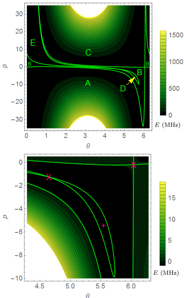
Figure 10: We include the phase portrait for \omega = 0.13 and \gamma = 1 (in the regime with three fixed points), with a complete picture (top) and reduced range to zoom in on the features of greatest interest (bottom). Two of the fixed points are hyperbolic (pink \times ), at (\bar{\theta} = 6.04, \bar{p} = -0.201) and (\bar{\theta} = 4.63, \bar{p} = -1.25) , and one is elliptical (pink + ), at (\bar{\theta} = 5.55, \bar{p} = -5.63) . The latter two points are responsible for partitioning off the new regions D and E inside region B. Periodic paths are possible within the island D, which is bounded by a separatrix of energy E_s = -0.938 MHz. We note that for smaller \omega compared with Fig. 7, we have a larger region B which now encroaches asymmetrically into A (making winding-number MMLPs less likely), and the region C has grown (indicating that it is easier for trajectories to travel against the weaker Rabi drive).
