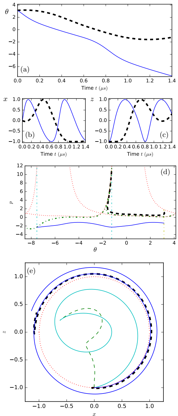
Figure 9: We show MMLPs with different winding numbers, from \theta_i = \pi to either \theta_f^{(B)} = -1.24 (thick dashed black) or \theta_f^{(A)} = -1.24 - 2\pi (solid blue). These are shown as \theta(t) (a), x(t) and z(t) (b,c), and in phase space (d). In the phase space plot we show \theta_i in dash-dotted yellow (the Lagrangian manifold at t = 0 ), the two \theta_f in dash-dotted cyan, the separatrix in dotted red, and the Lagrangian manifold at T = 1.4 \mu s in dash-dotted green. Finally, in (e) we show the pure state paths (still solid blue and thick dashed black) in the xz -plane of the Bloch sphere. The dotted red line marks the edge of the sphere; the pure-state curves are given an artificial radius outside the sphere for added visibility. The solid cyan and thin dashed green curves in (e) are the theory calculations for the example with \eta = 0.45 from Figs. 4 and 5 of the main text, shown for comparison.
