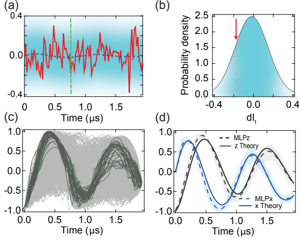
Figure 2: Path probability and most likely paths. (a), Demonstration of path-probability calculation. The blue (dashed) curve indicates \sqrt{\eta\gamma}x dt which determines the probability distribution (blue background color) for a corresponding homodyne signal (red solid curve). (b), A cross-section of the probability density at the time indicated by the long-dashed green line of (a). The Gaussian distribution is shifted from zero by \sqrt{\eta\gamma}x dt . The arrow shows the value of homodyne signal at that point. (c), The pre- and post-selected trajectories for initial \{z(0), x(0)\} = \{-0.97, 0\} and final \{z(1.94 \mu\text{s}), x(1.94 \mu\text{s})\} = \{-0.3, -0.6\} boundary condition (only z traces are shown). The top five percent of which have lowest Euclidean distance from others are highlighted in black. (d), Solid black line originating from -0.97 is the theoretical MLP for z obtained from Eqs. (6). The solid blue line originating from 0 is the theoretical MLP for x . The dashed lines are the corresponding experimental MLP obtained by averaging the highlighted trajectories. The shaded area along experimental curves shows the standard deviation of the averaged trajectories (see Appendix E for statistical information).
