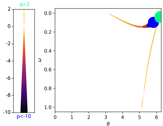
Figure 8: We plot the locations of fixed points \bar{\theta} against the dimensionless parameter \omega = \Omega/\gamma . Color and size denote the momentum \bar{p} . Experimentally we operate at \omega = 0.63 \cdot 2\pi , where there is only one fixed point. This fixed point is a location in the phase space where the Rabi drive and fluorescence cancel. Another pair forms for \omega < 0.145 = \omega_c , splitting around \theta = 5.18 . As the drive is eliminated entirely, these show system is able to stall at either the ground ( \theta = 0 or 2\pi ) or excited ( \theta = \pi ) states. All fixed points exist on the half of the Bloch sphere where the fluorescence and drive compete (the drive pushes the state from ground to excited, whereas the fluorescence pushes the state from excited to ground); none exist on the half where the fluorescence and drive work together (both push towards the ground state), indicating that no optimal readout can fight both the drive and spontaneous emission at the same time to hold the system still at some particular state.
