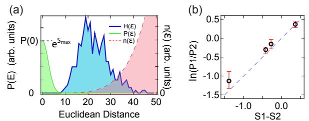
Figure 6: Relative probability of multiple most likely paths. (a), The peak of the probability density distribution of the Euclidean distance from the MLP (green, left distribution) is related to the extremum of the stochastic action ( S_{\max} ). The observed distribution (blue, center distribution) has a maximum that shifted from 0 due to the increasing multiplicity of trajectories (right distribution) with a larger Euclidean distance from the MLP. (b), To compare the experimental distributions to the theoretical stochastic entropy maxima, we use the multiplicity ( n(\mathcal{E}) ) and observed distribution H(\mathcal{E}) to determine P(0) . We compare the relative probability ( P(0)_{\text{cluster1}}/P(0)_{\text{cluster2}} ) to the predicted relative probability S_1 - S_2 . Error bars indicate the uncertainty in the fit to the relative distribution (see Appendix E for statistical information). We apply this analysis to 4 different MMLP pairs with initial state \{z(0), x(0)\} = \{-0.97, 0\} and final states \{z(T), x(T), T(\mu\text{s})\} = \{0.65, -0.08, 1.2\} , \{0.19, -0.93, 1.4\} , \{0.36, 0.47, 1\} , \{0.21, -0.62, 1.4\} , (left to right on graph).
