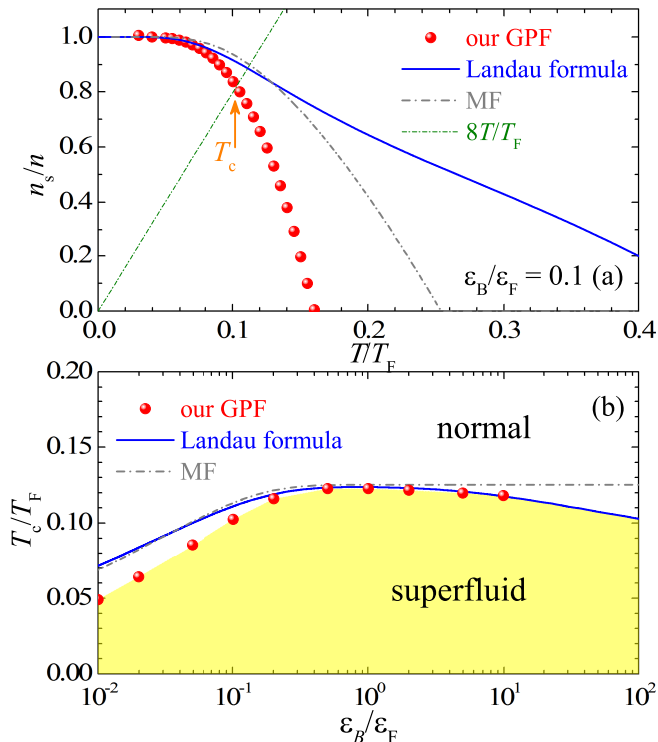
Figure 4. (color online). (a) The superfluid fraction as a function of temperature at interaction strength \epsilon_B = 0.1\epsilon_F . Our GPF prediction (red circles) is compared with the mean-field result (grey dot-dashed line) and the approximated result based on the zero-temperature GPF (blue solid line) [46]. The intersection with the curve 8T/T_F determines the BKT transition temperature. (b) The critical temperature as a function of \epsilon_B/\epsilon_F .
