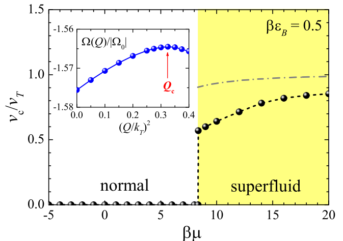
Figure 5. (color online). The critical velocity v_c , in units of the thermal velocity v_T \equiv [k_B T / (2M)]^{1/2} = \hbar k_T / (2M) , as a function of \beta\mu at the interaction strength \beta\epsilon_B = 0.5 . The black circles (with dashed line) and the grey dot-dashed line show the GPF and mean-field predictions, respectively. The inset shows the thermodynamic potential at nonzero superfluid velocity v = \hbar Q / (2M) , which exhibits a local maximum at v_c .
