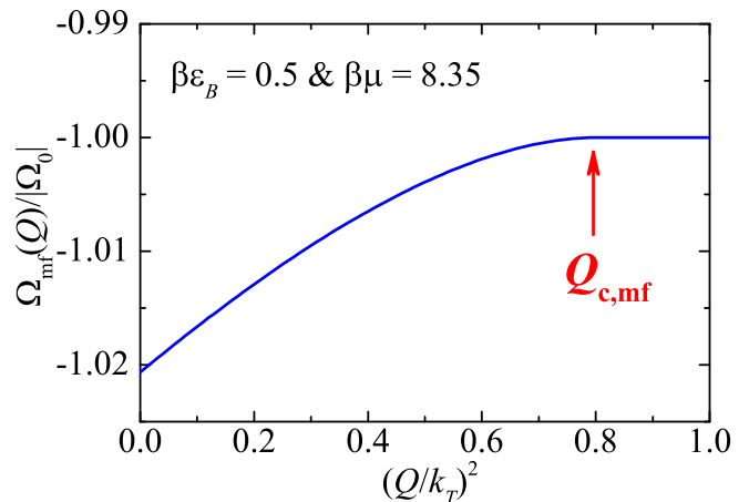
Figure 6. (color online). The mean-field thermodynamic potential at nonzero superfluid velocity v = \hbar Q/(2M) , which saturates to the ideal gas thermodynamic potential \Omega_0 at the pair-breaking velocity v_{pb} . Here we take \beta\varepsilon_B = 0.5 and \beta\mu = 8.35 .
