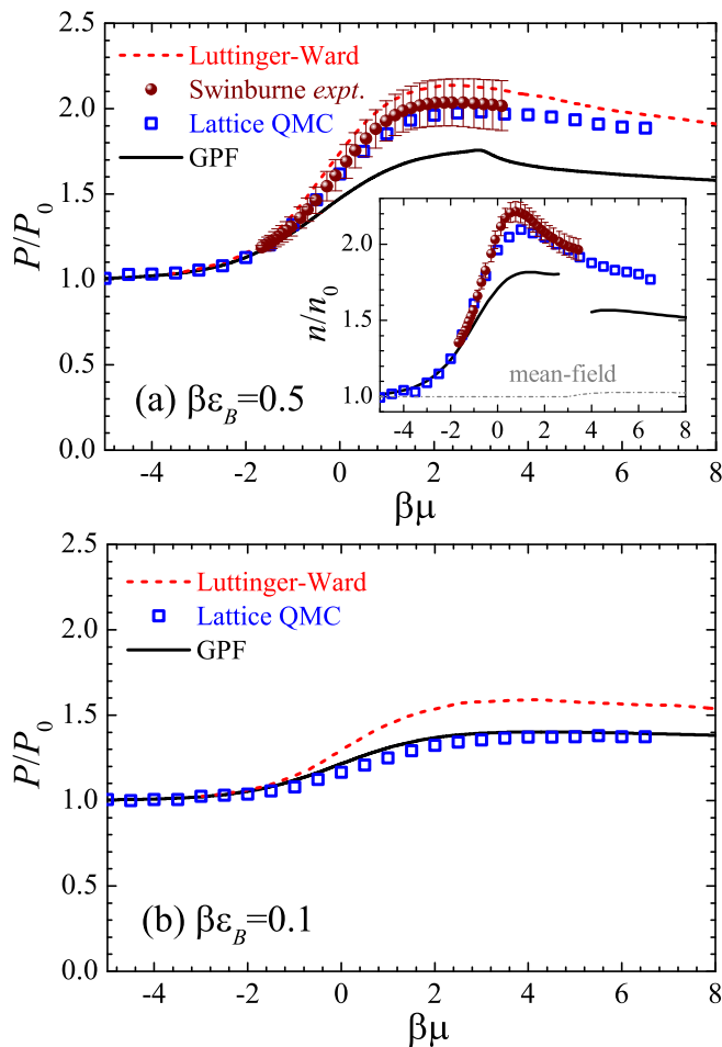
Figure 1. (color online). (a) Pressure equation of state at \beta\varepsilon_B = 0.5 where P = -\Omega/V . The prediction from the GPF theory (black solid line) is compared with the results from the Luttinger-Ward theory (red dashed line) [42, 45] and lattice QMC simulation (blue squares) [47], and the experimental data from Swinburne [33] (solid circles with error bar at a slightly smaller \beta\varepsilon_B = 0.47 ). The inset shows the density equation of state at the same interaction strength. (b) Pressure equation of state at \beta\varepsilon_B = 0.1 , where the Fermi gas remains normal up to \beta\mu = 8 . Here, P_0(\mu) and n_0(\mu) are the pressure and density of an ideal Fermi gas, respectively.
