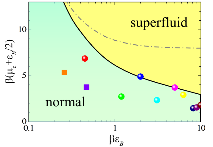
Figure 3. (color online). The critical chemical potential (with \varepsilon_B/2 added) as a function of the interaction strength. The black solid line and the grey dot-dashed line show the GPF and mean-field results, respectively. The symbols (in different colors) show the largest chemical potential achieved in the recent density equation of state measurements [33, 34], at different interaction strengths.
