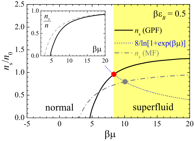
Figure 2. (color online). The superfluid density, in units of the density of an ideal Fermi gas n_0 , as a function of the chemical potential at the interaction strength \beta\varepsilon_B = 0.5 . The GPF and mean-field predictions are shown by the black solid and grey dot-dashed lines, respectively. The circles indicate the critical superfluid density (or chemical potential) for the BKT transition. The inset shows the superfluid fraction n_s/n .
