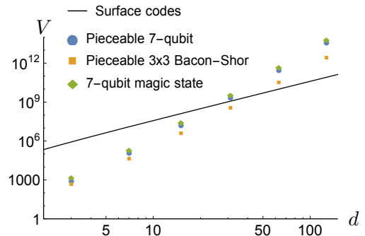
FIG. 3. Circuit volume for logical 3-qubit gate on pieceable 7-qubit code (circles), pieceable 3 \times 3 Bacon-Shor code (squares), and magic-state scheme on 7-qubit code (diamonds) in terms of code distance. The dots correspond to every concatenation level in the range. Although it may be hard to see the data for the magic-state scheme, the pieceable 7-qubit has slightly lower volume than the magic-state scheme for every distance shown.
