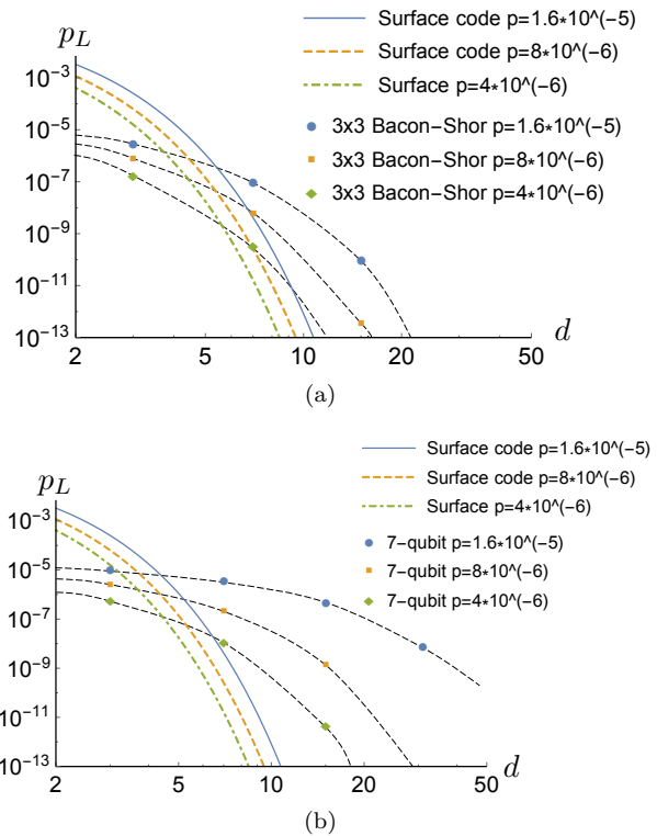
FIG. 2. Logical error rates for 3-qubit gate on the surface codes and (a) pieceable 3 \times 3 Bacon-Shor code (b) pieceable 7-qubit code in terms of code distance. Shown rates for pieceable codes are upper bounds obtained by concatenating the upper bounding function from Eq. (7). Black dashed curves are only a guide to the eye.
