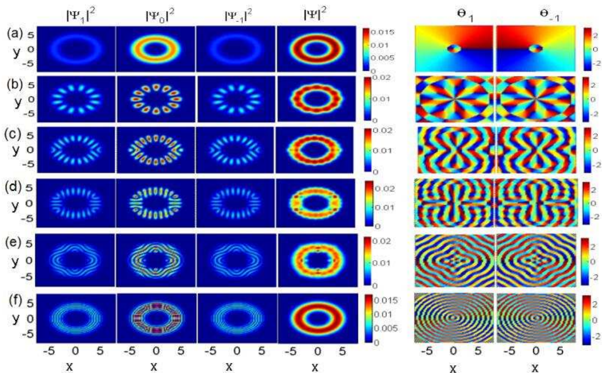
FIG. 2: (Color online) Left panels: The ground-state density profiles of the m_F = 1 component, the m_F = -1 component, and the m_F = 0 component. Right panels: the phases of the m_F = \pm 1 components. The relative interaction strength g = 5 and the toroidal trap radius r_0 = 4 . From (a) to (f), the SOC strength is respectively taken as \lambda = 0.25, 1.6, 2.4, 3, 4, 6.4 which correspond to the phases of (A)-(F) in Fig. 1(a).
