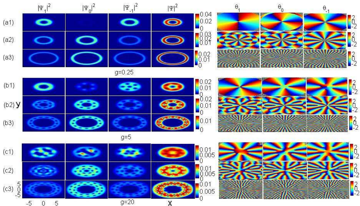
FIG. 6: (Color online) The ground-state density and phase profiles for the m_F = 1 , m_F = 0 , and m_F = -1 component. The rotational frequency \Omega = 0.5 and other parameters are the same with Fig.4.
