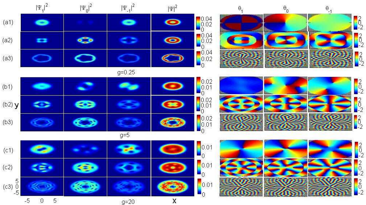
FIG. 5: (Color online) The ground-state density and phase profiles for the m_F = 1 , m_F = 0 , and m_F = -1 component. The rotation frequency \Omega = 0.25 and other parameters are the same as in Fig.4.
