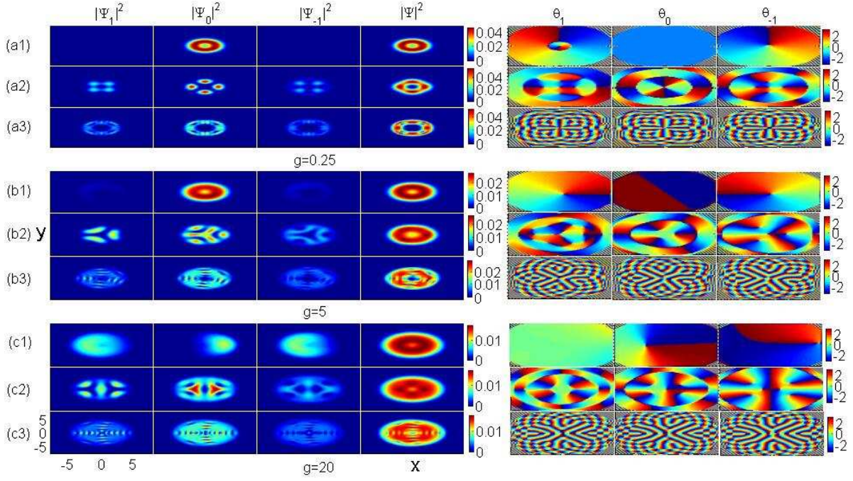
FIG. 4: (Color online) The ground-state density and phase profiles for the m_F = 1 , m_F = 0 , and m_F = -1 component for the SOC strengths ( \eta_1 ) \lambda = 0.1 , ( \eta_2 ) \lambda = 1 and ( \eta_3 ) \lambda = 4 ( \eta = a, b, c ), respectively. The relative interaction strengths (al) g = 0.25 , (bl) g = 5 and (cl) g = 20 , ( l = 1, 2, 3 ). The toroidal trap radius r_0 = 2 and the rotation frequency \Omega = 0.1 .
