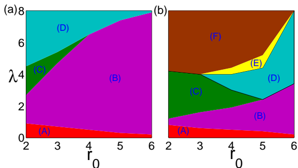
FIG. 3: (Color online) The ground-state phase diagram spanned by the SOC strength \lambda and the toroidal trap radius r_0 without the quadratic Zeeman shift ( q = 0 ). The relative interaction strength g = 0.67 in (a) and g = 5 in (b), respectively.
