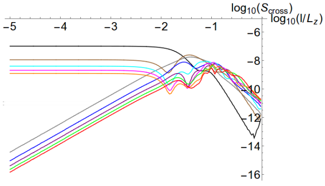
FIG. 9: Cross-noise (arbitrary units) along x -motion for a chain of 10 strongly coupled ions when dipoles in the surface are pointing along x , as a function of the inter-ion distance l \in [10^{-5}L_z, L_z] . The electrode has dimensions L_x = 10L_z and the ions are above the electrode at d = L_z . Black line is the mode with longest wavelength.
