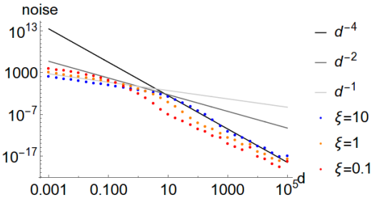
FIG. 7: Noise felt by 1 ion oscillating along x when dipoles in the surface are pointing along y , with spatial dipole-dipole correlation distance \xi . The typical scaling d^{-4} is broken for ion-electrode distances d < \xi , where it becomes d^{-1} . Distance is given in arbitrary units.
