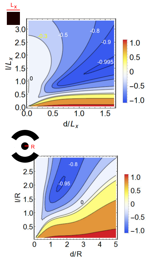
FIG. 5: Noise ratios S_{\text{cross}}/S_{\text{self}} for the x -motion of 2 ions above two different geometries, with homogeneous distribution of dipoles pointing normal to the surface: (Top) square electrode L_x = L_z , when the rest of y = 0 plane is dielectric (or empty), and (Bottom) a stylus trap as in [15] with inner disk electrode of radius R and an outer ring from 3R to 5R ; further apart there are 4 disks, but for the distances considered here they do not affect the ions; the spaces between electrodes act as empty spaces.
