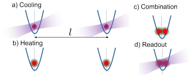
FIG. 3: Experimental sequence. - The four radial normal modes of motion of a two-ion system are first cooled close to the ground state [33]. After being exposed to interactions with the environment, the ions are combined in a common potential well. There the motional states of all four modes are read by coupling to the internal electronic states [34], giving access to the desired normal modes' heating rates \Gamma_\pm .
