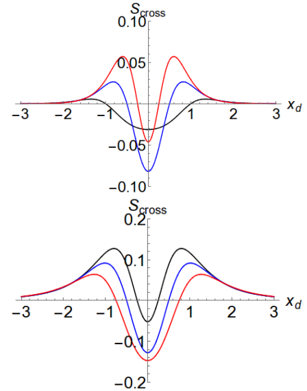
FIG. 4: (Top) Spatial dependence of cross-noise for x motion and dipoles oriented along y . (Bottom) Same plot for monopolar sources. Depending on the ratio l/d = 2, 1, 0.5 (black, blue, red) the shape enclose a negative, null or positive area, whence the noise crossover behavior.
