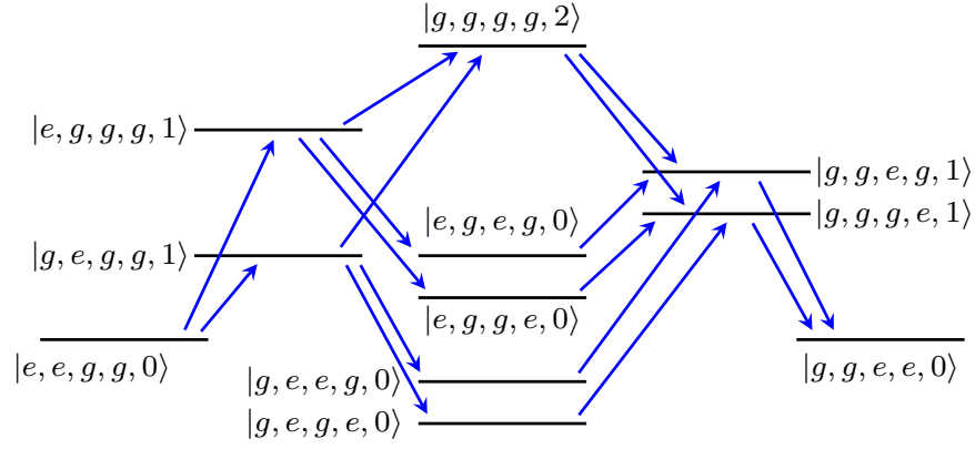
Figure 9. The 8 fourth-order paths connecting the states |e, e, g, g, 0\rangle and |g, g, e, e, 0\rangle using only the TC terms. To set the energy levels, we have used the parameter values \omega_c = 6\omega_2 , \omega_1 = 4\omega_2 , \omega_3 = 3\omega_2 , and \omega_4 = 2\omega_2 .
