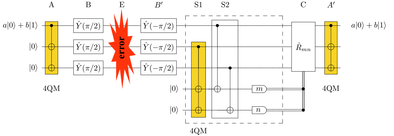
Figure 12. Circuit implementing an ECC correcting a single phase-flip error. If the modules B and B' are omitted, then the circuit corrects a single bit-flip error. The circuit modules include: encoder A , basis rotator B (from the basis \{|0\rangle, |1\rangle\} into \{|+\rangle, |-\rangle\} ) corresponding to the Hadamard gates or rotations \hat{Y}(\pi/2) , dissipative channel or evolution ( E , when the error happens), basis rotator B' (from \{|+\rangle, |-\rangle\} into \{|0\rangle, |1\rangle\} being inverse to B ), error-syndrome detector S (composed of blocks S_1 , S_2 , and detectors with two possible outcomes m, n = 0, 1 ), error corrector ( C , where the single-qubit operation R_{nm} , given by Eq. (D8) is conditioned on the classical information from the detectors), and decoder A' . In our implementation, the blocks A , A' , and S_1 , which are composed of two CNOT gates with two qubits in |0\rangle , can be replaced by type-II four-qubit mixing (4QM), i.e., by spontaneous evolution for the time t = \pi/(2J^{(4)}) of the system governed by the effective interaction Hamiltonian \hat{V}^{(4)} , given in Eq. (D1).
