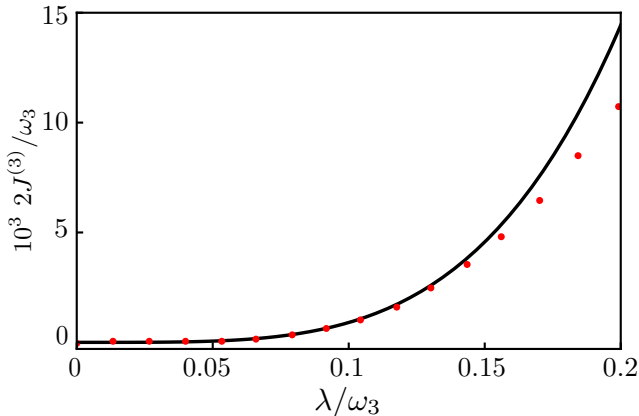
Figure 2. Comparison between the numerically-calculated normalized effective Rabi splitting (points) corresponding to J^{(3)} in Appendix B and the corresponding calculations using the fourth-order perturbation theory (continuous black curve), as a function of the normalized interaction strength \lambda/\omega_3 .
