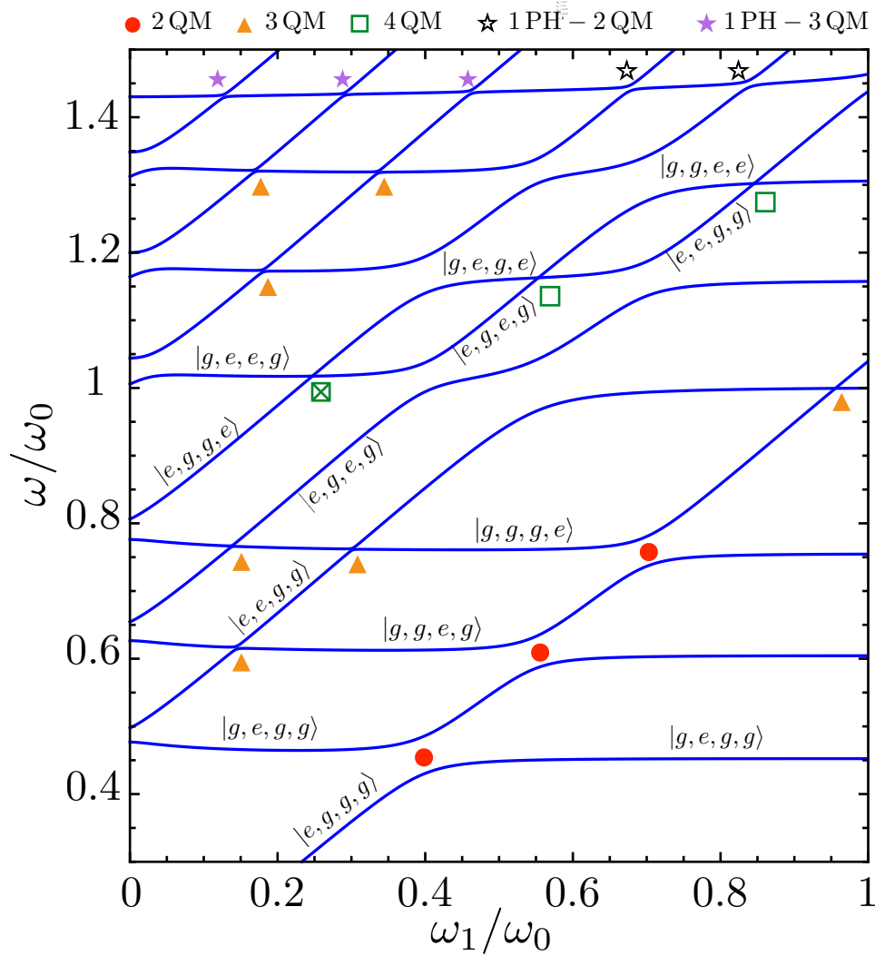
Figure 4. Four nondegenerate qubits dispersively coupled to a cavity mode at higher energy. (a) Lowest energy levels of the system as a function of the frequency of qubit 1, obtained by numerical diagonalization of the Hamiltonian in Eq. (4) with four qubits. The transition frequencies of the other three qubits as well as the resonance frequency of the cavity mode are kept fixed. All the parameters used are provided in the text.
