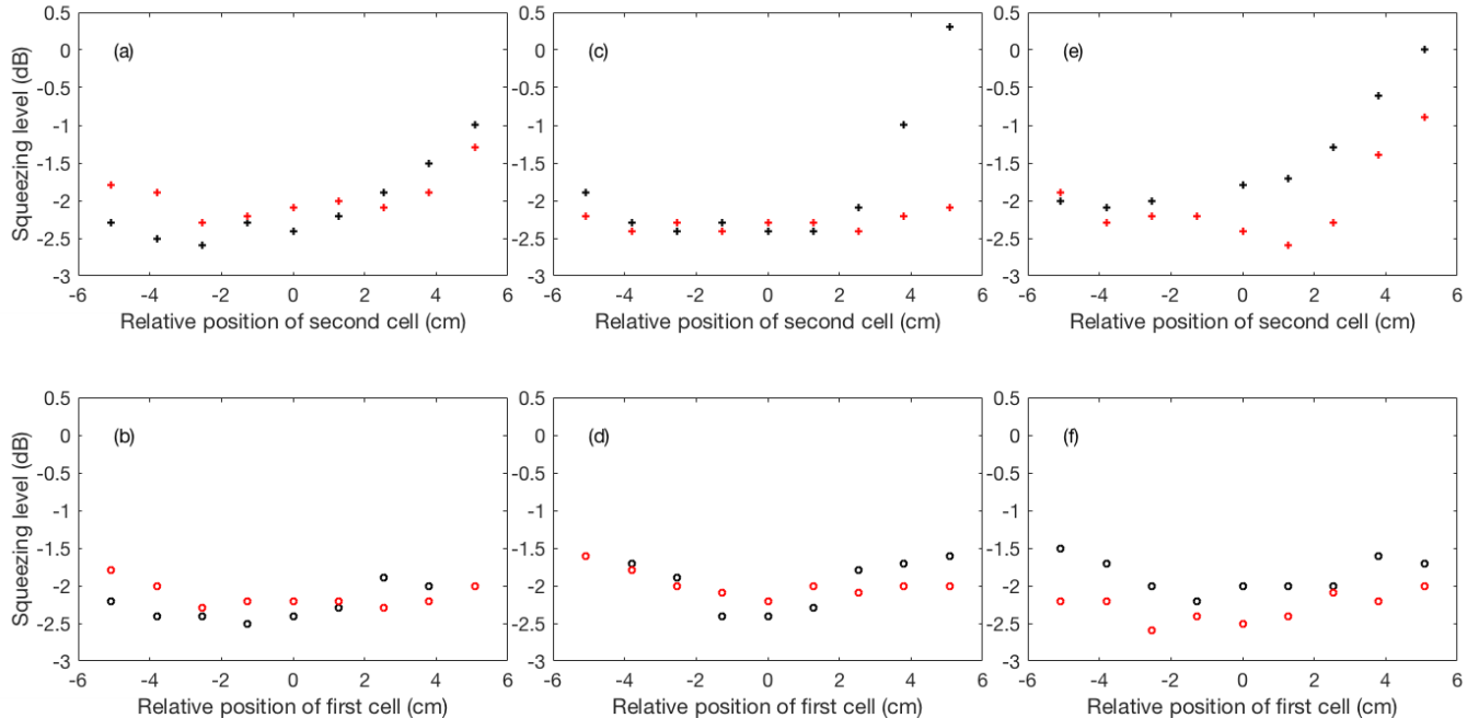
FIG. 8. (Color online) The dependence of squeezing amount on position of the first (circles) and second cell (crosses). Black represent the squeezing is measured when both cells are present. Red (light grey) is when an addition PBS is placed after the first cell and filters the squeezed field generated in the first cell. In figure (a) and (b) the atomic density in both cells is 4.3 \times 10^{11} \text{ cm}^{-3} . In figure (c) and (d) atomic density in the first cell is 4.3 \times 10^{11} \text{ cm}^{-3} and in the second is 9.3 \times 10^{11} \text{ cm}^{-3} . In Figure (e) and (f) the atomic density in both cells is 9.3 \times 10^{11} \text{ cm}^{-3} . In the top row, the position of first cell is -2.5 \text{ cm} . In the bottom row, the positions of second cell are each -2.5 \text{ cm} in (b), 0 \text{ cm} in (d) and 1.3 \text{ cm} in (f), which are the optimal positions found in the top row.
