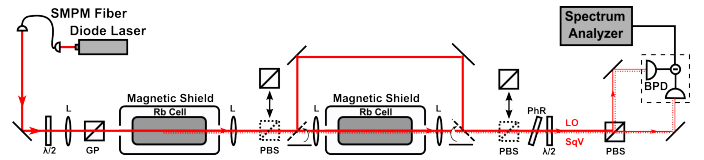
FIG. 6. (Color online) A modified experimental setup with two independent vapor cells. All the abbreviations are the same as in Fig. 1
