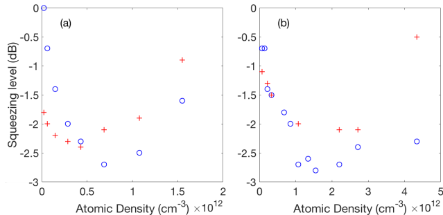
FIG. 7. (Color online) A measurement of squeezing dependence on the second cell density in the two-cell system. In (a) the atom density of the first cell is 9.3 \times 10^{11} \text{ cm}^{-3} and in (b) it is 4.3 \times 10^{11} \text{ cm}^{-3} . Crosses represent the squeezing amount in total and circles correspond to the case when a PBS is inserted after the first cell so that the first-cell-generated squeezing is filtered.
