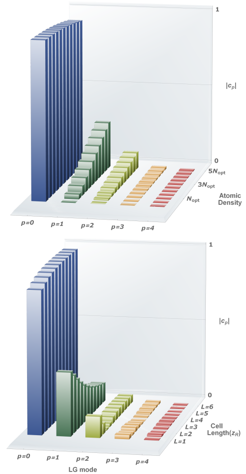
FIG. 5. (Color online) The calculated relative amplitudes of the first few higher-order Laguerre-Gause modes L_p^{\ell=0} as (a) atomic density N gradually increases; or as (b) the length of the atomic medium L (in the units of the Rayleigh radius z_R ) is increased.
