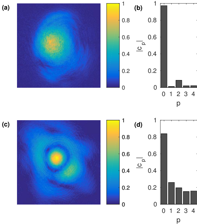
FIG. 4. (Color online) Transverse intensity distribution of the pump field (a) and the absolute values of the calculated deconvolution coefficients |c_p| of the Laguerre-Gause modes L_p^{\ell=0} , defined in Eq.(1) after the cell at room temperature ( T = 26^\circ\text{C} , N = 10^{10}\text{cm}^{-3} ). Small beam contamination due to diffraction give rise to non-zero c_2 coefficient, even if atoms are not present. Corresponding results for the pump beam after the interaction with Rb vapor at high temperature ( T = 91^\circ\text{C} , N = 2.6 \times 10^{12}\text{cm}^{-3} ) are shown in (c) and (d).
