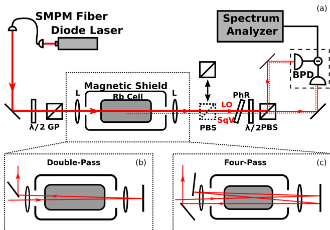
FIG. 1. (Color online) (a) Experimental setup for generation and measurement of PSR quantum noise in a single-pass configuration. SMPM is a single-mode polarization-maintaining fiber, \lambda/2 is half-wave plate, GP is Glan-laser polarizer, PBS is a polarizing beam splitter, PhR is a phase-retarding wave plate, and BPD is a balanced photodetector. Insets (b) and (c) show the modification of the experiment for the double- and quadruple-pass arrangements, correspondingly.
