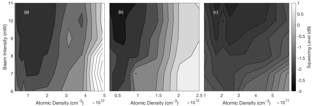
FIG. 2. Experimental optimization of squeezed vacuum in the parameter space of the pump beam power and atomic density for (a) single, (b) double and (c) quadruple-pass configurations. The color represents the value of the minimum quantum noise suppression below the shot noise level (see the scale on the right), with the darkest areas in each plot representing the “island” of optimal conditions for squeezing. Note the difference in horizontal scaling between the three graphs.
