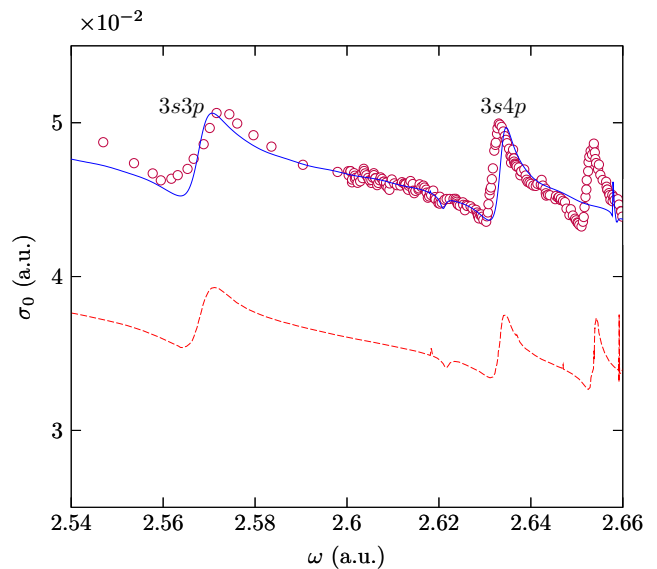
FIG. 2. Photoionization cross section of helium above the N = 2 threshold. Full (blue) line: our results. Dashed, red line: theoretical results of Ref. [28]. Circles: experimental results of Ref. [27] renormalized to our theoretical results.
