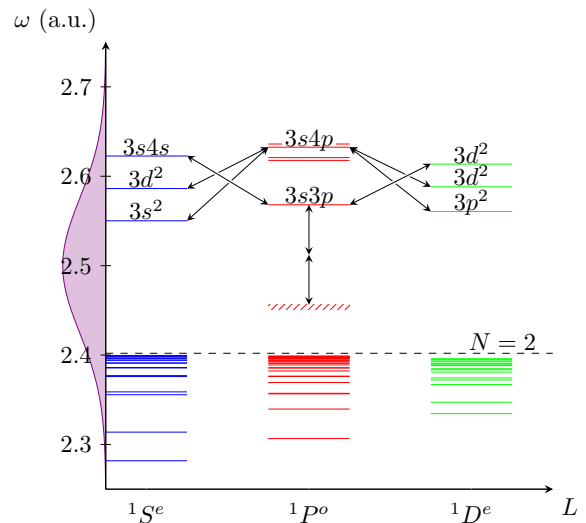
FIG. 1. A diagram of 1S^e , 1P^o , and 1D^e helium energy levels below and above the N = 2 threshold [20–22]. The P continuum between the N = 2 threshold and the 3s3p doubly excited state is illustrated with diagonal stripes. The N = 2 threshold is indicated by a black, dashed line. The frequency distribution of the XUV used to populate the states, shown to the left, is centered at 2.5 a.u. and has a FWHM of 0.18 a.u.. Likely transitions due to the VIS, which has a central frequency of 0.057 a.u., are illustrated using arrows.
