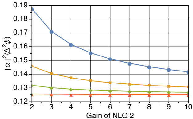
FIG. 11. Sensitivity versus gain of NLO 2 for intensity detection ( \hat{M}_N ) of conventional SU(1,1) interferometer, optimized over \phi . NLO 1 has g = 2 and there is no internal loss. The blue dots, yellow squares, green diamonds, and orange triangles represent external transmissions of \eta_{ae} = \eta_{be} = 0.5, 0.75, 0.9 and 0.99 , respectively.
