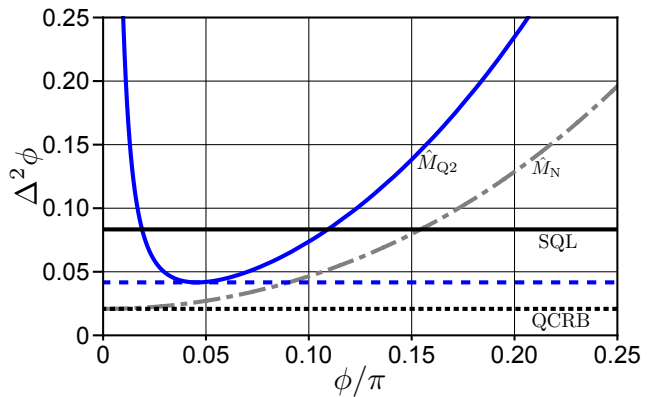
FIG. 6. Sensitivity as a function of operating point for vacuum-seeded schemes with a gain of 4. Sensitivity is shown for several experimental configurations: intensity detection ( \hat{M}_N ) is in gray dash-dot, homodyne detection of truncated and conventional SU(1,1) interferometer ( \hat{M}_{Q2} ) with LOs set at \theta_a = \theta_b = \pi/2 is dark blue, and homodyne detection of truncated and conventional SU(1,1) ( \hat{M}_{Q2} ) optimized over LO phases is blue dashed. The QCRB is the black dotted line and the SQL is the solid black line.
