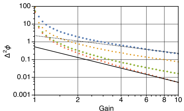
FIG. 9. Sensitivity as a function of gain for homodyne measurement of vacuum seeded truncated or conventional SU(1,1) interferometer ( \hat{M}_{Q2} ) and no external loss. Gain is linear in number of spontaneous photons: \bar{n}_s = 2g - 2 . The blue dots, yellow squares, green diamonds, and orange triangles represent internal transmissions \eta_{a_i} = \eta_{b_i} = 0.5, 0.75, 0.95 and 1, respectively. The black lines are guides for the eye where the dashed has scaling 1/g and the solid has scaling 1/g^2 .
