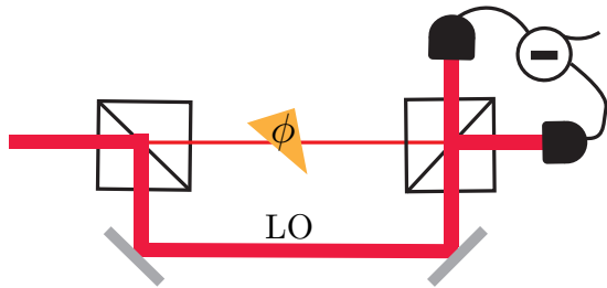
FIG. 3. A phase sensor that can be viewed either as an imbalanced Mach-Zehnder interferometer or as a balanced homodyne detector with a local oscillator (LO) that has a well-defined phase with respect to the weak beam. The weak beam passing through the optical phase shift, \phi , contains \bar{N}_p photons on average.
