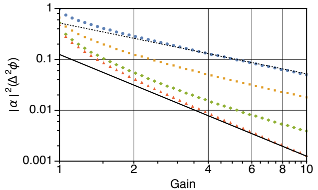
FIG. 7. Sensitivity as a function of gain for homodyne measurement of bright seeded truncated or conventional SU(1,1) interferometer ( \hat{M}_Q ) and no external loss. Gain is linear in number of spontaneous photons: \bar{n}_s = 2g - 2 . The blue dots, yellow squares, green diamonds, and orange triangles represent internal transmissions \eta_{ai} = \eta_{bi} = 0.5, 0.75, 0.95 and 1 , respectively. The black lines are guides for the eye where the dashed has scaling 1/g and the solid has scaling 1/g^2 .
