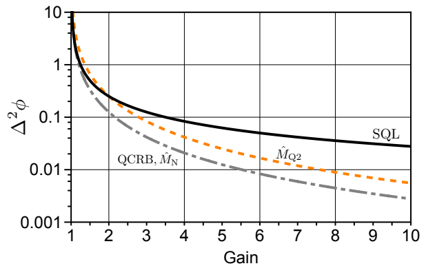
FIG. 8. Sensitivity as a function of gain for vacuum seeded configurations, optimized over \phi and LO phases. Sensitivity is shown for several experimental configurations: homodyne detection of truncated and conventional SU(1,1) interferometer ( \hat{M}_{Q2} ) is in orange dashed, intensity detection ( \hat{M}_N ) is in gray dash-dot. The QCRB coincides with the gray dash-dot curve and the SQL is the solid black curve.
