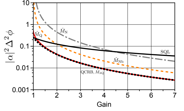
FIG. 5. Sensitivity as a function of gain for bright seeded configurations, optimized over \phi and LO phases. Sensitivity is shown for several experimental configurations: intensity detection ( \hat{M}_N ) is gray dash-dot, intensity detection of mode b_f only ( \hat{M}_{Nb} ) is orange dashed, homodyne detection for truncated and conventional SU(1,1) interferometer ( \hat{M}_Q ) is thick red, and homodyne detection for truncated SU(1,1) interferometer with classical gain correction ( \hat{M}_{\lambda Q} ) is black dotted. The QCRB coincides with black dotted and the SQL is solid black.
