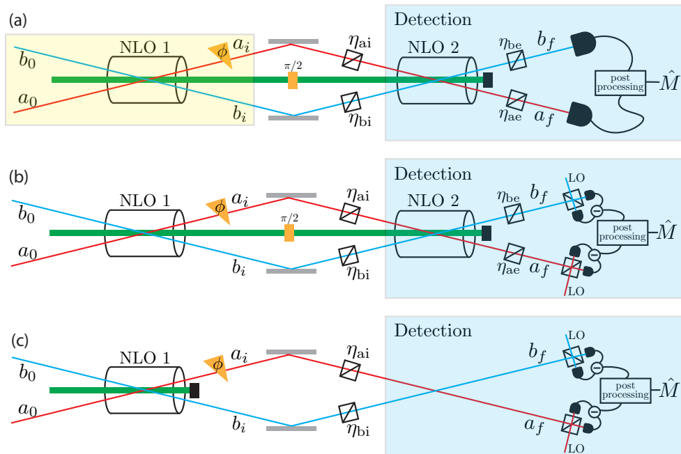
FIG. 2. The three experimental configurations considered in this paper. The thick green line is a strong classical pump beam. (a) The conventional SU(1,1) interferometer. (b) The conventional SU(1,1) with homodyne detection on the output. (c) The truncated SU(1,1) interferometer. LO indicates a local oscillator, and beamsplitters represent loss and are labelled by their transmission \eta .
