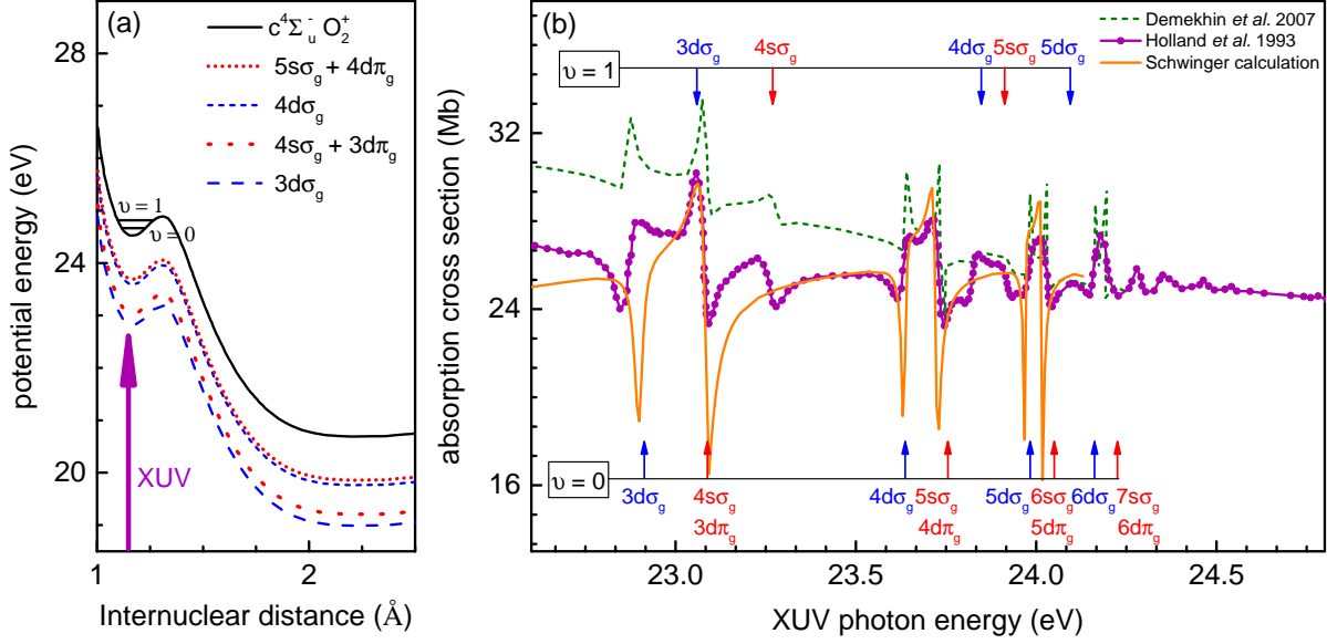
FIG. 1. (Color online) (a) Schematic potential energy diagram of O 2 . Black curve is the excited ionic c-state ( c^4\Sigma_u^- ). Blue dashed and red dotted curves are Rydberg series of neutral superexcited nd and ns states, respectively. Each state supports two vibrational levels. (b) (Purple line) Synchrotron measurement of photoabsorption cross section from [31]. Features associated with various electronic states and their vibrational levels ( \nu=0 at bottom and \nu=1 at top) are labeled. (Green dash line) Theoretical photoabsorption cross section from [32]. (Orange solid curve) Multichannel photoabsorption cross section that we obtained using Schwinger variational calculation.
