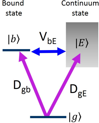
FIG. 6. (Color online) Three level model system showing a ground state |g\rangle , an excited bound state |b\rangle , and a continuum state |E\rangle , along with dipole couplings D_{gb} , D_{gE} , and interaction term V_{bE} .
