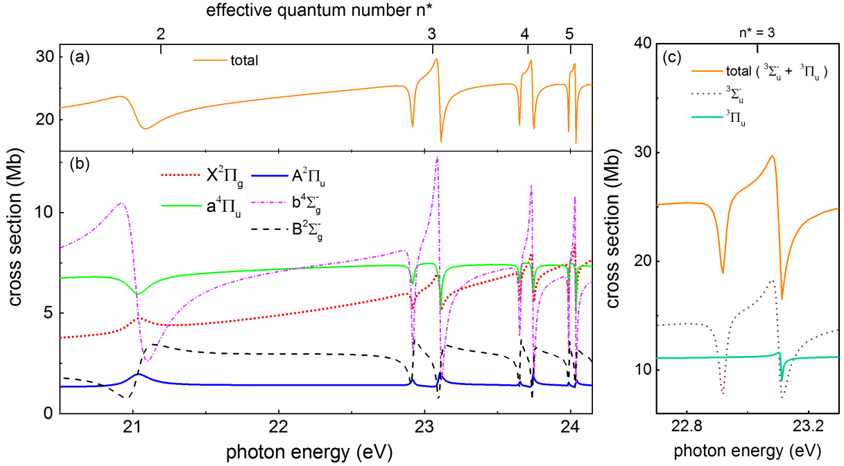
FIG. 4. (Color online) (a) Total cross section as a function of the photon energy and effective quantum number n^* . (b) Various electronic channels contributing the total cross sections and their Fano profiles. (c) Parallel ( ^3\Sigma_u^- ) and perpendicular ( ^3\Pi_u ) polarization contributions to the total XUV photoionization cross section in the vicinity of the pair of features with n^* = 3 in Fig. 1 showing the presence of the 3d\sigma_g (parallel), 4s\sigma_g (parallel), and 3d\pi_g (perpendicular) states.
