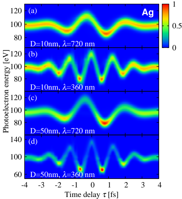
Figure 7. (Color online) Same as Fig. 6 for Ag nanospheres and streaking-field wavelengths of 720 and 360 nm.
