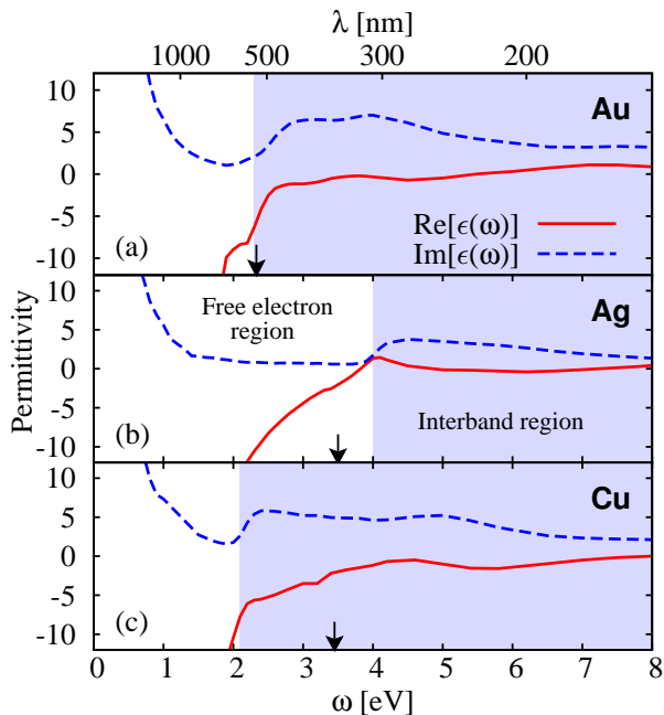
Figure 2. (Color online) Real and imaginary components of the complex permittivity \epsilon(\omega) for Au, Ag, and Cu (adapted from Ref. [51]). The white and shaded areas indicate free-electron and interband-transition regions, respectively. Arrows point to the dipole surface-plasmon frequencies \omega_D of sub-wavelength nanoparticles for each material.
