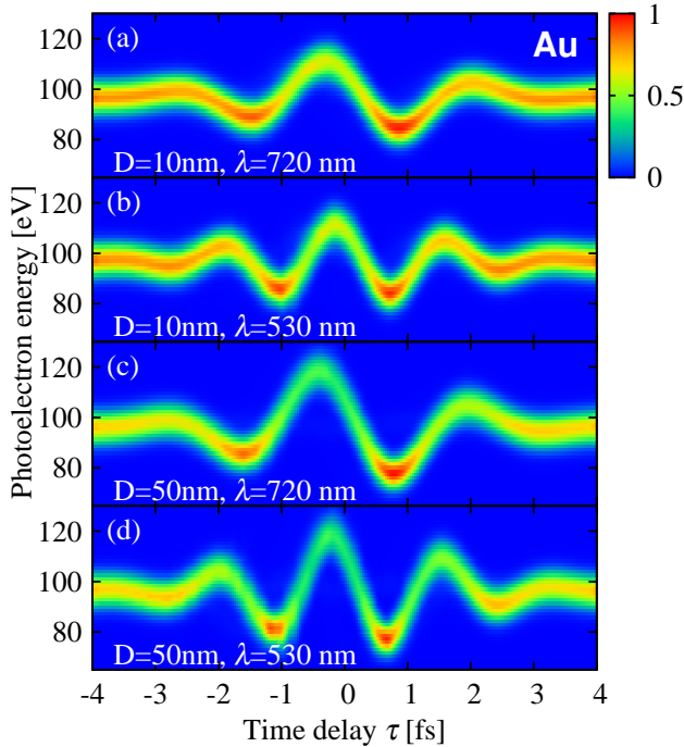
Figure 6. (Color online) Quantum-mechanically calculated streaked XUV photoemission spectra for 10 and 50 nm diameter Au nanospheres and streaking-field wavelengths of 720 and 530 nm. The linear color/gray scale gives the photoemission yield separately normalized to the maximal yields in (a)-(d).
