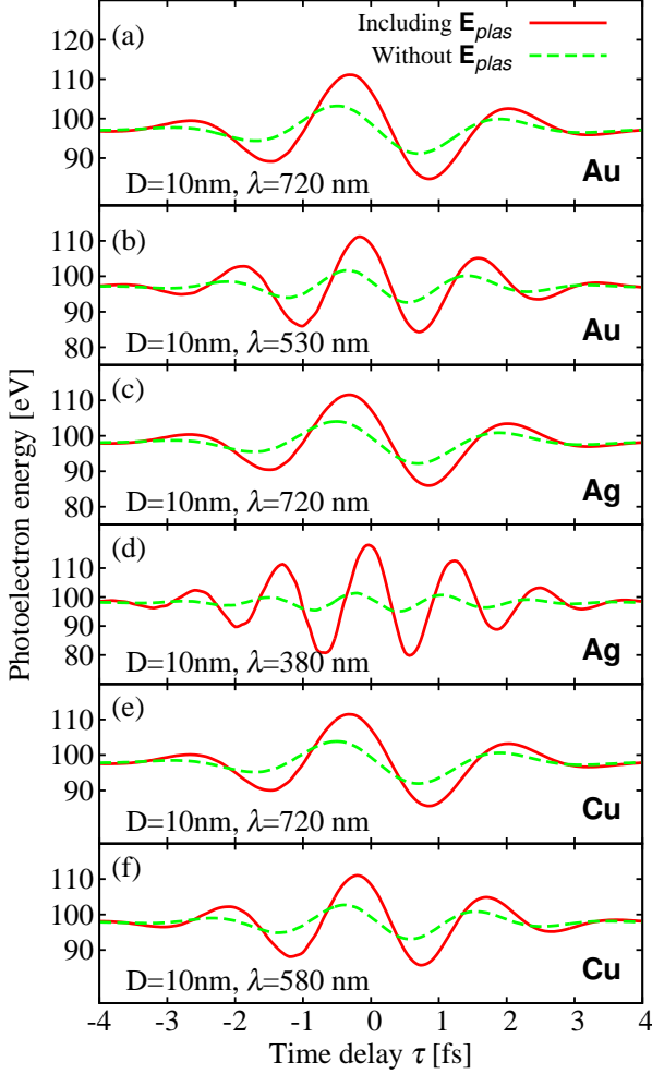
Figure 10. (Color online) Centers-of-energy of streaked photoelectron spectra for 10 nm diameter (a),(b) Au, (c),(d) Ag, and (e),(f) Cu nanospheres, including (red solid line) and excluding (green dashed line) the induced plasmonic field \mathbf{E}_{plas} in Eq. (2).
