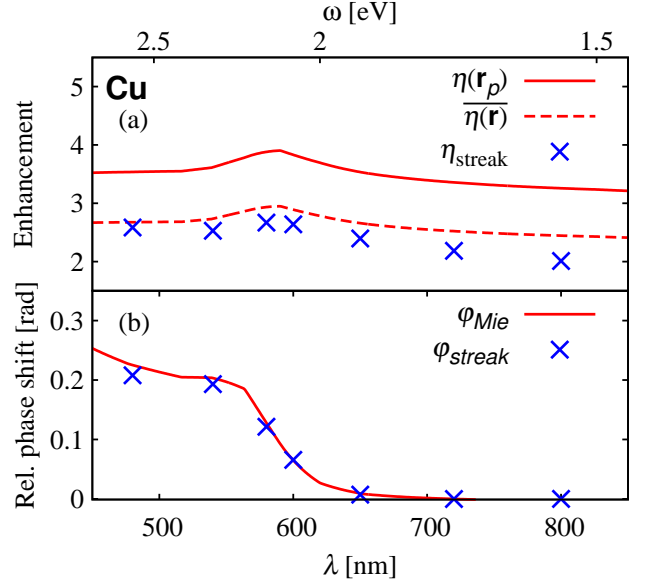
Figure 13. (Color online) Same as Fig. 11 for Cu nanospheres.
