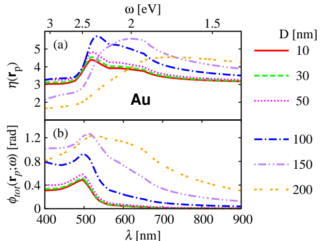
Figure 3. (Color online) (a) Plasmonic field enhancement \eta(\mathbf{r}_p) and (b) phase shift \phi_{tot}(\mathbf{r}_p; \omega) at the electric-field poles \mathbf{r}_p on Au nanospheres with diameters D as a function of the incident plane wave's wavelength \lambda .
