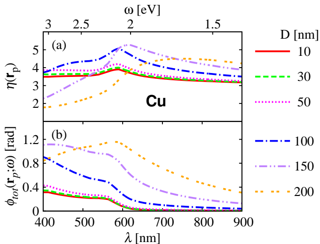
Figure 5. (Color online) Same as Fig. 3 for Cu nanospheres.
