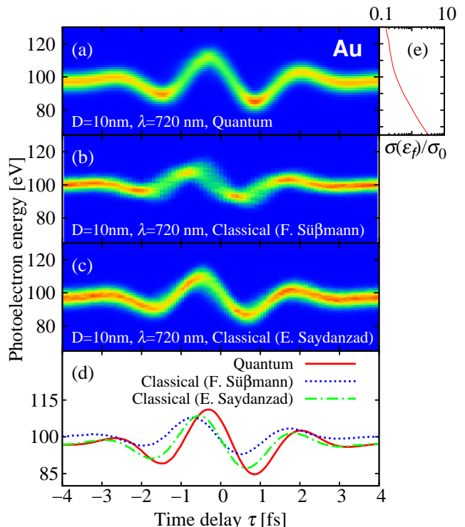
Figure 9. (Color online) Calculated streaked XUV photoemission spectra for 10 nm diameter Au nanospheres and streaking-field wavelengths of 720 nm according to (a) our quantum-mechanical model, (b) the classical model of Süßmann and Kling (adapted from Ref. [19]), and (c) the classical model of Saydanzad et al. (adapted from Ref. [48]). The linear color/gray scale gives the photoemission yield normalized to the maximal yield for each plot. (d) Centers of energy of the spectra in (a)-(c). (e) XUV-photoionization cross section \sigma(\varepsilon_f) , normalized at \sigma_0 = \sigma(80 \text{ eV}) .
