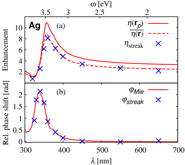
Figure 12. (Color online) Same as Fig. 11 for Ag nanospheres.
