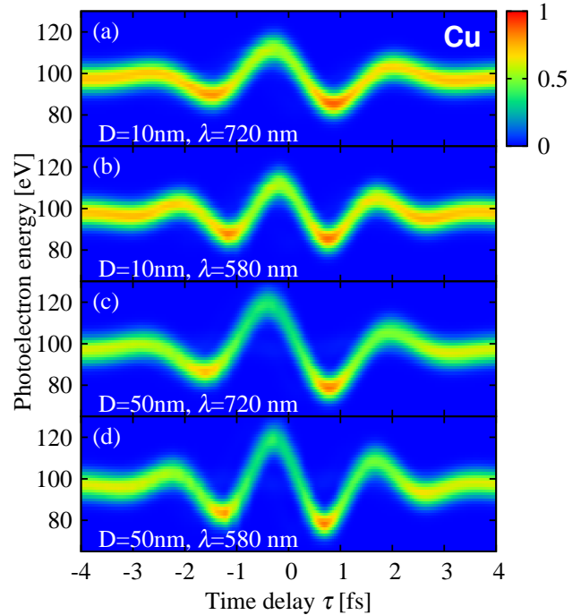
Figure 8. (Color online) Same as Fig. 6 for Cu nanospheres and streaking-field wavelengths of 720 and 580 nm.
