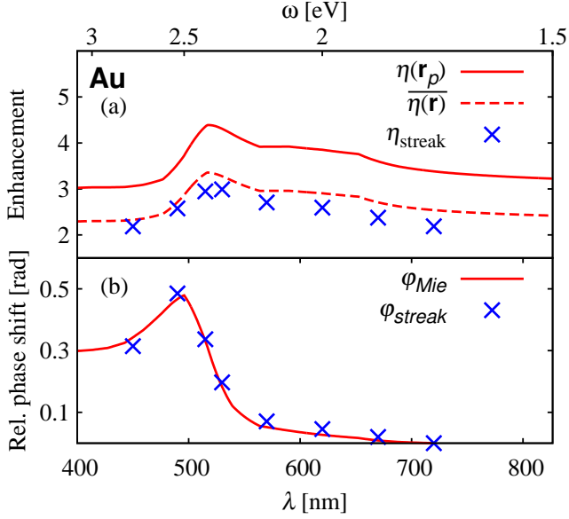
Figure 11. (Color online) Plasmonic amplitude-enhancement and phase-shift retrieval for 10 nm diameter Au nanospheres from streaked photoemission spectra. (a) Plasmonic field enhancement \eta defined in Eq. (4), as predicted by classical electrodynamics: \eta(\mathbf{r}_p) (solid red line) gives values at the nanosphere poles; \overline{\eta(\mathbf{r})} (dashed red line) gives the field-strength enhancement, dipole-averaged over the nanosphere surface. Blue markers indicate the retrieved field-strength enhancement \eta_{streak}(\lambda) defined in Eq. (25). (b) Plasmonic phase shift \varphi_{Mie}(\lambda) according to Eq. (27) as predicted by classical electrodynamics at the nanosphere poles (solid red line). Blue markers show the retrieved plasmonic phase-shift difference \varphi_{streak}(\lambda) defined in Eq. (26) as a function of the streaking-pulse wavelength.
