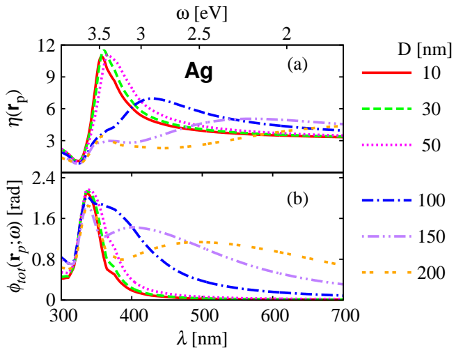
Figure 4. (Color online) Same as Fig. 3 for Ag nanospheres.
