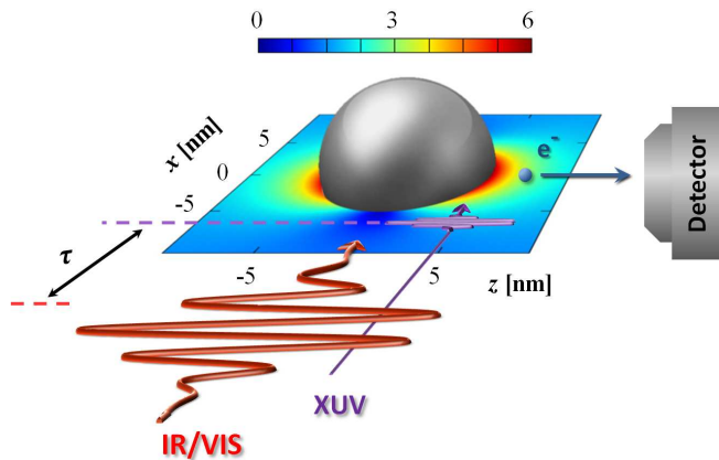
Figure 1. (Color online) Schematic of attosecond streaking from nanoparticles. A single ultrashort attosecond XUV pulse emits electrons into the field of a delayed IR or visible streaking laser pulse. The linear color/gray scale represents the maximal local electric-field-strength enhancement \eta(\mathbf{r}) [cf., Eq. 25] in the x-z plane for the example of 10 nm diameter Ag nanospheres exposed to 720 nm incident IR pulses with peak intensity 10^{12} \text{W/cm}^2 .
