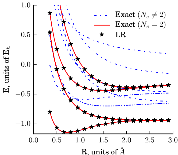
FIG. 5. The energy of different electronic states as a function of internuclear separation for the H_2 molecule in a minimal STO-6G basis, encoded into qubits by the Jordan-Wigner mapping. Both the entire exact spectrum is shown with dot-dashed lines, as well as the exact spectrum restricted to a neutral molecule ( N_e = 2 ). The blue dotted lines depict only ionic N_e \neq 2 states that are not the focus in this study. This depicts the volume of states in a naïve mapping that must be avoided to capture physical solutions. In this case the linear response (LR) approximation from an exact reference is sufficient to capture exactly the excited states with the correct number symmetry, as the excitation operators conserve the number from the exact reference state.
