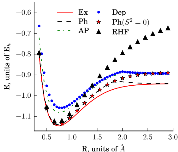
FIG. 3. The exact solution of the VCS model for the ground state of \text{H}_2 is shown for a number of different quantum channels including amplitude and phase damping (AP), dephasing only (Ph), and depolarizing noise (Dep). These results are shown along side both the exact (Ex) ground state, an anti-symmetric product state approximation (RHF), and the best solution of a dephasing channel constrained to have correct spin ( S^2 = 0 ). It is seen that dephasing noise is sufficient to destroy the entanglement required to describe the dissociated limit, in that the solution without symmetry constraints obtains an accurate energy, but only by breaking spin symmetry in an unphysical way, as evidenced by the difference when compared to the optimal dephasing solution under symmetry constraints. Other types of noise raise the energy of the whole curve due to number symmetry breaking. The kink in the curves without symmetry enforcement results from a spin symmetry breaking in the variationally optimal solution in the presence of decohering noise.
