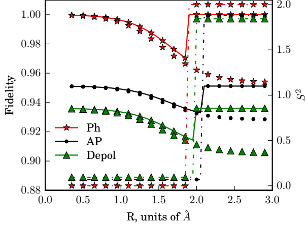
FIG. 2. The fidelity of the initial and final states as a function of internuclear distance ( R ) in H_2 after being passed through three different quantum channels (Ph–Dephasing, AP–Amplitude and Phasing Damping, Depol–Depolarizing) improves under variation in the presence of the channel (VCS solution, solid lines with markers) when compared to the exact less ground state as input (ground state of untransformed Hamiltonian, markers only). The dotted lines represent the expected value of S^2 for the same color line under the ideal solution with a channel (solid line). From this, one can see the kinks correspond precisely to discontinuous changes in the spin-symmetry. The discontinuities are indicators of locating a decoherence resistant state that is symmetry broken with respect to the exact, ideal solution. The channels are characterized by an experiment time T_p relative to coherence time parameters T_1 = T_2 = T_{\text{depol}} time such that T_p/T_1 = 0.05 .
