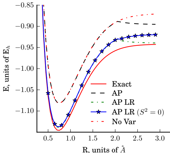
FIG. 6. In examining the energy as a function of separation for the ground state of H_2 under a particular amplitude and phase damping channel (AP), one sees that in the linear response subspace (AP LR), the solution quality is increased with respect to the optimal solution of the quantum channel model (AP). The qualitative kink in the approximate solution can be repaired by enforcing the correct spin symmetry ( S^2 = 0 ). This also demonstrates the effect on the energy between variational minimization with the channel (AP) and without (No Var).
