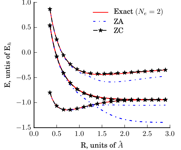
FIG. 7. The ground and first two excited states of H_2 are plotted as a function of internuclear separation using both the Zero Approximation (ZA) and the Zero Approximation under the commutator construction (ZC). Both methods require only the original measurements used for the ground state to approximate the excited states, and we see here that ZC achieves an extremely high accuracy, while ZA is qualitatively correct in some cases but produces sub-variational solutions in others.
