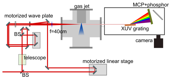
FIG. 1. Experimental setup, see text for details.
