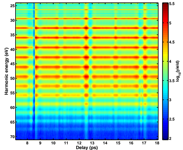
FIG. 2. (color online) Raw spectrum in logarithmic scale of harmonics generated from N_2 as a function of the delay between the first pump and the probe and of the harmonic energy. The second pump is present at a delay of 8.36 ps respect to the first pump. Strong features at times of alignment for all harmonics are visible. However, further features at times of anti-alignment before the full alignment (delay \approx 16 ps) become more visible as the harmonic energy increases.
