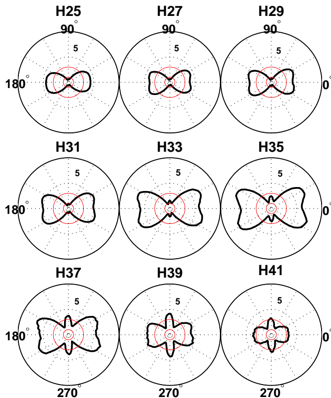
FIG. 4. (color online) Measured harmonic yield of individual harmonics as a function of angle between pump and probe at the full revival of 17.04 ps ( \langle \cos^2 \theta \rangle \approx 0.67 ). The experimental data was generated under the same conditions as presented in Fig. 3. Each harmonic yield is normalized to its corresponding isotropic value for an unaligned molecular ensemble. The red circles represent radial values of 1 and 3 units.
