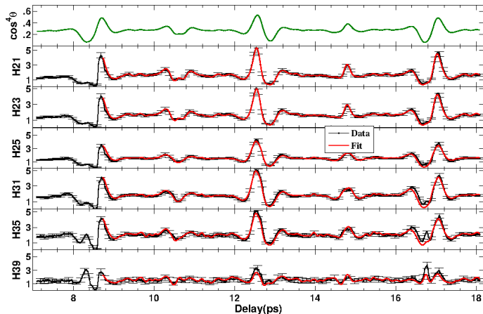
FIG. 3. (color online) Yield of harmonics H21, H23, H25, H31, H35 and H39 from N_2 , normalized to the respective isotropic values, as a function of the delay between the first pump and the probe in 20 fs steps (black). In all cases the second pump is at a delay of 8.36 ps respect to the first pump. Harmonics 21 and 23 show the same behavior as our calculations of \langle \cos^4 \theta \rangle , depicted in green (top panel). Harmonics 31 and higher, show a peak at the anti-alignment dip (16.78 ps) in front of the full revival (17.04 ps). In particular, for harmonic 39 this peak becomes brighter than the full-revival peak. There are other smaller features in the delay scan of harmonic 39 that show a clear departure from the expected \langle \cos^4 \theta \rangle . Also shown is the fitting using the procedure outlined in [18] (red). The error bars are the standard deviation from 18 averages, resulting in a standard error of the mean that is \sqrt{18} smaller than the standard deviation.
