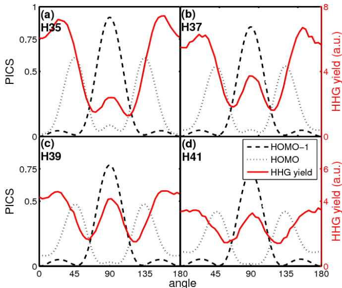
FIG. 5. (color online) A comparison between the experimental angle scans (solid red line) at the full revival of 17.04 ps and theoretical calculations of the photoionization cross sections of HOMO (dotted line) and HOMO-1 (dashed line) from Ref. [43]. The cross section is normalized to 1, while the experimental data is normalized to the isotropic harmonic yield. The dotted line of the PICS of HOMO shows a strong minimum at 0^\circ and 180^\circ that is due to the Cooper minimum in nitrogen. Without better alignment, this feature cannot be fully resolved. However, the feature at 90^\circ can only be explained by the strong contribution from HOMO-1 to HHG (dashed line). As we then look at the experimental data as a function of harmonic order, the yield at 90^\circ gets stronger as we increase the harmonic order, compared to 0^\circ and 180^\circ .
