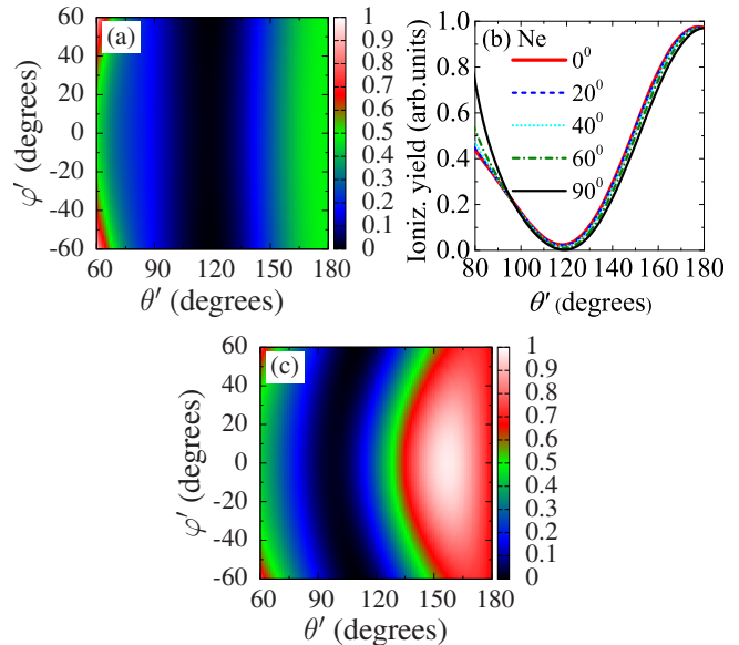
FIG. 4. (Color online) (a) Yields extracted with a “proper” choice of return direction (or z' -axis) with k_s = 1.22 a.u. for Ne(2p - ) as a function of scattering angles \{\theta', \varphi'\} . (b) A few cuts of (a) along different \varphi' , showing the independence of the “retrieved” DCS on \varphi' when the proper return direction is used. (c) Same as (a) but with a z' -axis rotated by -20^\circ in xy plane from the proper return direction.
