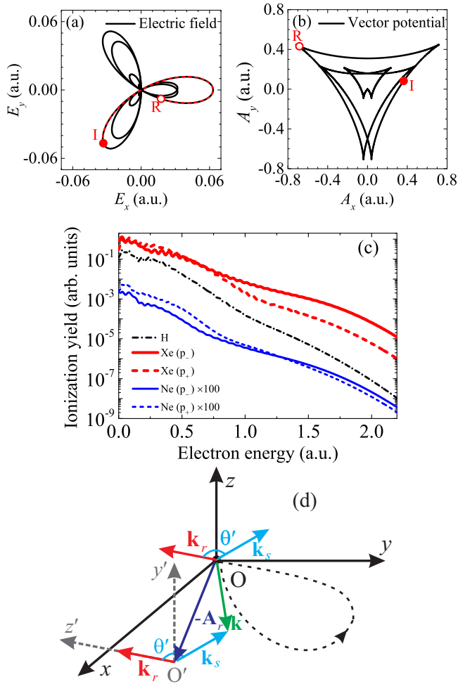
FIG. 1. (Color online) (a) The electric field (Lissajous curve) of the laser used in the calculations and (b) its vector potential. An ionization (and return) event is marked as I (and R), which gives the return energy near 2.25U_p . (c) Electron energy spectra from H, Ne, and Xe. Note that the yields for Ne have been multiplied by a factor of 100. (d) Schematic of the kinematics and the notations used in the text. The laser polarizations are in xy plane. The electron trajectory is shown as dashed line in xy plane, with the return momentum \mathbf{k}_r . z' and y' axes of new frame F' are also shown. See text for details.
