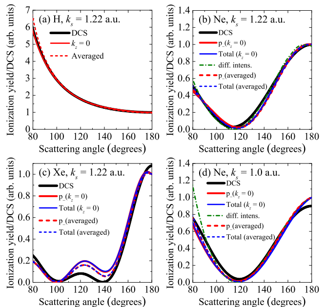
FIG. 3. (Color online) (a), (b), and (c): Extracted yields along the white arcs shown in Fig. 2 with a “radius” k_s = 1.22 a.u., for H, Ne, and Xe, respectively. Different extraction procedures were used (see the labels). The sum of yields from p_- and p_+ is labeled as “total”. Results extracted from Fig. 2(d) are labeled as “diff. intens.”. The averaged results from Fig. 2(d) are labeled as “averaged”. (d) Same as (b) but for k_s = 1.0 a.u. Note that the blue curves are almost on top of the red curves in all cases. The theoretical laser-free DCS is shown as a thick solid black line. The photoelectron yields have been normalized to that of the DCS near 180^\circ .
