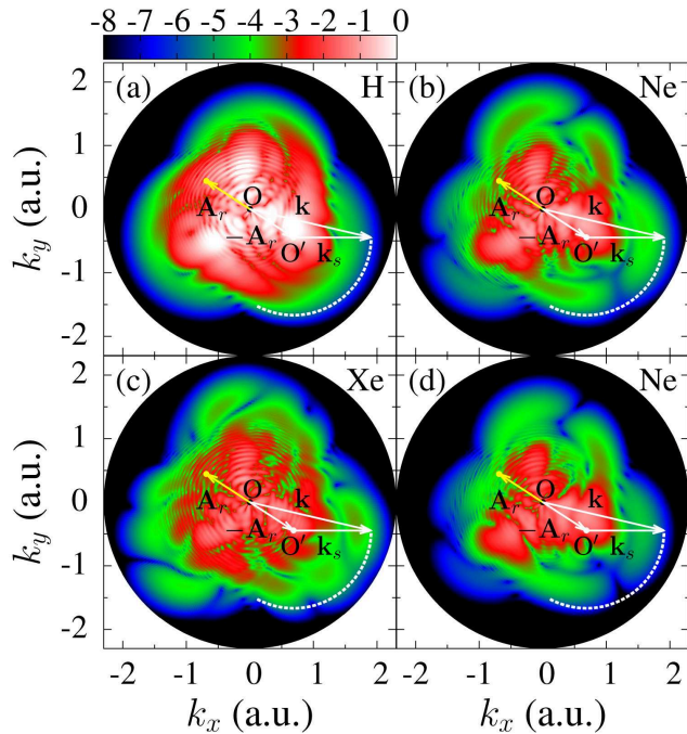
FIG. 2. (Color online) 2D momentum spectra in xy plane from H, Ne( 2p_- ), and Xe( 5p_- ) in (a), (b), and (c), respectively. The dashed white circular arcs denote the region where electron yields are extracted in Fig. 3, for k_s = 1.22 a.u. (d): Same as (b) but with different intensity and ellipticity for 400-nm laser pulse. The peak in each panel has been normalized to 1. See text for details.
