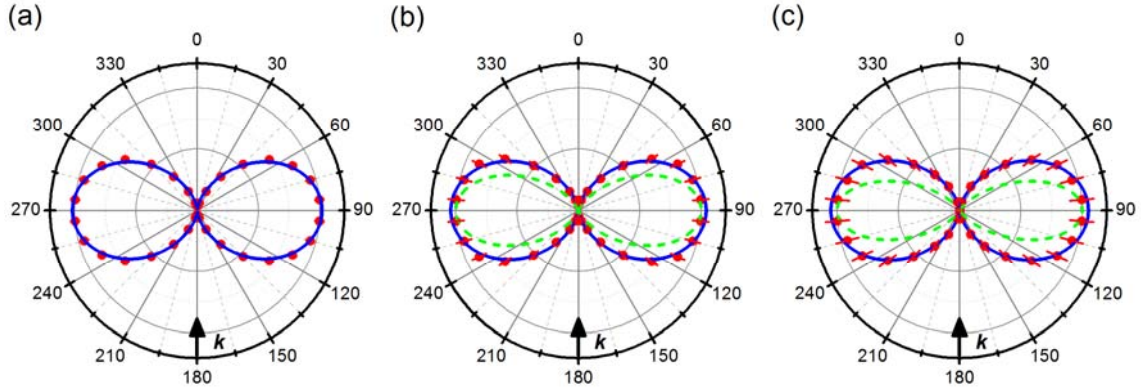
Fig. 4. Angular distributions of photoelectrons measured for the (a) first, (b) second and (c) third harmonics from the helical undulator. The peak photon energies of the undulator radiation are 31, 32 and 32 eV for the first, second and third harmonics, respectively. The solid blue curve in (a) represents a fit assuming electric dipole transitions. The dotted green curves in (b) and (c) show the angular dependence of the photoelectrons expected for non-dipole transitions induced by the OAM carried by the XUV vortex. The solid blue curves in (b) and (c) represent fit results assuming both electric dipole and non-dipole transitions.
