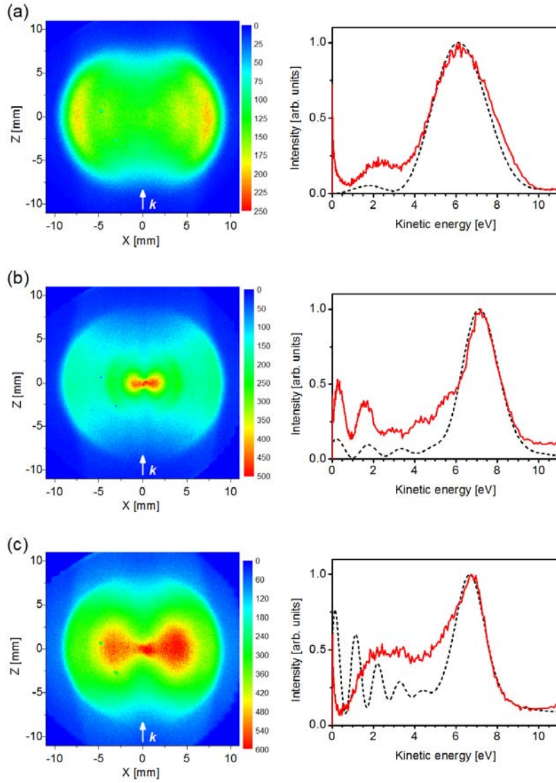
Fig. 3. Images and kinetic energy distributions of photoelectrons measured for the (a) first, (b) second and (c) third harmonics from the helical undulator. The peak photon energies of the undulator radiation are 31, 32 and 32 eV for the first, second and third harmonics, respectively. In the kinetic energy distributions, measurement and calculation results are plotted by solid red and dotted black curves, respectively.
