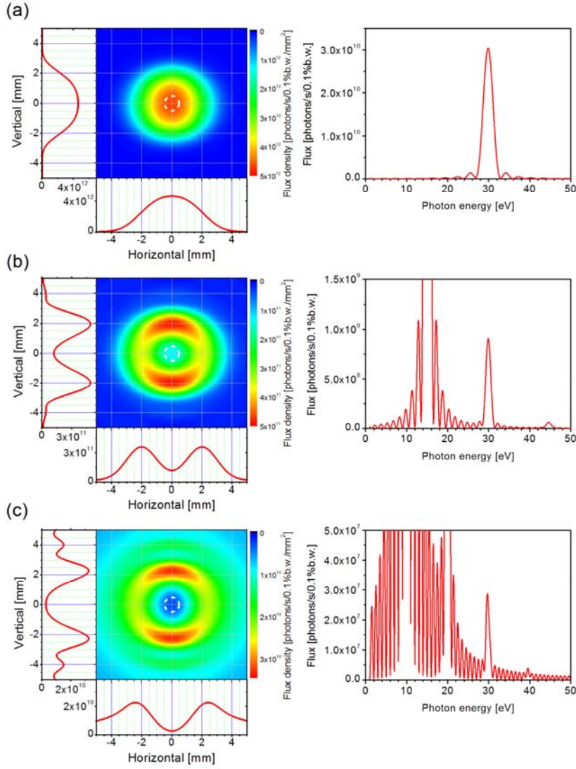
Fig. 2. Simulation of the undulator radiation at the interaction point for the (a) first, (b) second and (c) third harmonics. Left: two-dimensional flux density plots in units of photons per second per 0.1% bandwidth (b.w.) per \text{mm}^2 for 30 eV photons. The intensity profiles along the horizontal and vertical center axes of the two-dimensional plots are attached. The first harmonic corresponds to a plane wave. The second and third harmonics correspond to XUV vortices carrying OAM of l\hbar per photon with l=1 and 2 , respectively. For the harmonic radiation, the phase of the electromagnetic field changes according to the azimuthal angle around a zero-intensity minimum corresponding to the phase singularity on the propagation axis. In the present study, the zero-intensity minimum associated with the phase singularity is blurred due to the finite emittance of the electron beam. In the measurements, undulator radiation is collimated by a 1 mm diameter pinhole. The cut out areas are indicated by dotted circles. Right: partial photon flux obtained for the undulator radiation passing through the 1 mm diameter pinhole.
