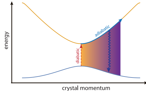
FIG. 8. (Color online) A schematic plot of the momentum space three-step picture for harmonic generation in solids. In the first step, the valence electron tunnels through the band gap. In the second step, the electron wave function evolves adiabatically in the valence and conduction bands. In the final step, the coherence between the valence and conduction band states leads to emission of radiation with energies corresponding to the instantaneous energy difference between the dressed valence and conduction bands.
