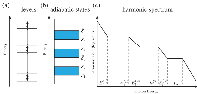
FIG. 5. (Color online) (a) A schematic plot of a multi-level system where levels are coupled in pairs. (b) The energies of the adiabatic states form allowed regions indicated by the blue area. (c) Schematic plot of the multi-plateau structure from this multi-level system. The beginning and end of each plateau are determined by the bounds of the allowed energy regions, as in Eqs. (17) and (19).
