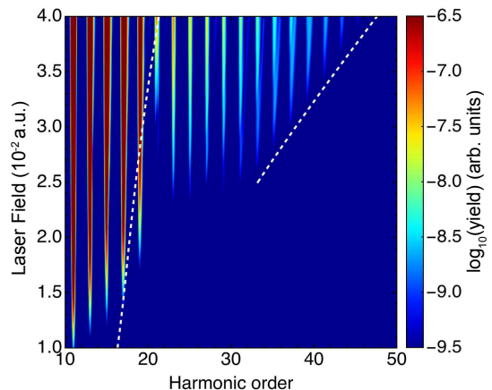
FIG. 6. (Color online) Intensity dependent harmonic spectra for the four-level model for solid argon. The dashed lines indicate the cutoff prediction from Eq. (17) and Eq. (19).
