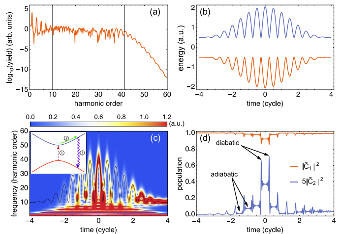
FIG. 1. (Color online) (a) Harmonic spectrum for a two-level system, with parameters \omega_0 = 1 a.u., \Omega_0 = 2 a.u. and \omega = 0.1 a.u.. (b) Adiabatic state energies as a function of time. Avoided crossings are formed at the zeroes of the vector potential. (c) Wavelet transform of the time-dependent current, corresponding to the emission time of the harmonics. The thin black line indicates the energy difference between the adiabatic states in (b). The inset shows the three-step picture for the HHG process near an avoided crossing (see text). (d) Population on the two adiabatic eigenstates.
