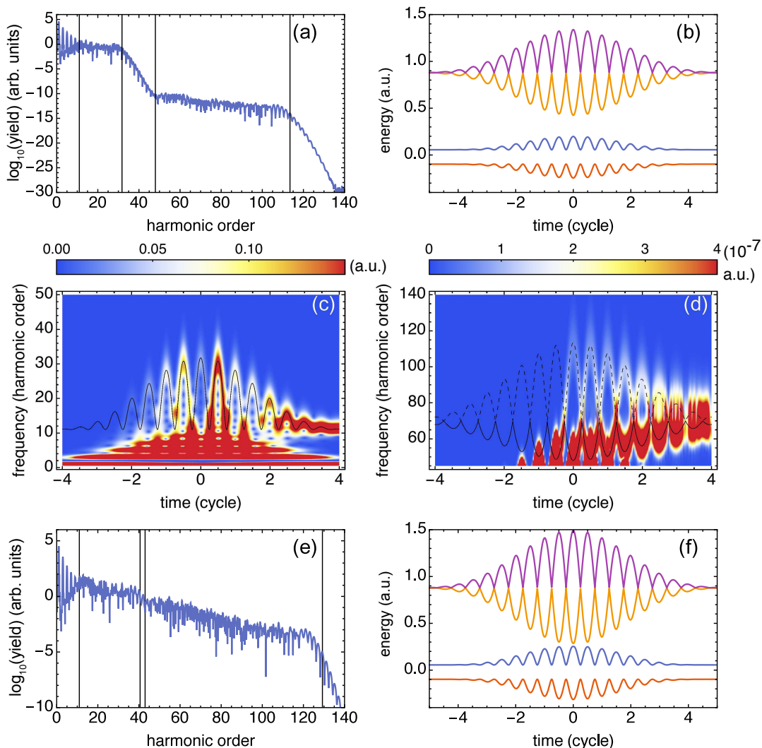
FIG. 3. (Color online) (a) HHG spectrum from a four-level system, with the field strength E_0 = 4.1 \times 10^{-3} a.u.. The harmonic spectrum has two plateaus. The solid lines indicate the predictions from Eq. (17-19) for the lowest and cutoff energies of the two plateaus. (b) The energy of the adiabatic states as a function of time. (c) The wavelet transform of time-dependent current in the energy range of the first plateau. The solid line overlaid on top is the energy difference between the first and the second adiabatic states. (d) The same as (c) but in the range of the second plateau. The solid line indicates the energy difference between the first and third adiabatic states, whereas the dashed line indicates the energy difference between the first and fourth adiabatic states. (e,f) The same as (a,b) but with a field strength E_0 = 5.5 \times 10^{-3} a.u.. At this field strength, the second plateau merges onto the first plateau.
