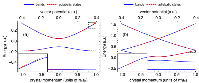
FIG. 7. (Color online) Comparison of the band structure (blue solid lines, bottom axis) and the energy of the adiabatic states vs vector potential (red dashed lines, top axis) for (a) a three-level and (b) a five-level system. The insets in both (a) and (b) show a zoom-in of the region near the edge of the third band, indicated by boxes.
