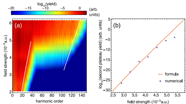
FIG. 4. (Color online) (a) Harmonic spectrum for a four-level system as a function of the field strength. The cutoffs predicted from Eq. (17) and Eq. (19) are indicated with white lines (b) The intensity of the second plateau (blue dots) agrees very well with the prediction from Eq. (24) (red solid line).
