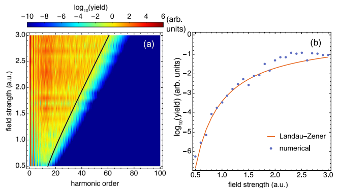
FIG. 2. (Color online) (a) Evolution of the harmonic spectrum as a function of the peak field strength. The solid line indicates the prediction for the cutoff from Eq. (14). As the Rabi frequency exceeds the two-level energy, the cutoff is approximately linear with the field strength. (b) The strength of the harmonic plateau (blue dots) agrees with the prediction of Landau-Zener tunneling (red solid line) very well.
