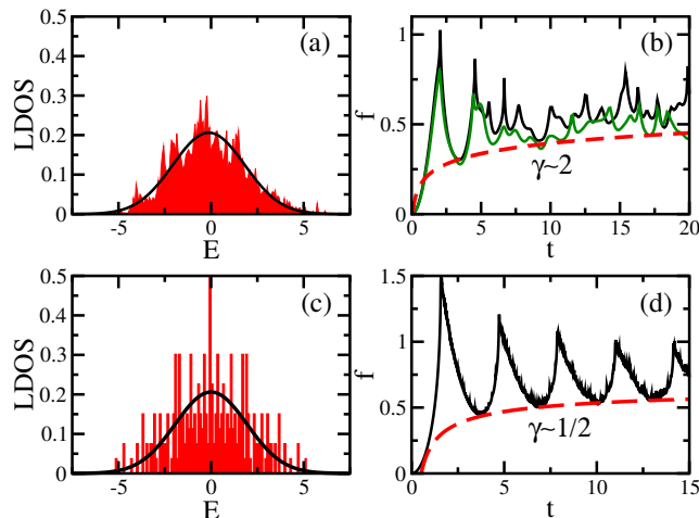
FIG. 3: LDOS (a,c) and f(t) (b,d) for the Néel state under the chaotic open H(2) with h=0 , \Delta=1/2 , \lambda=1 (a,b) and under the closed XX H(c,d) . In (a,c): numerical LDOS (shaded area) and Gaussian envelope (solid line). In (b): numerical results for L=22 (light), L=24 (dark), and const-L^{-1}\ln t^{-2} (dashed). In (d): L=400 (solid) and f_{XX}^{\text{Néel}}(t) (dashed).
