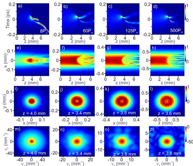
FIG. 4. Subcycle pulse generation by self-compression of laser pulses with \lambda_0 = 3.9 \mu\text{m} and the initial pulse width \tau_0 = 250 fs in an anomalously dispersive nonlinear medium: (a – d) spatiotemporal evolution, (e – h) beam dynamics, (i – l) transverse beam profiles and (m – p) the angular spectra at the point of maximum pulse compression. The input peak power of the laser pulse and beam diameter are P_0 = 8P_{cr} , w_0 = 0.17 mm (a, e, i, m), 60P_{cr} , w_0 = 0.35 mm (b, f, j, n), 125P_{cr} , w_0 = 0.5 mm (c, g, k, o), and 500P_{cr} , w_0 = 1.0 mm (d, h, l, p).
