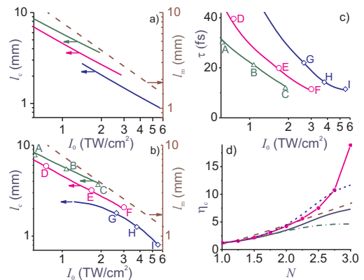
FIG. 1. (a, b) The MI buildup length l_m (dashed line) and the optimal pulse compression length l_c (solid lines) calculated using the NSE (a) and the 1D GNSE (b) as functions of the field intensity. (c) The pulse width \tau_c at the point of maximum compression as a function of the field intensity calculated with the use of the 1D GNSE. The input pulse width is \tau_0 = 80 fs (blue), 150 fs (red), and 250 fs (green). Results of (3 + 1) -dimensional simulations are shown as circles, triangles, and diamonds. (d) The pulse compression ratio \eta = \tau_c/\tau_0 calculated as a function of the soliton number N for \tau_0 = 80 fs using the NSE (dashed line) and the full 1D GNSE (solid line), 1D GNSE without ionization terms (dash-dotted line), 1D GNSE without HOKE terms (dotted line), and 1D GNSE with both ionization and HOKE terms disabled (filled circles connected with a solid line).
