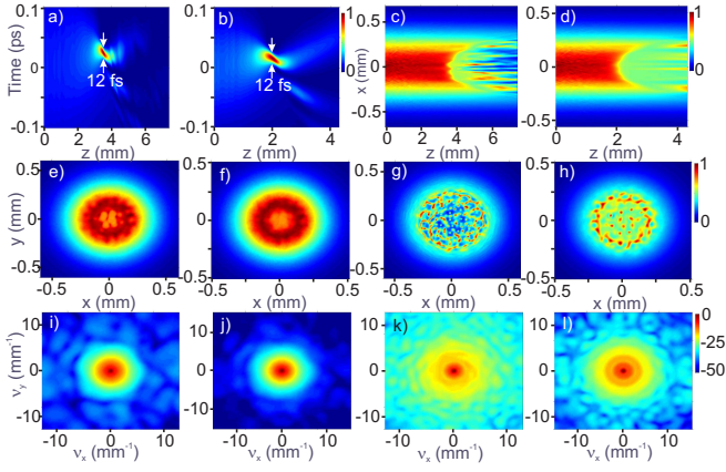
FIG. 2. Self-compression of laser pulses with the central wavelength \lambda_0 = 3.9 \mu\text{m} and the input peak power P_0 = 250P_{cr} in the regimes represented by points C and F in Figs. 1b and 1c: (a, b) spatiotemporal evolution, (c, d) beam dynamics, (e – h) transverse beam profiles and (i – l) the angular spectra at the point of maximum pulse compression, z = 3.7 \text{ mm} (e, i) and 2.1 \text{ mm} (f, j), and in the far field at z = 7.4 \text{ mm} (g, k) and 4.2 \text{ mm} (h, l). The input pulse width and beam diameter are \tau_0 = 80 \text{ fs} , w_0 = 0.4 \text{ mm} (a, c, e, g, i, k) and \tau_0 = 150 \text{ fs} , w_0 = 0.6 \text{ mm} (b, d, f, h, j, l).
