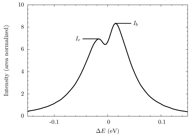
FIG. 1. The double-peaked H \beta line shape. The asymmetry of the core is defined as the fractional difference of the intensity of the blue peak and red peak, (I_b - I_r)/I_b , where the subscripts b and r denote the blue ( \Delta E > 0 ) and red peak ( \Delta E < 0 ), respectively.
