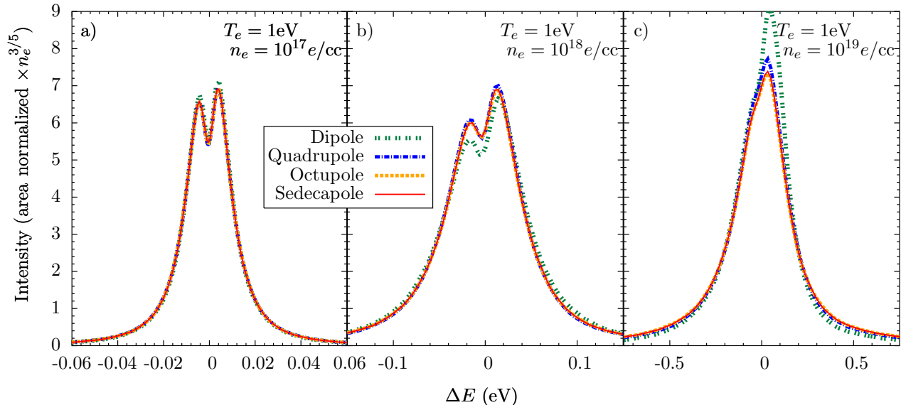
FIG. 3. Area-normalized H\beta profiles at various levels of approximation over several different conditions. Profiles calculated at electron densities of 10^{17} , 10^{18} , and 10^{19} e/cc are shown (all at 1-eV temperature). All moments include contributions from both ions and electrons. The green line shows the dipole approximation of Eq. (4); blue line shows up to the quadrupole term, orange line shows up to octupole term; lastly, red shows up to the sedecapole ( k \leq 4 ) term, indistinguishable from the octupole profile. The profiles that include up to the quadrupole term match reasonably well to the sedecapole profile.
