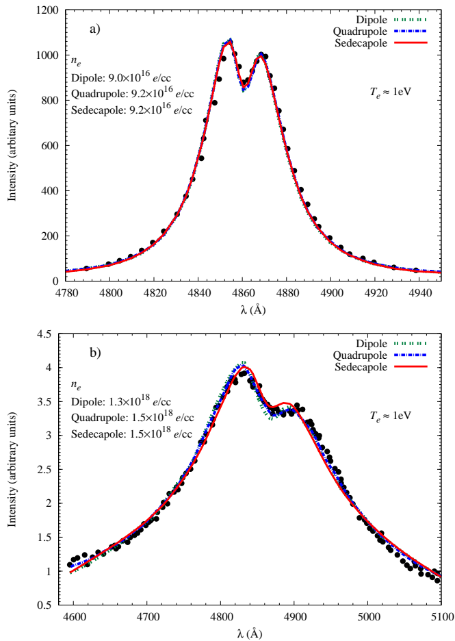
FIG. 4. a) the highest-density measured spectrum from the Wiese et al. [27] experiment, focused on H \beta (dots). The fits for the calculated dipole, quadrupole, and sedecapole profiles are identical, yielding fit differences less than the fit errors. b) the measured H \beta spectrum measured by Carlhoff et al. [23] (dots). The fits for the calculated dipole, quadrupole, and sedecapole profiles yield differences in density of 12%, which is greater than the fit errors.
