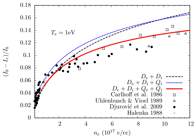
FIG. 2. Asymmetry calculations (lines) with different approximations: dipole-only interaction (black); dipole + ion-quadrupole (blue); dipole + electron- and ion-quadrupole moment (red). The dipole-only calculation agrees well with the data (various points) below 3 \times 10^{17} e/cc. Including only ion-quadrupole created discrepancy at these densities. Calculations including both electron- and ion-quadrupole terms created agreement with the data between 10^{17} and 10^{18} e/cc. Models assume 1eV temperature.
