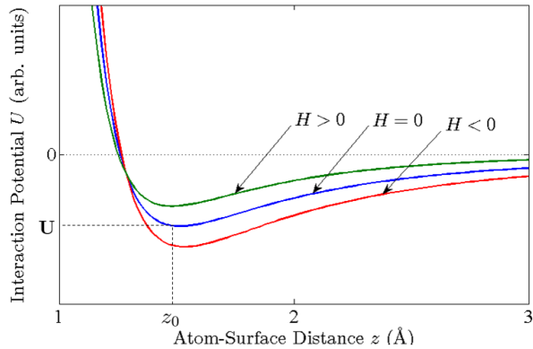
FIG. 2. Qualitative plot of interaction potential U(z) from Eq. 44 for surfaces that are planar H = 0 , have positive curvature H > 0 , and negative curvature H < 0 . The distance scale depicted is typical for adsorbates, in this case a hydrogen adatom on a gold surface. Note in particular the direction of the shift of the binding energy, defined as the minimum U = U(z_0) , and the transition frequency, defined through the second derivative of U(z) at z = z_0 . In the case of H-Ag interactions, z_0 \approx 1.5 \text{ \AA} .
