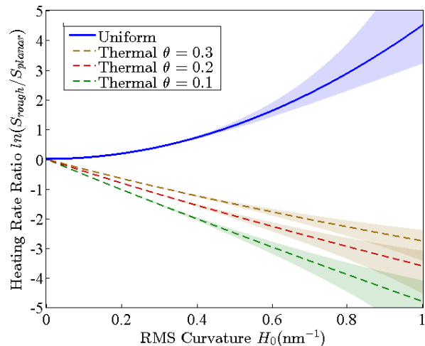
FIG. 4. Ratio of Heating rate for rough surfaces S_{\text{rough}} over planar surfaces S_{\text{planar}} with respect to root mean squared surface curvature H to first order in H . Normalized for the same number of adsorbates, a uniform distribution (thick) of adatoms sees a strong exponential enhancement. When the distribution relaxes to thermal equilibrium (dashed), heating rates are gradually suppressed depending on the filling fraction \theta of binding sites. The shaded area depicts the estimated contribution of higher order H^2 terms for typical physical surfaces. Parameter values used: h\nu_p/k_B = 200\text{K} , z_0 = 3\text{\AA} , T = 4\text{K} .
