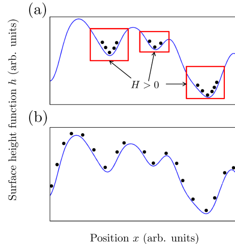
FIG. 3. Distribution of adatoms (dots) on a rough surface (line) in two limiting regimes. a) The thermal regime where atoms equilibrate at positions of positive curvature where the binding energy is enhanced. b) The uniform regime where atoms are uniformly distributed, such as at non-equilibrium, or if binding sites are full. The roughness (vertical axis) is exaggerated.
