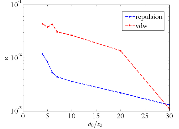
FIG. 5. \epsilon value for the van der Waal's potential (red) and the repulsion (blue) potential. For typical electrode surfaces, the error on the potential curve from approximating the whole surface as a parabolic surface is less than 5%, and therefore the parabolic approximation is valid.
