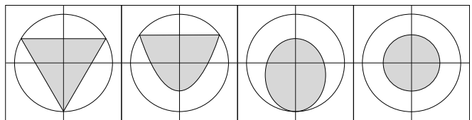
Figure 1: Cross-sections of the qutrit Bloch vector space. Allowed regions in the hypersphere are shaded.
