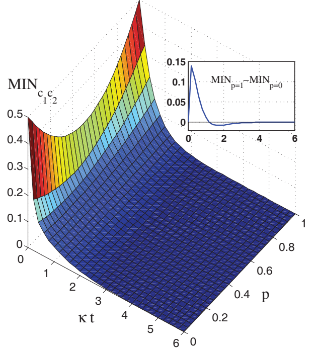
FIG. 2: (Color online) Evolution of the MIN of the MMES in two cavities, where the nonlocality is shown as a function of the time \kappa t and the probability p . The inset is the difference \text{MIN}_{p=1} - \text{MIN}_{p=0} as a function of \kappa t .
