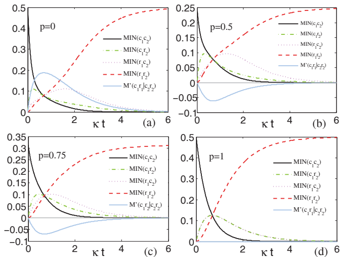
FIG. 4: (Color online) The MIN distribution of the MMES in multipartite 2 \otimes 2 \otimes 4 \otimes 4 cavity-reservoir systems, where the residual nonlocality M'_{c_1r_1|c_2r_2} can be positive, zero or negative as a function of the time parameter \kappa t .
