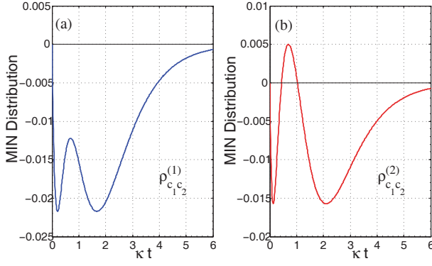
FIG. 7: (Color online) The MIN distributions of the MMESs in multipartite 2 \otimes 2 \otimes 6 \otimes 6 and 2 \otimes 2 \otimes 8 \otimes 8 cavity-reservoir systems are plotted as a function of \kappa t , where the negative values indicate that the MIN is not monogamous.
