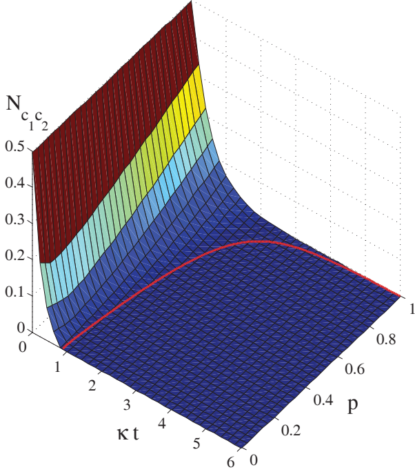
FIG. 1: (Color online) Evolution of entanglement of the MMES in two cavities, where the negativity is shown as a function of the time \kappa t and the probability p , and the red line indicates the entanglement sudden death of the two cavities.
