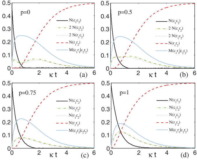
FIG. 3: (Color online) The distribution of negativity in the dissipation of multipartite 2 \otimes 2 \otimes 4 \otimes 4 cavity-reservoir systems, where the non-negative values of M_{c_1r_1|c_2r_2} indicate multipartite entanglement.
