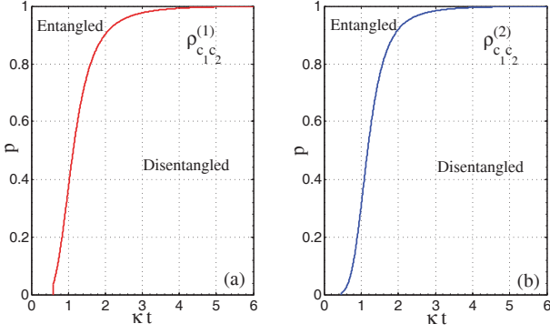
FIG. 6: (Color online) The ESD lines in the evolution of two cavities which are initially in the MMESs: (a) \rho_{c_1 c_2}^{(1)} in Eq. (D1), (b) \rho_{c_1 c_2}^{(2)} in Eq. (D6).
