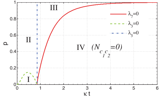
FIG. 5: (Color online) Four regions in the entanglement evolution of two cavities, where, in region IV, all three eigenvalues ( \lambda_3, \lambda_5, \lambda_7 ) are positive and the negativity N_{c_1c_2} becomes zero.
