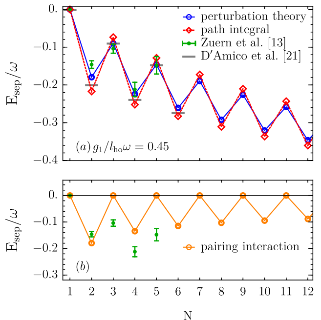
FIG. 1. (color online) (a) Separation energy as a function of particle number N for interaction strength g_1/l_{\text{ho}}\omega = 0.45 . The leading-order perturbative solution (7) and (8) is indicated by blue circles and the path integral fluctuation correction (25) by red diamonds. Lines are a guide for the eye. Our result is in excellent agreement with the experimental results by Zürn et al. [13], which are shown as green error bars. In addition, we compare with results from exact diagonalization [21], indicated by gray bars. (b) Orange line: separation energy including only pairing interactions. The Hartree density interaction is essential to fit the experimental data.
