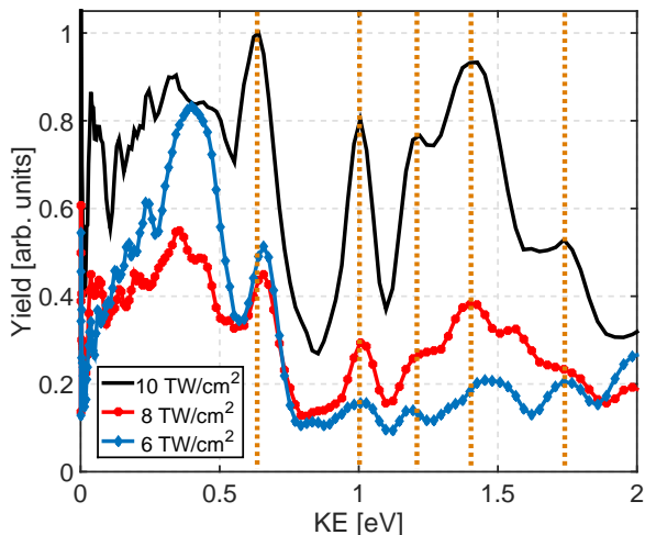
FIG. 3. Photoelectron spectra for \text{CF}_3\text{I} as a function of intensity produced with a 9 fs pulse from 6-10 \text{TW}/\text{cm}^2 . The dotted vertical lines mark positions of resonantly enhanced peaks.
