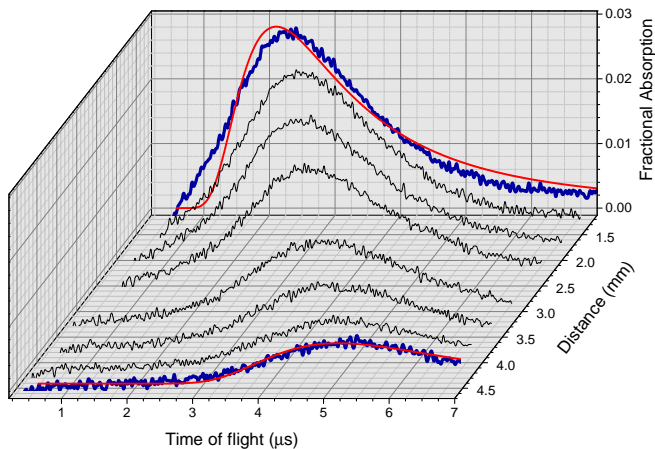
FIG. 3. TOF absorption signals (blue and black curves) of the BaH ablation plume recorded at different distances L of the probe laser from the target surface. The red lines represent the best fit to the data according to Eq. (3).
