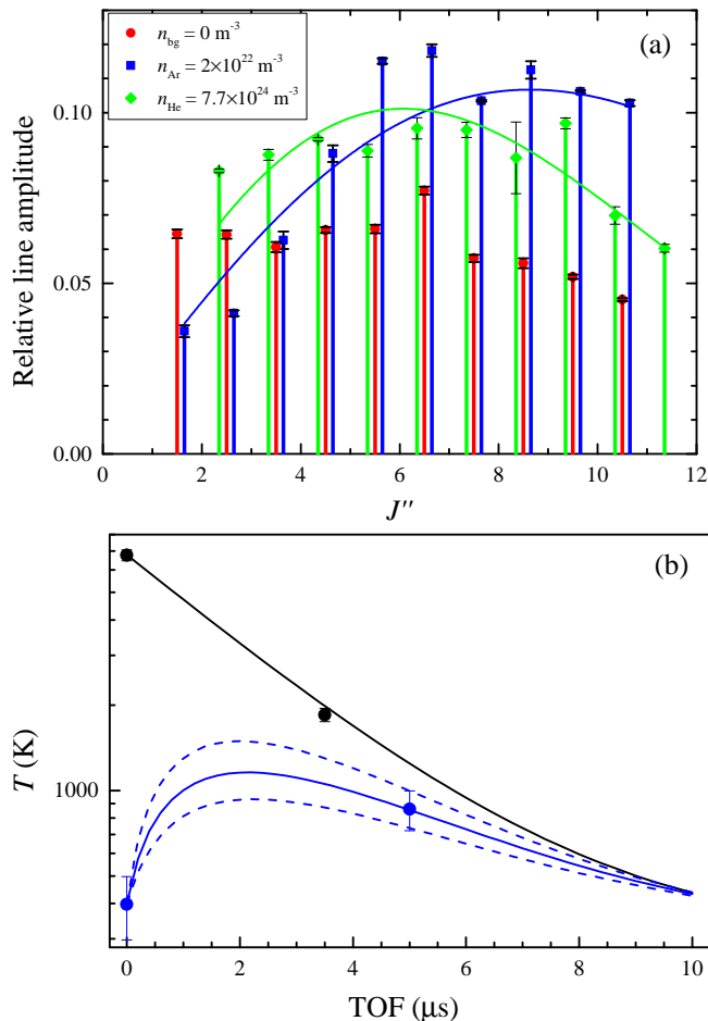
FIG. 6. Rotational cooling of ablated BaH by Ar and He buffer gases. (a) P_2 absorption lines for various ground-state rotational levels, for determining the rotational temperatures with and without a room temperature buffer gas. (b) The measured translational and vibrational thermalization for room temperature Ar at the density of 2 \times 10^{22} \text{ m}^{-3} , along with the fitted translational thermalization curve (black solid line) and the rotational thermalization curve with a thermalization rate chosen to best describe the data (blue solid line, with dashed lines showing the range consistent with the data).
