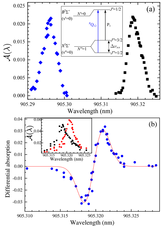
FIG. 7. B^2\Sigma^+(N' = 0) - X^2\Sigma^+(N'' = 1) spectroscopy. (a) Determination of the X^2\Sigma^+(N'' = 1) level spin-rotation splitting. (b) Doppler shift measurement for transverse spectroscopy on the P_1(1.5) cooling transition.
