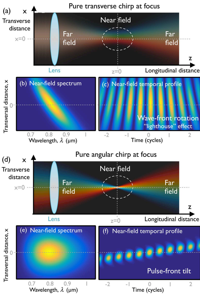
FIG. 1. (Color online) (a) Schematic of a beam with transverse chirp at the focal plane, with the transverse spectrum, |E(x, \lambda)|^2 , (b), and temporal profile, Re[E(x, t)]^2 , (c), of the electric field E at the focal plane. The variation of the local frequency across the focal spot leads to wavefronts with surface normal directions that vary from one cycle to the next, which has been applied to obtain the “lighthouse” effect. (d) Schematic of a beam with angular chirp at the focal plane proposed in this work to drive HHG: A transverse spatially chirped beam is focused, so each frequency beam propagates along a different direction, overlapping at the focal plane. The transverse spectrum, |E(x, \lambda)|^2 , (e), and temporal profile, Re[E(x, t)]^2 , (f), of the electric field E are shown both at the focal plane, where the beam exhibits a pulse front tilt with wavefronts all perpendicular to the optical axis.
