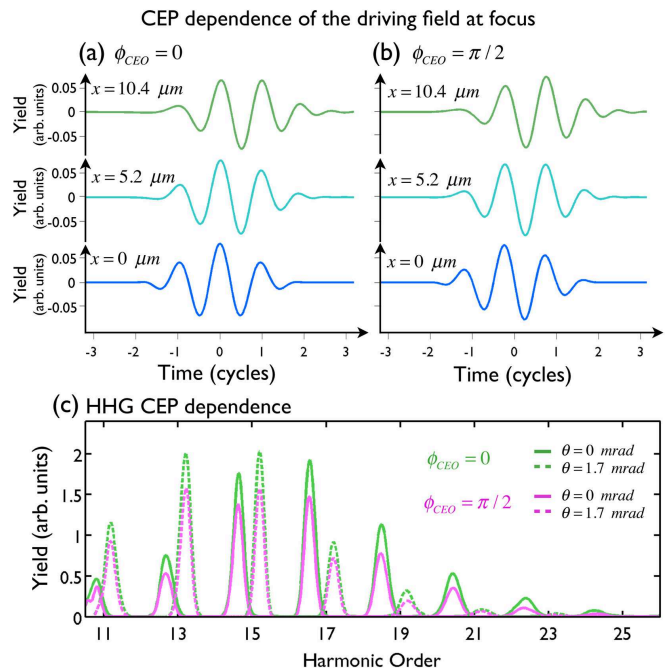
FIG. 4. (Color online) CEP invariance of angularly chirped HHG. (a) and (b) show the electric field at focus ( z=0 ) at three different transversal positions ( x=0, 5.2 \mu\text{m} and 10.4 \mu\text{m} ), with \phi_{CEO} = 0 and \phi_{CEO} = \pi/2 . (c) HHG spectrum (linear scale) detected at two angles (0 mrad-solid lines, 1.7 mrad-dashed lines), driven by an input angularly chirped beam with \tau_p = 3.8 fs, \gamma_0 = 16.4 as, and \phi_{CEO} = 0 (green) and \phi_{CEO} = \pi/2 (pink).
