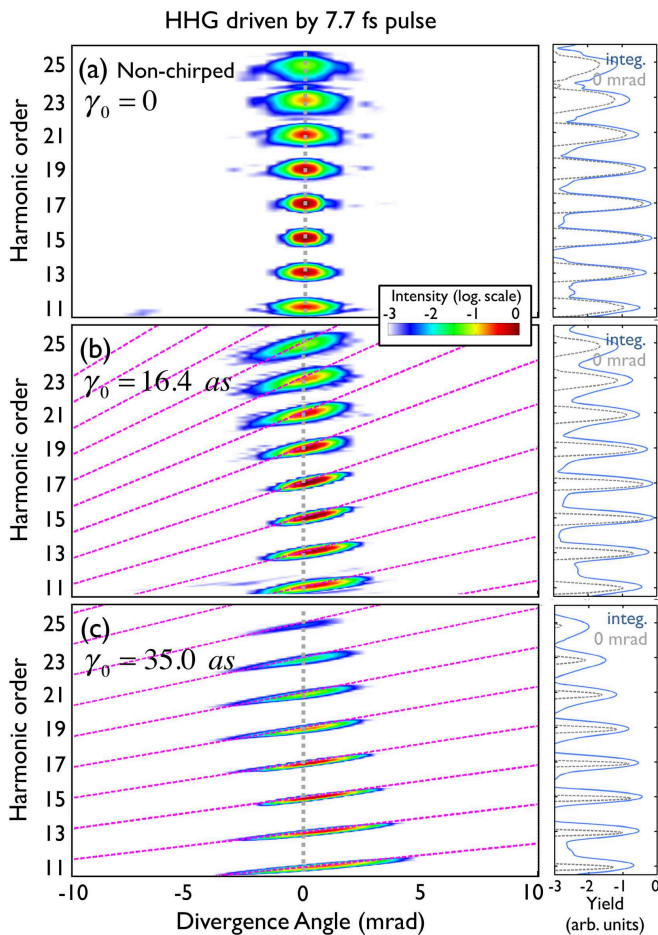
FIG. 2. (Color online) Angular distribution of high-order harmonics driven by a non-chirped (a) and an angularly chirped beam with (b) \gamma_0 = 16.4 as and (c) \gamma_0 = 35.0 as (other parameters: \lambda = 800 nm, \tau_p = 7.7 fs, \phi_{CEO} = 0 , E_0^2 = 2 \times 10^{14} W/cm 2 ). The dashed pink line represents the fitted angular chirp rate \gamma_q = \gamma_0/q . On the right of each panel is shown the angularly integrated (blue line) and the on-axis (dashed-grey line) spectrum.
