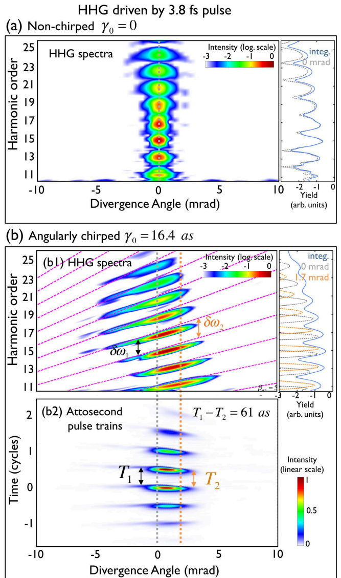
FIG. 3. (Color online) Angular distribution of the high-order harmonics driven by a \tau_p = 3.8 fs pulse, (a) without angular chirp, and (b) angularly chirped with \gamma_0 = 16.4 as. All other parameters of the beam are as in Fig. 2. On the right of panels (a) and (b1) is shown the angularly integrated (blue line) and the on-axis (dashed-grey line) spectrum. For the angularly chirped case, an additional spectrum at 1.75 mrad is shown (orange-dashed line). The dashed pink line in panel (b1) represents the model through the expected angular chirp rate \gamma_q = \gamma_0/q for each odd harmonic order. In panel (b2) we present the angular distribution of the attosecond pulse trains after Fourier transform of the spectra in panel (b1) and filtering the low-order harmonics q \leq 9 . Note, that the intensity yield is shown in logarithmic scale in (b1), but in linear scale in (b2). The periodicity of the attosecond pulse trains detected on-axis ( T_1 ) and at 1.75 mrad off-axis ( T_2 ) is modified by T_2 - T_1 = 61 as.
