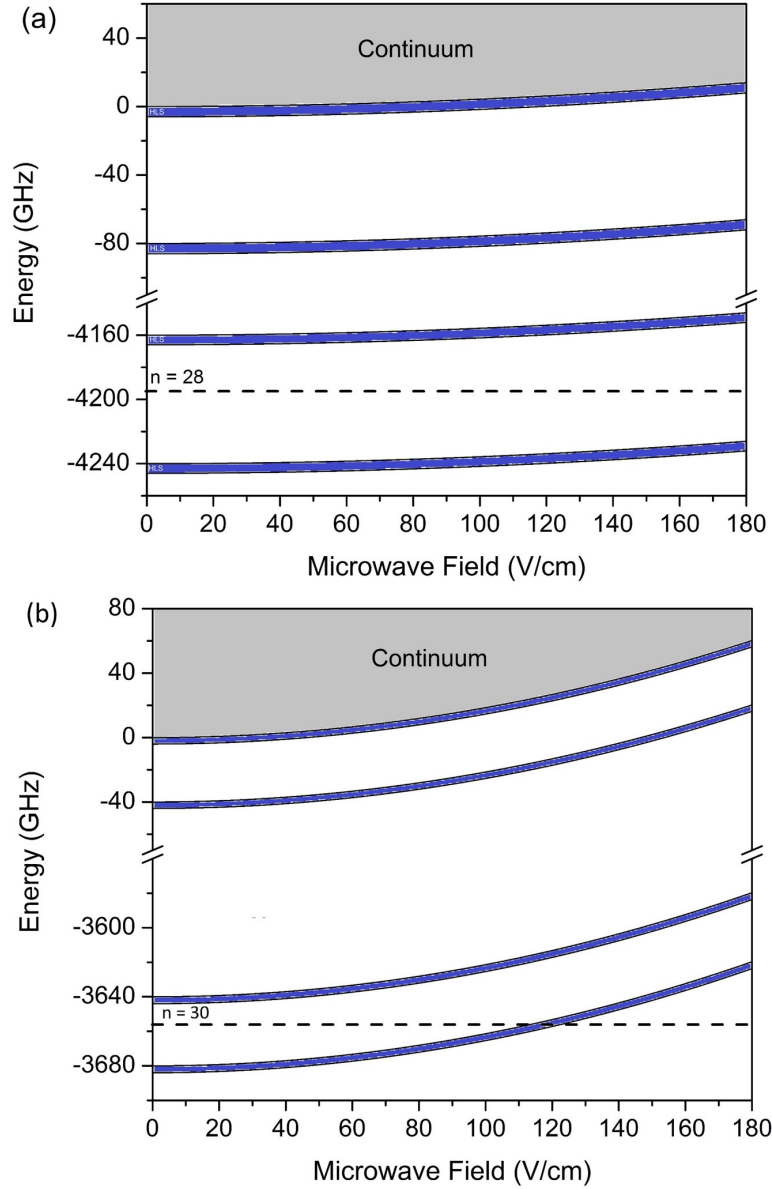
FIG. 7: (color online). (a) Energy level diagram vs amplitude of an 80-GHz microwave field. The band of the HLS is shown as a dark shaded band just below the continuum. It exhibits the ponderomotive shift to higher energy at higher microwave fields. There are Floquet states containing the HLS at integral multiples of 80 GHz below the HLS as shown. The n = 28 state lies between two of the Floquet states and does not come into resonance with the HLS before ionization occurs, and no HLS are produced. The HLS are only produced when a multiphoton resonance with the HLS exists. (b) The same energy level diagram as in (a) except that the frequency of the microwave field is 40 GHz. The ponderomotive shift is increased by a factor of four and the spacing between the Floquet levels is halved. Now, even a state with the maximum detuning, as shown for n = 30 , comes into a multiphoton resonance with the HLS, and the HLS are produced for all initially populated Rydberg states.
