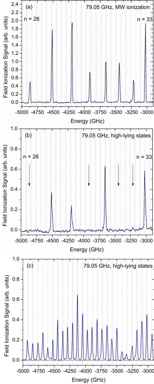
FIG. 1: (color online). Frequency scans of the third laser over the energy range from 5000 to 3000 GHz below the ionization limit, encompassing states from n = 26 to 33. The horizontal scale is the energy relative to the ionization limit. (a) Microwave ionization signal observed when the atoms are exposed to a 200-ns long, 170-V/cm, 79.05-GHz microwave pulse subsequent to laser excitation. For all states at least 40% of the atoms initially excited are ionized by the microwave pulse. (b) The same timing sequence and the microwave pulse as in (a), but atoms in the HLS are detected instead of microwave ionization. No HLS are observed for n = 26, 29, 31, and 32 . The arrows indicate where the HLS signals should appear. The HLS are only observed when there is a multiphoton resonance between the initial Rydberg states and the HLS. The vertical dotted lines indicate the calculated locations of the Floquet states based on the HLS. (c) Spectrum observed when the laser excitation occurs in the presence of the 170-V/cm 79.05-GHz field. In this case a regular series of peaks 79.05 GHz apart is observed, extending from the limit to more than 5000 GHz below the limit. The peaks are Floquet states containing the HLS and occur at the locations of multiphoton resonances with the limit. The n states in (b) for which the HLS are observed are in multiphoton resonance with the HLS.
