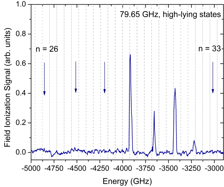
FIG. 3: (color online). Frequency scan over the same range as shown in Fig. 1. The microwave pulse is subsequent to laser excitation of the Rydberg states, and atoms in the HLS are detected. The microwave field is again 170 V/cm, but the frequency has been changed to 79.65 GHz. Now the HLS are produced for different n states than in Fig. 1 (b). The arrows again indicate missing states. As in Fig. 1 (b) the dotted lines indicate the calculated locations of the Floquet states based on the HLS. Only initial states in multiphoton resonance with the HLS lead to the observation of the HLS.
