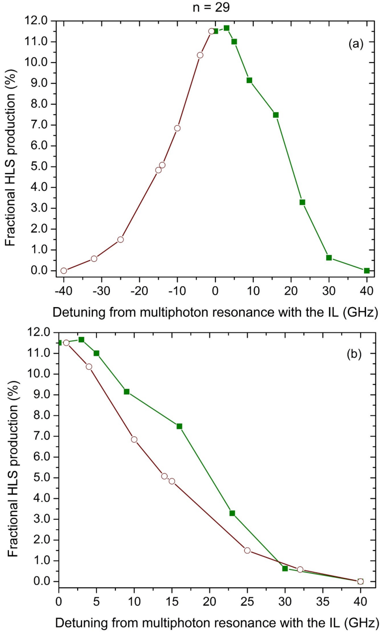
FIG. 4: (color online). (a) Fractional population in the HLS following the excitation of the 29f state vs the detuning between the 29f state and the multiphoton resonance with the HLS. (b) The same data as in (a) but plotted vs the magnitude of the detuning to show the difference between positive detunings (■) and negative detunings (○). The difference arises because the ponderomotive energy shift brings small positive detunings into resonance.
