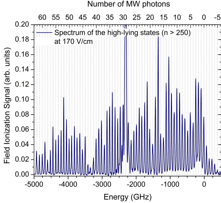
FIG. 2: (color online). Frequency scan of the third laser from 5000 GHz below the limit to 500 GHz above the limit. The laser excitation occurs in the presence of a 170-V/cm 79.05-GHz microwave field, the same conditions as in Fig. 1 (c). The spectrum shown in Fig. 1 (c) is simply a section of this spectrum. As in Fig. 1, the vertical dotted lines indicate the calculated locations of the Floquet states based on the HLS.
