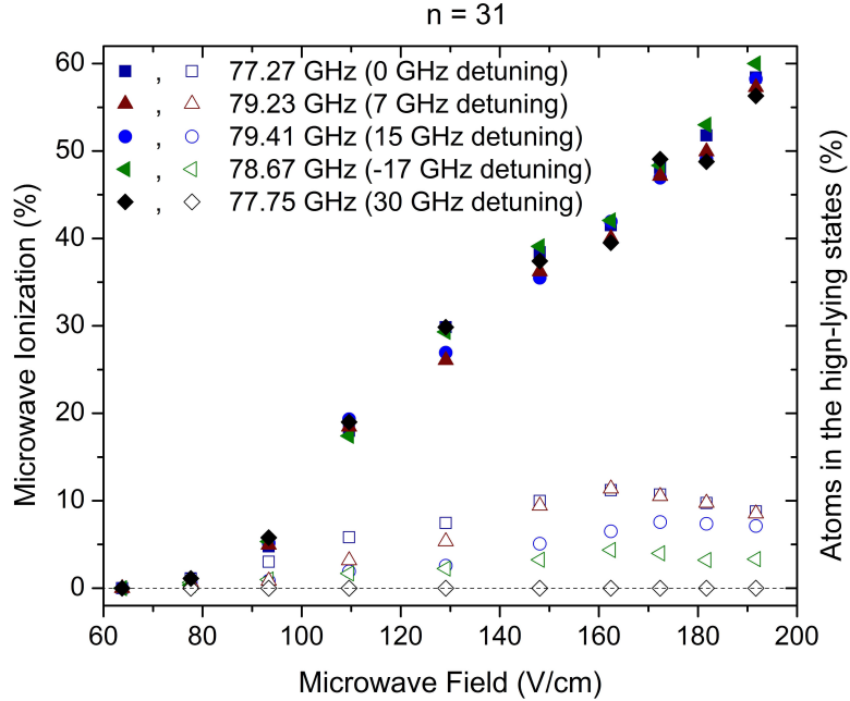
FIG. 5: (color online). Microwave ionization and the HLS production subsequent to the initial excitation of the 31f state vs. detuning from multiphoton resonance with the HLS. The microwave ionization signals are shown as solid symbols and the HLS production as open symbols. 0 GHz detuning (77.27 GHz) ( \blacksquare, \square ), 7 GHz detuning (79.23 GHz) ( \blacktriangle, \triangle ), 15 GHz detuning (79.41 GHz) ( \bullet, \circ ), -17 GHz detuning (78.67 GHz) ( \blacktriangleleft, \triangleleft ), and 30 GHz detuning (77.75 GHz) ( \blacklozenge, \lozenge ). The microwave ionization signals are essentially identical, but the number of atoms left in the HLS is peaked at the multiphoton resonance with the HLS.
