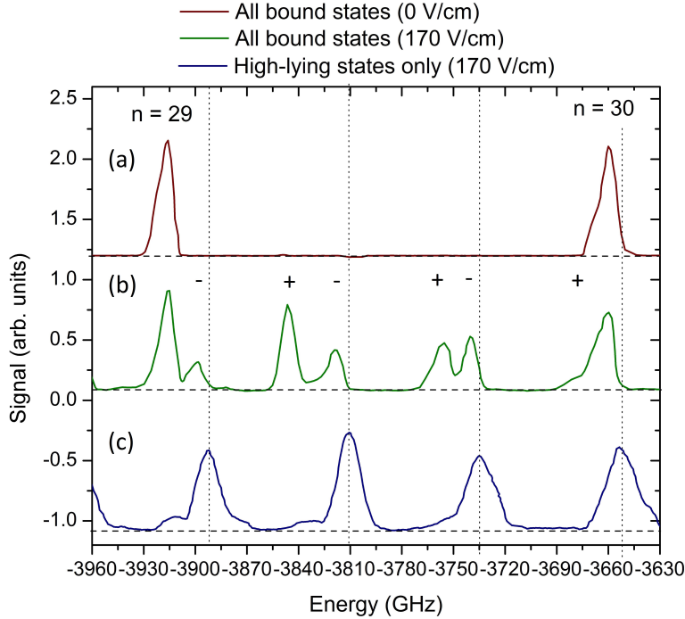
FIG. 6: (color online). Spectra observed when scanning the laser over the range including n = 29 and n = 30 . (a) Laser excitation occurs in zero field, and the atoms are subsequently ionized by a 170-V/cm 79.05-GHz microwave pulse. (b) Atoms are excited in the presence of the 170-V/cm microwave pulse and ions are detected. In this case the only effect of the microwave field is the generation of sidebands displaced from the zero field states of (a) by multiples of 79.05 GHz. There are no measurable shifts. The lower n = 30 sidebands are indicated by - and the upper n = 29 sidebands by + . (c) Spectrum observed when laser excitation occurs in the presence of the 170-V/cm field, and the HLS are detected. A spectrum similar to those shown in Figs. 1 (c) and 2 are observed. This spectrum has no particular relation to the one shown in (b). As before, the dotted vertical lines indicate the calculated locations of the Floquet states based on the HLS.
