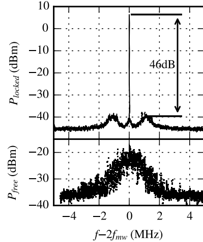
FIG. 4. Spectra of the laser beat note acquired by the spectrum analyzer shown in Fig. 3. The frequency is offset by twice the microwave frequency 2f_{mw} . Top: Laser beat signal locked at 2f_{mw} = 28 GHz (RBW: 1kHz, no averaging). Bottom : Beat note spectrum when the lasers are free running (RBW: 10 kHz, no averaging).
