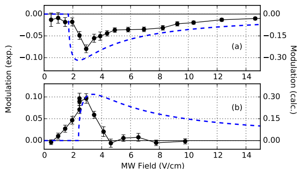
FIG. 6. (Color online) Peak-to-Peak modulation of the Rydberg state signal as a function of microwave field E_{mw} when the laser is tuned (a) 17 GHz below and (b) 25 GHz above the ionization limit. The experimental data points have error bars and the results of a classical calculation are shown as broken lines. The negative modulation in (a) reflects the phase inversion between Fig. 5(a) and Fig. 5(b). Note the factor of three difference in the two vertical scales.
