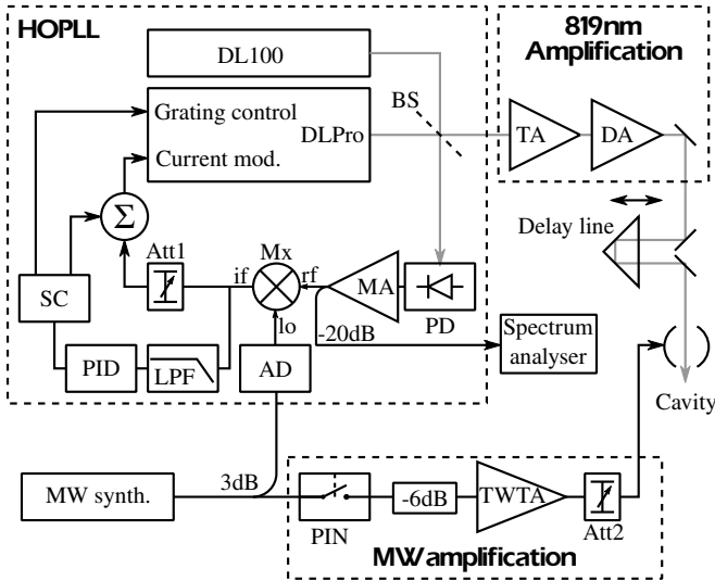
FIG. 3. Scheme of the experimental apparatus encompassing three different functions: generating the amplitude modulated IR excitation laser, generating the microwave field, and phase-locking the envelope of the 819 nm field to the microwave field as shown in Fig 2. The 819 nm AMLaser is generated by the DL Pro and DL 100 lasers superimposed on the beamsplitter (BS), and then amplified by the IR amplification chain. The microwaves are generated by a microwave synthesizer, formed into pulses by the PIN-diode switch (PIN) and amplified by the Traveling Wave Tube Amplifier (TWTA) before injection in the cavity. The locking of the 819 nm field envelope to the microwave field is performed an Heterodyne Optical Phase Locked Loop (HOPLL).
