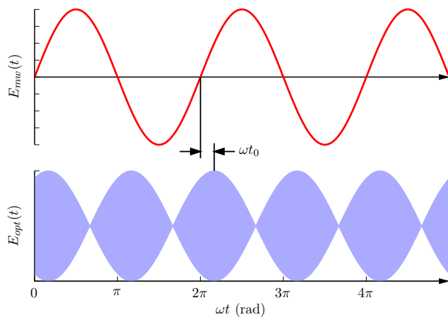
FIG. 2. (Color online) Temporal view of the microwave field (top) phase-locked with the amplitude modulated laser field E_{opt} (bottom). The maximum optical field occurs at the microwave phase \omega t_0 , and it is varied using an optical delay line. In the figure, \omega t_0 = \pi/6 , approximately the phase at which maximum energy transfer occurs.
