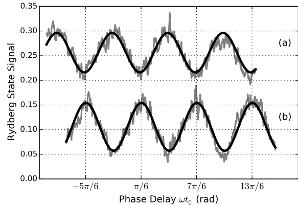
FIG. 5. Rydberg state signal as a function of phase \omega t_0 between the microwave field and laser envelope for two different laser tunings: (a) \omega_o/2\pi is 17 GHz below the ionization limit, (b) \omega_o/2\pi is 25 GHz above the limit. In both cases the microwave field is E_{mw} = 3 V/cm. The data (light gray) are fit to a sine function (black) to extract the peak-to-peak modulation. The total number of excited atoms in nf or \epsilon f states is 1.00 on this scale. The phase origin for the horizontal scale is chosen to have the maximum energy transfer up and down at \pi/6 , in accordance with the results of our classical calculation. We observed that the two fits are inverted within 0.3 radian.
