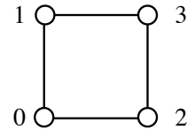
FIG. 2. Labeling of the sites in a plaquettes
