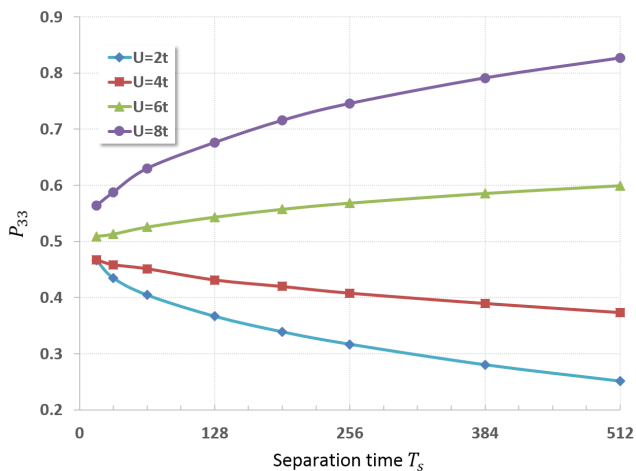
FIG. 6. Shown is the probability P_{33} of finding three electrons on each of the plaquette after decoupling two plaquettes with a total of six electrons as a function of the time T_s (in units of t^{-1} ) over which the plaquettes were nearly adiabatically separated. A decrease of P_{33} indicates pairing of holes in the ground state of a plaquette.
