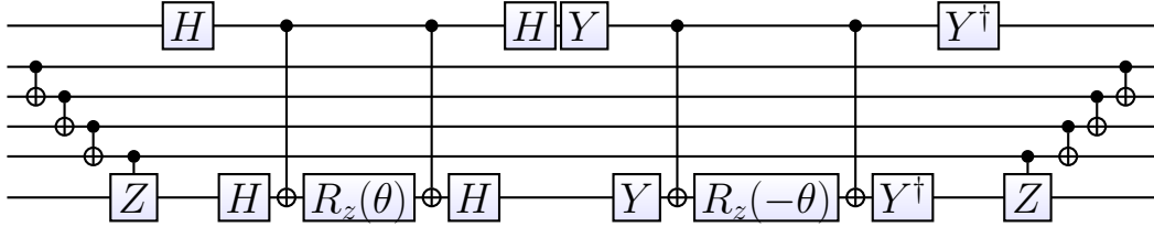
FIG. 10. Quantum circuit to implement time evolution for a time step \theta under the pairing term c_{p,\sigma}^\dagger c_{q,\sigma'}^\dagger + c_{q,\sigma'} c_{p,\sigma} . Top and bottom lines represent qubits for p, \sigma and q, \sigma' .
