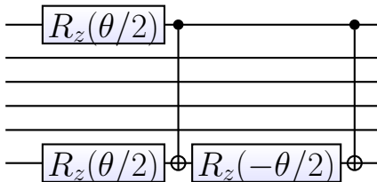
FIG. 7. Quantum circuit to implement time evolution for a time step \theta under the term H_{pqpp} = n_{p,\sigma}n_{q,\sigma'} = c_{p,\sigma}^\dagger c_{q,\sigma'}^\dagger c_{q,\sigma'} c_{p,\sigma} . Top and bottom lines represent qubits for p, \sigma and q, \sigma' .
