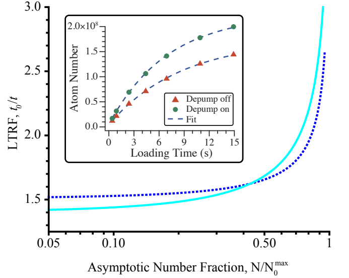
FIG. 6. (Color online) The Loading Time Reduction Factor (LTRF) for ^{88}\text{Sr} (dotted blue line) and ^{84}\text{Sr} (solid cyan line). The saturated atom number, N_0^{\max} , is the asymptote of the trap loading curve with the 688-nm laser off (for ^{88}\text{Sr} , red triangles, inset). The loading time necessary to transfer N atoms into the rMOT with the depump laser on (off) is given by t ( t_0 ). Inset: The raw data and fits associated with the ^{88}\text{Sr} (dotted blue) LTRF curve. The standard error is smaller than the data points. We find t and t_0 by inverting the appropriate fit function (see text).
