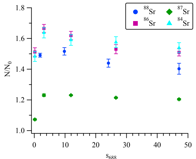
FIG. 5. (Color online) Atom number enhancement versus s_{688} with w_{688} = 1.35 mm. ^{87}\text{Sr} data are for the F=11/2 \rightarrow F'=11/2 transition and all isotopes are recaptured in the rMOT. Error bars represent the standard error in the mean for \geq 10 measurements. The 688-nm and 679-nm laser detunings are set to \approx 30 MHz.
