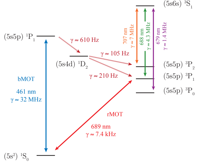
FIG. 1. (Color online) The low-lying energy levels of bosonic strontium taken from [1, 23, 24]. A Magneto-Optical Trap operating on the blue, 461-nm transition (bMOT) captures atoms from a Zeeman-slowed beam. Atoms in the bMOT continuously leak into the long-lived {}^3P_2 state, which is magnetically trapped by the bMOT quadrupole field. Two lasers at 688 nm and 679 nm increase the magnetic trap loading rate by pumping atoms that populate {}^3P_1 into {}^3P_2 . The 679-nm laser and a 707-nm laser return atoms to the ground state via the {}^3P_1 state once magnetic trap loading is complete. A Magneto-Optical Trap operating on the red, 689-nm transition (rMOT) then cools the sample to \approx 1 \mu\text{K} .
