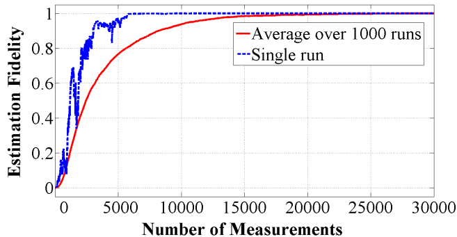
FIG. 2. (Color online) Estimation of the Larmor frequency and axis of rotation for a spin-1/2 particle. The estimation fidelity for the probability distribution of the dynamical parameters as a function of the number of measurements for a single run (dashed blue line) and averaged over 1000 runs (red line)
