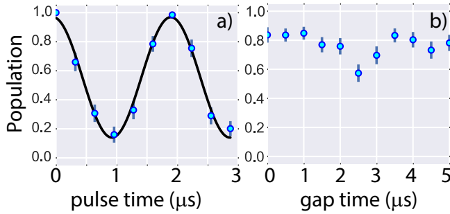
FIG. 8. (color online) Ground state population after a 2\pi Rydberg pulse a) and after a \pi -gap -\pi Rydberg pulse sequence with variable gap time b).
