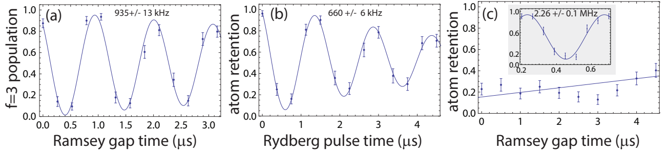
FIG. 3. (color online) Experimental data used to determine optical beam powers. The figure shows measurements on the control site only and fitted frequencies are indicated in the plots. (a) ground state Ramsey oscillations with 459 nm laser used to extract \Omega_1 . (b) ground-Rydberg Rabi oscillations used to extract \Omega_2 once \Omega_1 and \Delta_1 are known. (c) ground-Rydberg Ramsey experiment used to measure \Delta_{\text{diff,gR}} . The straight line is an aid to the eye and is not a fit, but suggests a frequency < 0.1 MHz. The inset shows a faster ground-Rydberg Ramsey oscillation using other parameters. Beam powers extracted from these measurements are given in Table II.
