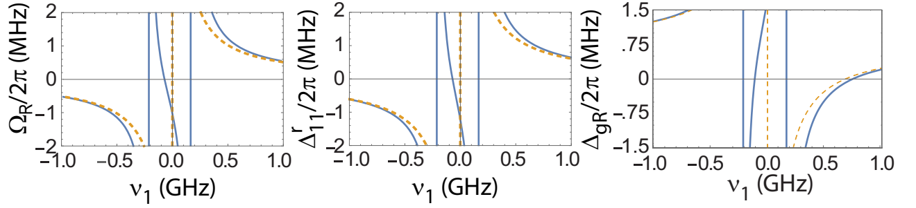
FIG. 9. (color online) Calculated ground-Rabi frequency \Omega_R (left), resonant Stark shift of |6s_{1/2}, f = 4\rangle due to the 459 nm light \Delta_{11}^r (center), and total ground-Rydberg differential Stark shift \Delta_{gR} including resonant and non-resonant contributions (right), for two-photon excitation of Cs |82s, m_j = -1/2\rangle starting in |4, 0\rangle using parameters from Table II for the control site. Solid blue curves account for the 7p_{1/2} hyperfine structure, while the dashed yellow curves do not include hyperfine corrections. The spontaneous emission plot only accounts for scattering from 7p_{1/2} as the Rydberg state decay is negligible for the parameters used. The gate experiments used \nu_1 = 0.83 GHz.
