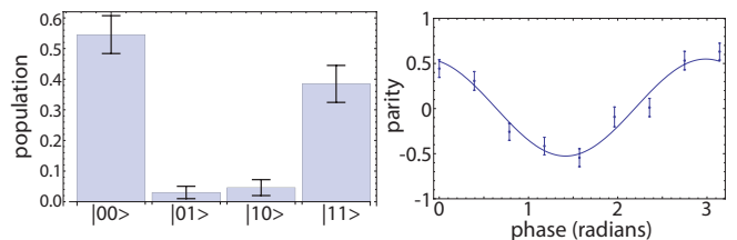
FIG. 6. (color online) Bell state population measurement and parity oscillation measurement with no loss correction using next nearest neighbor sites. The populations measured for the Bell state are |00\rangle : 0.54 \pm 0.06 , |01\rangle : 0.03 \pm 0.02 , |10\rangle : 0.05 \pm 0.03 , |11\rangle : 0.38 \pm 0.06 . The fit to the parity curve gives |C_1| = 0.27 \pm 0.02 and |C_2| = 0.006 . This results in an entanglement fidelity F = 0.73 \pm 0.05 and F = 0.79 \pm 0.05 when corrected for atom loss.
