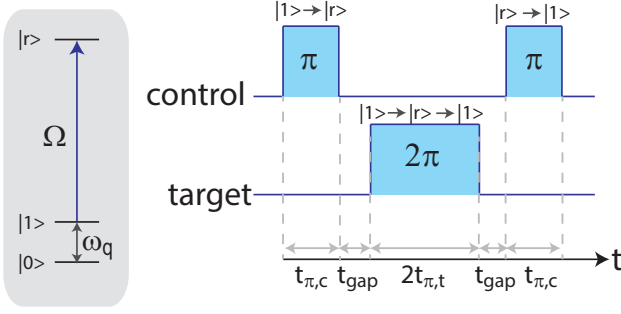
FIG. 1. (color online) Level structure (left) and pulse sequence (right) for two-qubit Rydberg blockade C_Z gate. The qubits are encoded in ground hyperfine states |0\rangle , |1\rangle while |r\rangle is a high lying Rydberg state.
