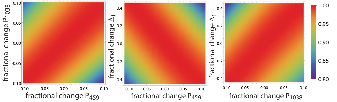
FIG. 7. (color online) The entanglement fidelity as a function of the fractional change of the optical powers P_{459} , P_{1038} and the detuning \Delta_1 from the optimal values. The center point of each plot uses the parameters found experimentally in Sec. III B and the color scale is the fidelity normalized by the value at the center of each panel.
