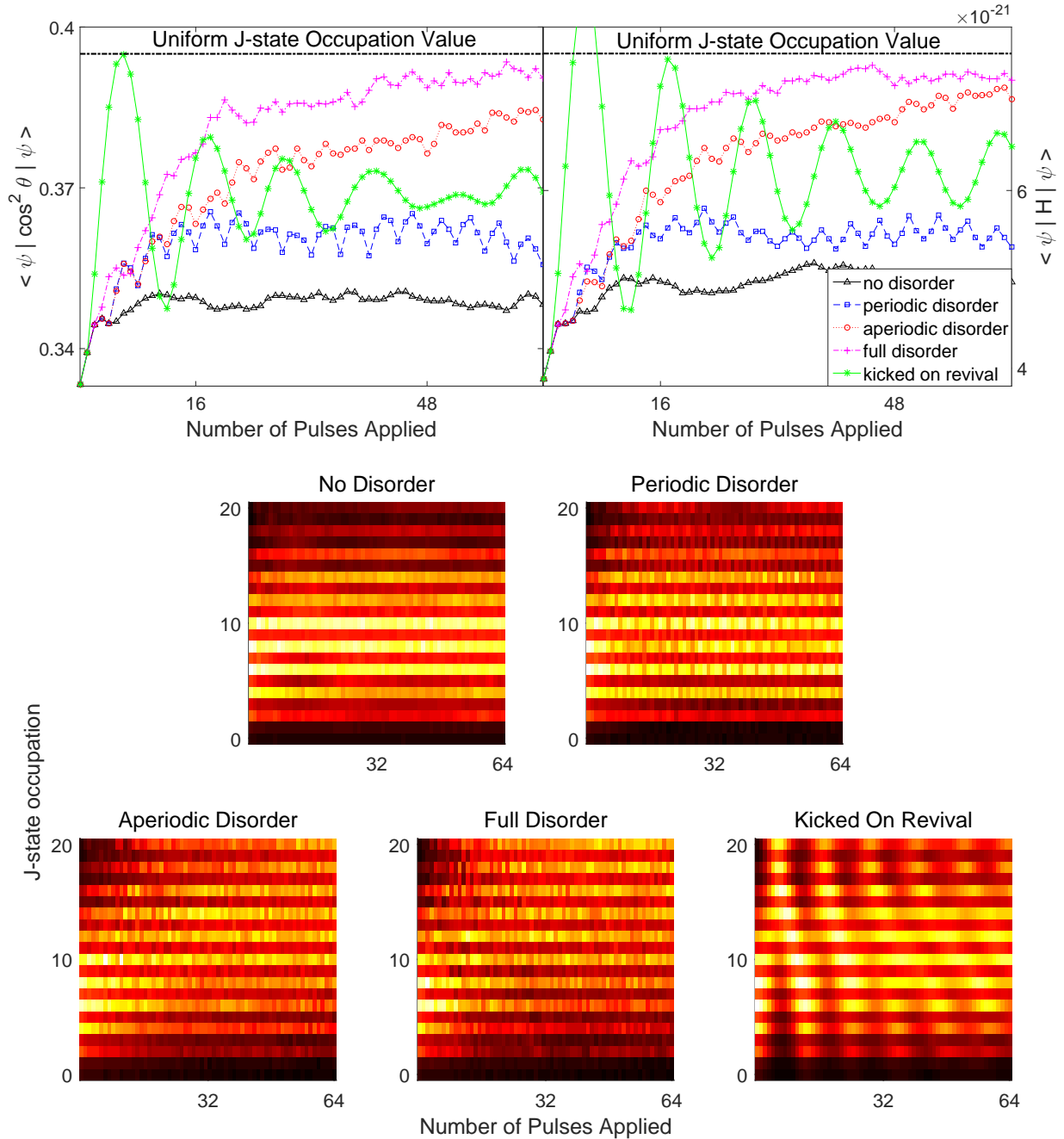
FIG. 1. Simulated population alignment and energy for extended pulse trains with different levels of spacing disorder. The train with no disorder is a pulse train with uniform \tau = 1.159T_{rev} = \frac{2\pi+1}{2\pi}T_{rev} . The periodic disorder train consists of a repeating series with three spacings of \tau = 1.159T_{rev} and a fourth spacing of \tau = 1.183T_{rev} . The aperiodic disorder train is similar to the periodic sequence, except every fourth spacing is a randomly generated value within the range \tau = [1.159T_{rev}, 1.207T_{rev}] . The full disordered train uses random values within the range \tau = [1.159T_{rev}, 1.207T_{rev}] for all spacings. The train that excites ^{14}\text{N} with kicks on revival is periodic with all \tau = T_{rev} ; it is plotted here for reference only. The rotational energy of ^{14}\text{N} is plotted for comparison to theoretical studies of dynamical localization. The relationship between these two values is not one-to-one but shows matching behaviors, especially in terms of boundedness. The color maps indicate the J-state population distribution as a function of kick count for each of the applied pulse trains. The mapped J-states are summed up over directional angular momentum degeneracy. Brighter colors indicate higher state occupation. The peak intensity used for this simulation is 1.2 \cdot 10^{14} \frac{\text{W}}{\text{cm}^2} . T_{rev} is the well known ^{14}\text{N} alignment revival time of 8.38 ps.
