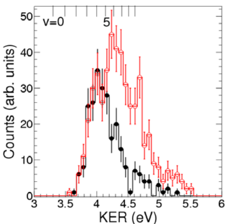
FIG. 3: (color online) Vibrational level progression for the main feature of the H^+ + C_2H_3^+ channel. The KER distribution is shown for selected Auger electron energies E_{Auger} [solid black circles for E_{Auger} = 259 to 260 eV and open red circles for E_{Auger} = 255 to 257 eV energy range]. The vertical lines on the top axis represent the expected KER for the respective vibrational levels.
