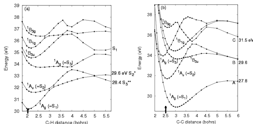
FIG. 2: Cut of the selected singlet potential energy surfaces (PEs) of the ethylene dication for the (a) C-H and (b) C-C distance calculated using the multi-configuration self-consistent field method (adapted from Ref. [29]). The black arrows at the horizontal axis show the center of the Franck-Condon region.
