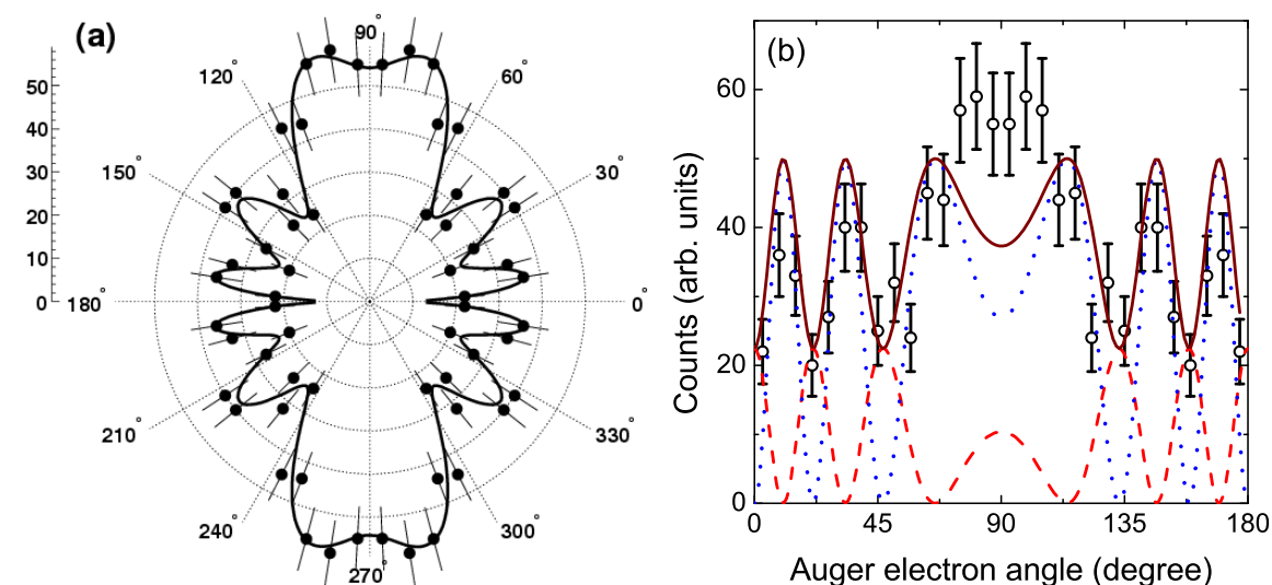
FIG. 6: (color online) Molecular frame Auger electron angular distribution (molecule is horizontal) for the island-like feature of the symmetric breakup channel (feature III in Fig. 1b). For the fitting with spherical harmonics (line) in (a) l = 0 to 4 and m = 0 , and +/-1 are needed. The circles in (b) represent the measured data while the dashed and dotted lines represent the cosine and sine functions of the diffraction patterns of the Auger electrons from g and u states. The solid line represents the incoherent sum of both contributions. The molecular axis is horizontal and the paper plane represents the polarization plane of the circular polarized light.
