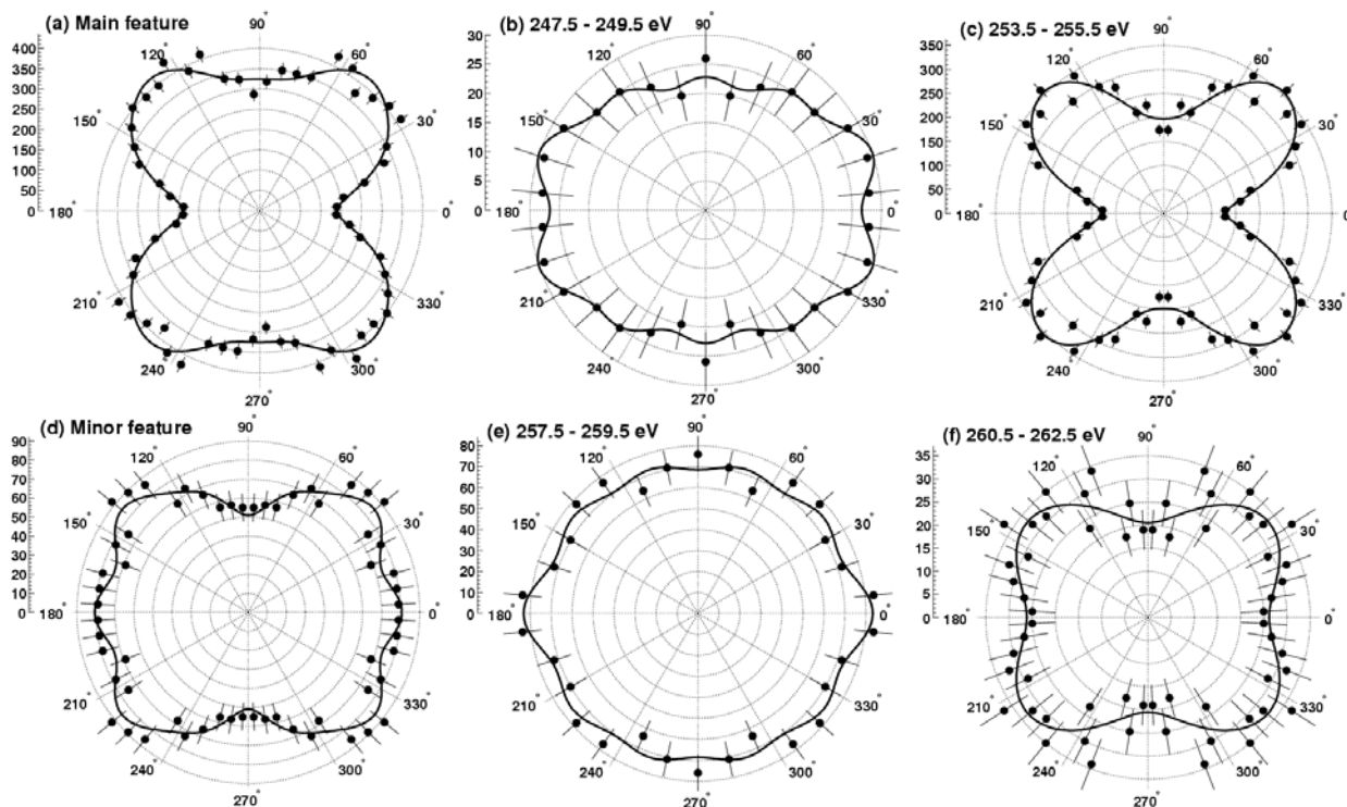
FIG. 5: Auger electron angular distributions (molecular axis is horizontal) for two different features (a) and (d) and four different Auger electron energies E_{\text{Auger}} intervals (b, c, e, and f) of the symmetric breakup channel in Fig. 1(b): (a) main feature I, (b) E_{\text{Auger}} = 247.5 - 249.5 eV, (c) E_{\text{Auger}} = 253.5 - 255.5 eV, (d) minor feature II, (e) E_{\text{Auger}} = 257.5 - 259.5 eV, and (f) E_{\text{Auger}} = 260.5 - 262.5 eV. For the fitting with spherical harmonics (lines) l = 0 to 4 and m = 0 are used. The molecular axis is horizontal and the paper plane represents the polarization plane of the circular polarized light.
