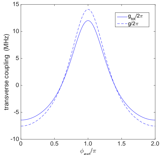
FIG. 7. (Color online) Coupling strength in the perturbative nonlinear approximation for system parameters given in Table I. The dashed line is coupling (44) in the linearized model.
