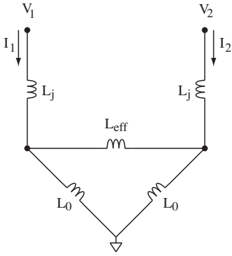
FIG. 8. Network of linear inductors.
