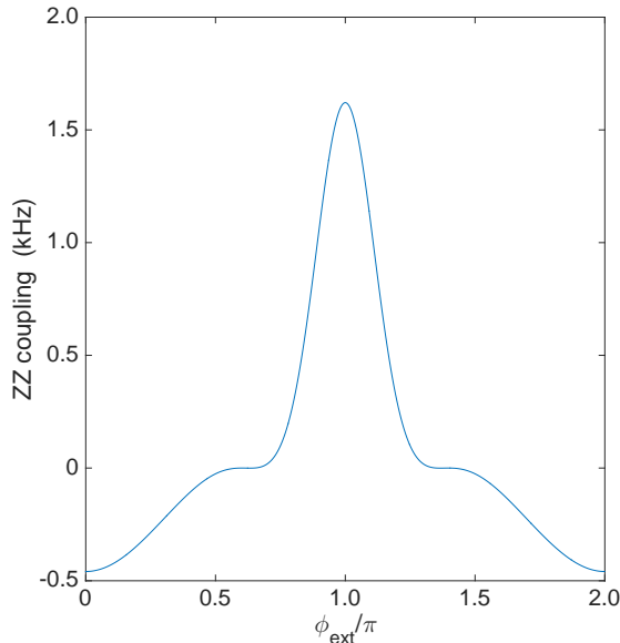
FIG. 6. (Color online) Subdominant contribution (57) to the diagonal coupling J , versus flux. This contribution zeros when g does.
