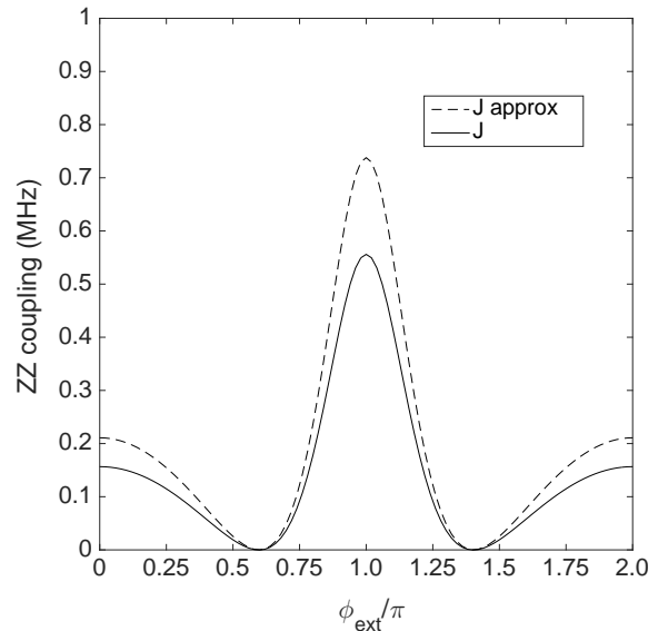
FIG. 5. Diagonal coupling strength (50) computed by exact diagonalization, and the approximation (55).
