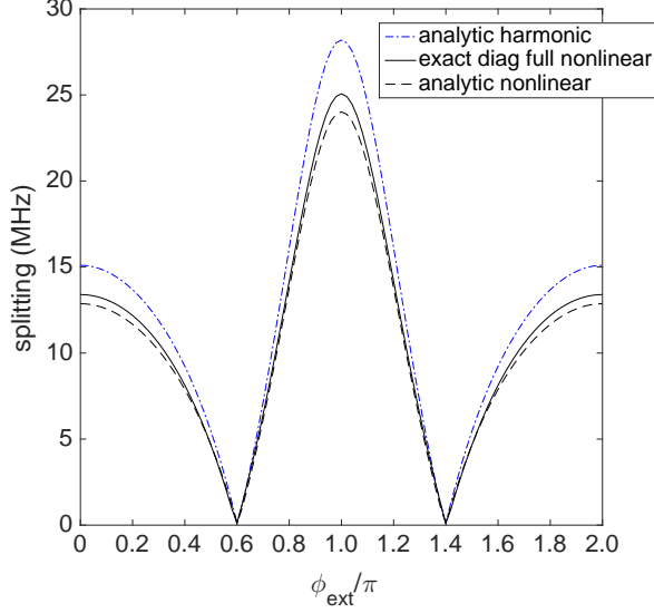
FIG. 3. (Color online) Splitting (equal to twice the magnitude of the coupling) in the fully nonlinear model (18) calculated by exact diagonalization (solid curve). Also shown are the corresponding harmonic approximation (dashed-dotted curve) and perturbative nonlinear (dashed) results.
