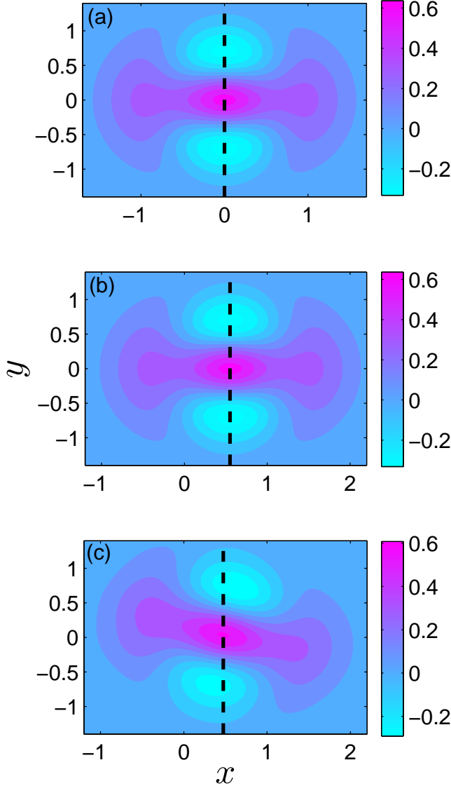
FIG. 6: Wigner functions (a) \mathcal{W}_c^I(\beta, \beta^*) , (b) \mathcal{W}_c^D(\beta, \beta^*) , (c) \mathcal{W}_c^A(\beta, \beta^*) respectively for (a) \rho_c^I , (b) \rho_c^D , and (c) \rho_c^A . Here x = \text{Re}(\beta) , and y = \text{Im}(\beta) . In the above figures, the parameters are chosen as \omega_z/2\pi = 19.5 GHz, \omega_x = 1.6 GHz, \omega = 2 GHz, \gamma_{21}/2\pi = \kappa/2\pi = 1 MHz, \gamma_{11} = 0 , \gamma_{22} = 0.1 MHz, \eta = \eta_m = 1.11 , and x_d = x_d^m = 1.305 . We have used a vertical dashed line in (a), (b), and (c) to highlight the displacement of the central point, also the maximum point, of the Wigner functions. As shown in (a), the central point of \mathcal{W}_c^I(\beta, \beta^*) is the origin. Since \rho_c^D = D(\eta_m/2)\rho_c^I D^\dagger(\eta_m/2) , the Wigner function for \rho_c^D , \mathcal{W}_c^D(\beta, \beta^*) and that for \rho_c^I , \mathcal{W}_c^I(\beta, \beta^*) have the relation \mathcal{W}_c^D(\beta, \beta^*) = \mathcal{W}_c^I(\beta - \eta_m/2, \beta^* - \eta_m/2) . This is the very reason why (a) and (b) exhibit the same profile as well as a horizontal translation. The exact value of this translation length is, of course, \eta_m/2 = 0.555 . Compared to the ideal target state in the original picture, i.e., \mathcal{W}_c^D(\beta, \beta^*) in (b), the actual target state \mathcal{W}_c^A(\beta, \beta^*) in (c) possesses nearly the same central point. But due to the effects of environment and unwanted terms, there appears, in (c), a new feature of small local twists and a global rotation.
