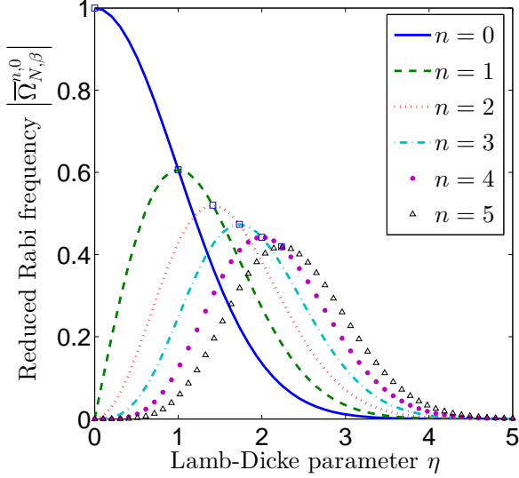
FIG. 7: (color online) Reduced Rabi frequency |\bar{\Omega}_{N,\beta}^{n,0}| , from Eq. (A22), as a function of \eta , for n = 1, 2, 3, 4 , and 5 , respectively. The square on each plot denotes the point that achieves the largest |\bar{\Omega}_{N,\beta}^{n,0}| . Recall that \eta = 2g/\omega , where g is the qubit-cavity coupling constant and \omega is the frequency of the single-mode cavity field. Thus, \eta is the normalized coupling.
