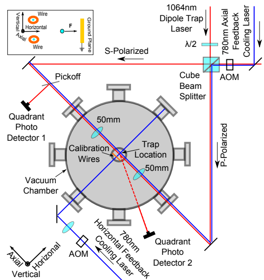
FIG. 1: (Color Online) The optical dipole trap is created by focusing two orthogonally polarized laser beams using 50 \text{ mm} focal length inside a vacuum chamber. A 780 \text{ nm} laser provides active feedback cooling to stabilize the trapped beads in vacuum and provide optical damping. (inset) A set of calibration electrodes is used to conduct force measurements with a known applied electric field at the location of the trap.
