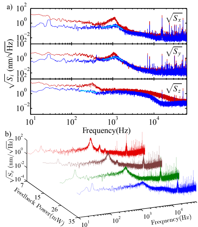
FIG. 4: (Color Online) (a) Typical position spectrum of a bead held at low vacuum of 1.7 Torr with no feedback cooling applied (red), and at high vacuum of 5 \times 10^{-6} \text{ Torr} with feedback cooling applied (blue). Also shown (light blue) is a Lorentzian fit to the peaks in the high vacuum data, with fit parameters as discussed in the text. (b) x - spectrum of a bead at 5 \times 10^{-6} \text{ Torr} with varying feedback cooling rates.
