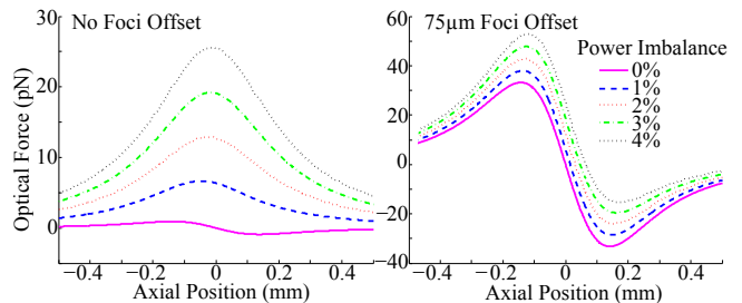
FIG. 2: (Color Online) Optical force along the laser axis with coincident foci (left) and offset foci (right) for various power imbalance between the S- and P- polarized beams. Power imbalance is defined so that e.g. 1% indicates 51% of the power is in the P- polarized beam. The total laser power is 2.2 \text{ W} and the waist is 9 \mu\text{m} .
