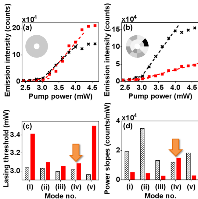
FIG. 4. (Color online) Emission intensity as a function of pump power for mode (iv) in panel (a) and mode (iii) in panel (b) under uniform ring pumping (black crosses) and non-uniform pumping to select mode (iv) (red squares). The insets show the intensity distribution of (a) uniform and (b) optimized pump profiles. (c,d) Lasing thresholds and power slopes under uniform pumping (patterned bars) or selective pumping (filled bars). The target mode (iv) becomes the dominant lasing mode even though its lasing threshold is not the lowest because adaptive pumping greatly suppresses the power slopes of the competing modes.
