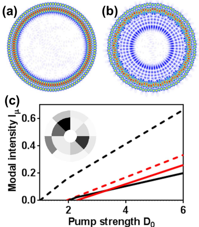
FIG. 7. (Color online) Numerical simulation of changing the power slopes of lasing modes by adaptive pumping of a microdisk with rough boundary. The disk radius is 3 \mu\text{m} , and the refractive index is 3.13. (a,b) Calculated spatial distribution of magnetic field ( |H_z| ) for two WG modes of second radial order, labeled mode 1 and 2, respectively. (c) Lasing intensity for these two modes with uniform ring pumping (dashed lines) and non-uniform pumping to make mode 2 stronger than mode 1 (solid lines). The optimized pump profile found by the Genetic Algorithm does not change the lasing order but greatly suppress the power slope of mode 1 (black lines).
