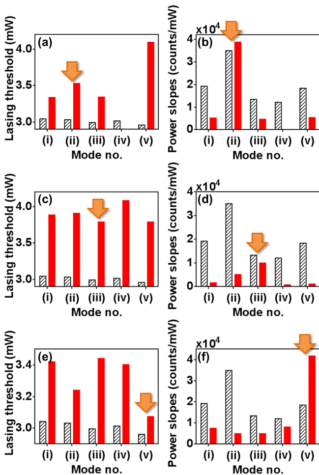
FIG. 5. (Color online) (a,c,e) Lasing thresholds and (b,d,f) power slopes for modes (i-v) after optimizing for mode (ii), (iii) and (v). Patterned bars represent the case for uniform pumping and filled bars for selective pumping. While the target mode not necessarily has the lowest lasing threshold, their power slope becomes the highest among all lasing modes.
