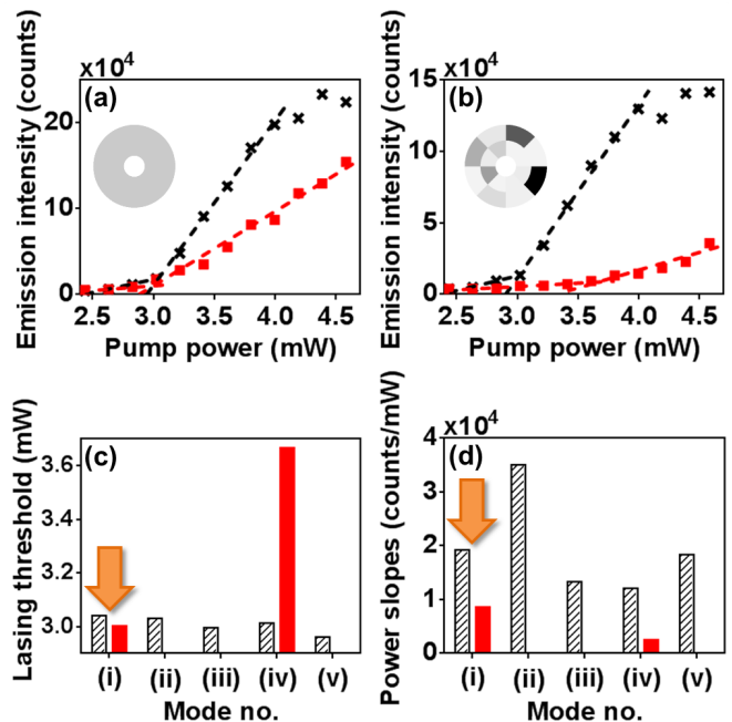
FIG. 3. (Color online) Emission intensity as a function of pump power for (a) mode (i) and (b) mode (iv) under uniform ring pumping (black crosses) and non-uniform pumping (red squares) to optimize mode (i). The insets show the intensity distribution of (a) uniform and (b) optimized pump profiles. Dashed lines represent the linear regression of the data points below and above the lasing threshold. The intersection of the two lines determines the lasing threshold pump power, and the slope of the line above the threshold gives the power slope of the lasing mode. (c,d) Lasing thresholds and power slopes for modes (i-v) under uniform pumping (patterned bars) and adaptive pumping (filled bars). Mode (i) becomes the dominant lasing mode because the inhomogeneous pumping suppress all other competing modes by greatly increasing their lasing thresholds.
