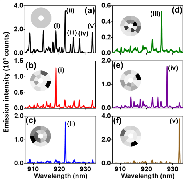
FIG. 2. (Color online) Lasing spectra with different pump patterns. (a) Under uniform ring pumping, many modes lase simultaneously. (b-f) Lasing spectra when modes (i-v) are target as the dominant lasing mode with adaptive pumping. Insets show the final optimized pump profiles in gray scales with darker color corresponding to higher intensity.
