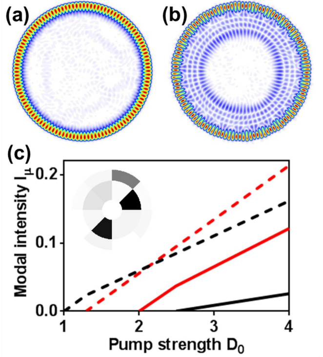
FIG. 6. (Color online) Numerical simulation of switching of lasing order by adaptive pumping of a microdisk with rough boundary. The disk radius is 3 \mu\text{m} , and the refractive index is 3.13. (a,b) Calculated spatial distribution of magnetic field ( |H_z| ) for two TE-polarized high- Q modes, labeled mode 1 and 2, respectively. Mode 1, at \lambda = 917.7 \text{ nm} , has Q factor of 1.20 \times 10^5 . Mode 2, at \lambda = 902.9 \text{ nm} , and Q = 1.09 \times 10^5 . Mode 1 in (a) consists predominantly of CCW propagating WG wave with radial number 1 and azimuthal number 57. Mode 2 in (b) is primarily a WG modes of radial number 1 and azimuthal number 58, but contains additional WG waves of higher radial order number 7 due to disorder-induced mode mixing. (c) Lasing intensity for mode 1 and 2 as a function of pump strength D_0 with uniform ring pumping (dashed lines) or non-uniform pumping to select mode 2 (solid lines). Mode 1 lases first before mode 2 with uniform pumping, but the lasing order switches, i.e., mode 2 lases first, with the non-uniform pump profile (inset) shown in the gray scale with darker color corresponding to stronger pumping. D_0 is normalized to the lasing threshold of mode 1 with uniform ring pumping.
