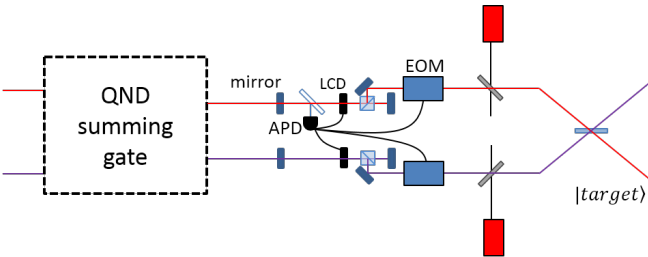
FIG. 4. (Color online) Repeat-until-success scheme in which a pulsed resource state remains in a cavity until a photon detection is registered.
