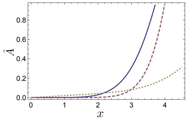
FIG. 1. (Color online) The effect of imperfect detectors is shown where the operator \hat{A} = U_N(\gamma) - e^{i\gamma\hat{x}^3} is the difference between the approximation and ideal cubic phase operators. The expectation value, both real (solid) and imaginary (dashed) parts, as well as the standard deviation (dotted) of this operator, in a position eigenstate |x\rangle , is plotted for \gamma = 0.03 [11, 21] and N = 1 . We consider a detector with an efficiency of 90%, a dark count rate of 100Hz and a timing resolution of 100ps; such a detector is within the reach of current technology [22–24]. We see that for small values of x the effect of detector imperfections on our approximate cubic phase gate are small and we still approximate the ideal gate closely.
