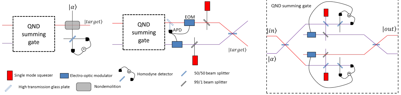
FIG. 3. (Color online) Experimental implementation of a single U_l operation in the cubic phase gate decomposition. Left: after application of the two-mode unitary a QND measurement is made to project onto the subspace orthogonal to |0\rangle\langle 0| . This could consist of an inverse V-STIRAP scheme via strong atomic coupling to a photonic cavity mode (cavity QED)[25], or via cross-phase modulation. However, in the case of cross-phase modulation a phase shift can be registered, but not its magnitude, in order to avoid projection onto a specific number state. Middle: After the QND measurement, the resource state is sent through a weak beam splitter and an avalanche photodiode registers a click to signal a photon-subtraction measurement. The QND summing gate is then run in reverse, where the photon detection triggers inverse operations on the phase modulators and squeezers compared to the original QND summing gate. If the squeezers in the inverse gate are kept phase locked to the first set in the previous measurement, homodyne detectors are unnecessary here as the APD serves as the conditional measurement and the squeezing angles are known, allowing for deterministic feed forward control. Right: the QND summing gate consisting of feed-forward phase modulation and offline squeezing resources.
