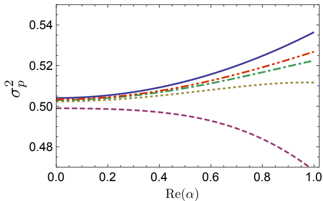
FIG. 2. (Color online) The variance \sigma_p^2 is plotted for the ideal (solid) cubic phase gate as well as U_N(\gamma) for N = 1 (dashed), 3 (dotted), 5 (dash-dot), 7 (dash-double dot); the strength of the gate is given by \gamma = 0.03 . The input state is chosen to be a coherent state with constant imaginary part \text{Im}(\alpha) = 0.25 where the real part varies with the horizontal axis. Additional squeezing, omitted in this plot, can be utilized to improve the strength or quality of the gate; here we are interested only in the differences as one varies N and we see that as N increases we obtain a closer approximation. Deviation from the ideal curve will result in extra variance in the momentum quadrature, compared to the ideal curve, after one squeezes the mode.
