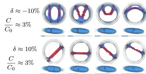
Figure 4. (Color online, movie in [12].) The trap on the top is wider than it is tall – the energetically favored configuration would be a vertical vortex, but the initial conditions lead to a slightly more energetic vortex aligned along the longer of the two axes. On the bottom, we imprint an oblique vortex line in a trap with the same asymmetry as the experiment. As it oscillates long the trap, the vortex alignment oscillates about the favored horizontal position, but without significant damping, continues past this alignment to another oblique position. The presence of significant damping – such as through phonons at finite T – might allow this to relax to a horizontal alignment. However this relaxation would likely be comparable to the time it takes the vortex to oscillate out of the system – the true “minimum” energy state has no vortex at all.
