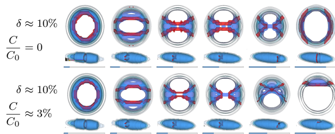
Figure 2. (Color online, movie in [12]) Effects of moderate anisotropy \delta = 1 - \omega_y/\omega_x \approx 10\% (trap is taller than wide): the ring hits the narrow walls on the side, forming two parallel vortices. Without any anharmonicity C = 0 (top), these undergo several recombinations, oscillating between a horizontal and vertical orientation. The presence of an anharmonicity C/C_0 \approx 3\% breaks the symmetry, eventually expelling one vortex from the system, resulting in a long-lived vortex that oscillates back and forth.
