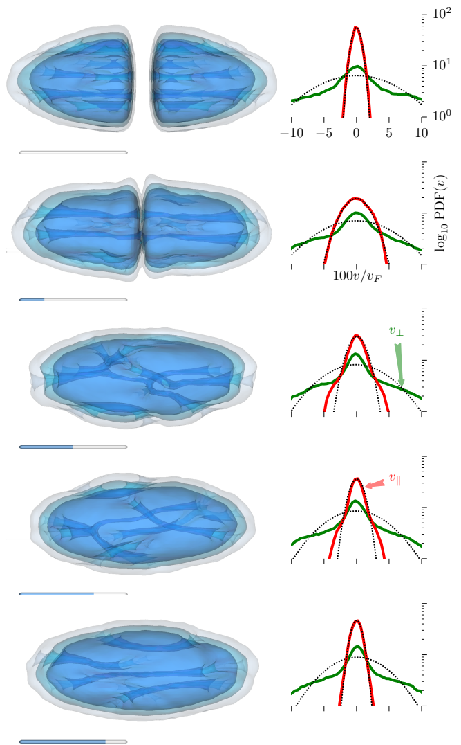
Figure 5. (Color online, movie in [12].) Generation of quantum turbulence by phase imprint of the vortex lattice. In the left column consecutive frames show: a) vortex lattice with knife edge dividing cloud, b) just after phase imprint removal of the knife, c-e) decay of turbulent motion. In the right column we show the corresponding PDFs for longitudinal v_{\parallel} and transverse v_{\perp} components of collective velocity. Dotted lines show the gaussian best fit to the data.
