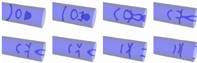
Figure 1. (Color online, movie in [12].) Demonstration of off-axis vortices in the UFG generated by firing a “bullet” along an axially symmetric trap in a movie from the simulations included with Ref. [6]. Off-axis vortex rings attach to the walls, and turn into vortex lines that cross and reconnect. The movie also demonstrates that vortex rings and lines move at similar velocities.
