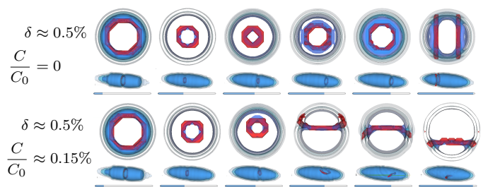
Figure 3. (Color online, movie in [12].) Effects of weak anisotropy: the ring now lives long enough to return as a small ring. Without an anharmonicity (top) several oscillations occur before the ring expands and hits the walls forming two parallel vortices. Adding a weak anharmonicity (bottom) causes the small ring to rotate. Once twisted off axis, this ring rapidly converts to a single vortex as seen in [7]. The rapid production of a single vortex from a twisted defect was also described in [17] and provides a convenient way of constructing vortices.
