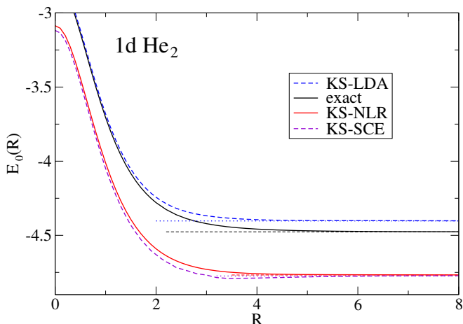
FIG. 13. (Lack of) binding for the 1d soft-Coulomb helium dimer. KS-SCE predicts a weakly bound state. Horizontal lines indicate twice the energy of a single isolated helium atom within each method.
