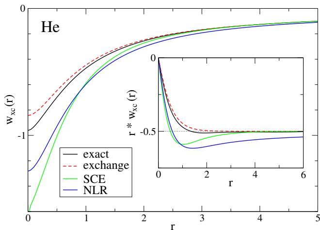
FIG. 3. The interaction XC energy per particle (41) as a function of the radius r for the exact 3d helium atom density [49]. Inset: r w_{\text{XC}}(r) to see asymptotic behavior. The exact w_{\text{XC}}(r) \rightarrow -1/(2r) as r \rightarrow \infty .
