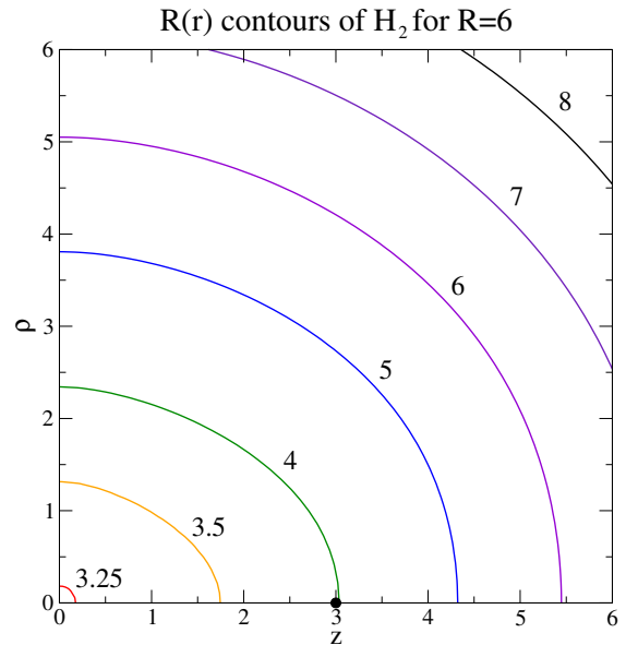
FIG. 2. Nonlocal radius R(\mathbf{r}) (32) for the exact density of the \text{H}_2 molecule with bond length R = 6 , in cylindrical coordinates (z, \rho) . Exact density is the Full-CI result from GAMESS-US [89] within the aug-cc-pV6Z [90] basis set. The bond-axis is along the z coordinate, and the nuclei are at z = \pm 3 .
