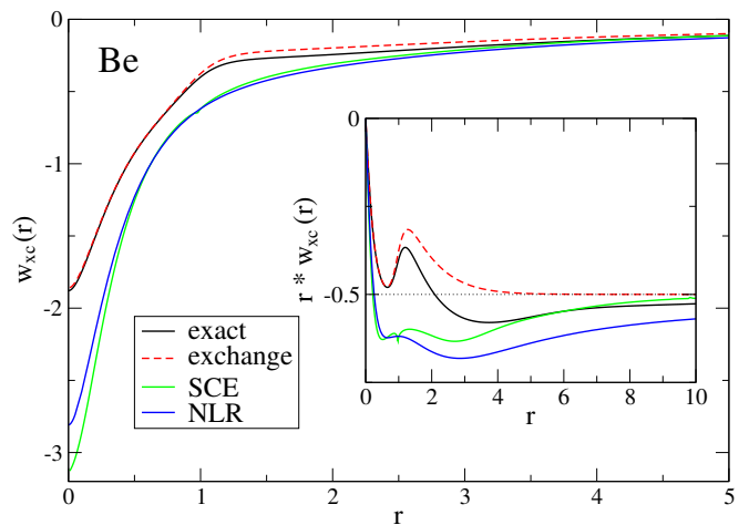
FIG. 5. The interaction XC energy per particle (41) as a function of the radius r for the exact 3d beryllium atom density [49]. Inset: r w_{\text{XC}}(r) . Notice that the SCE energy density physically has a kink near r = 1 , which has to do with classical electrons disappearing to infinity in the SCE method [49].
