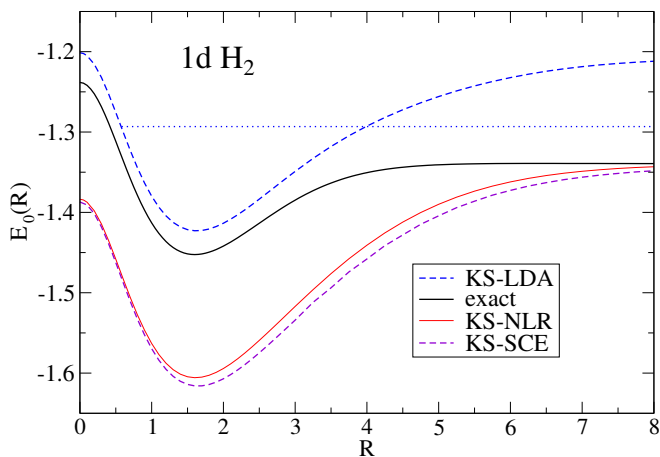
FIG. 12. The total molecular energy of 1d \text{H}_2 with soft-Coulomb interactions between all particles. Exact and KS-LDA data from Ref. [51]. The horizontal dotted line is twice the energy of a KS-LSDA hydrogen atom.
