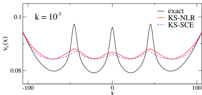
FIG. 11. KS potentials for the k = 10^{-5} system of Fig. 10.
