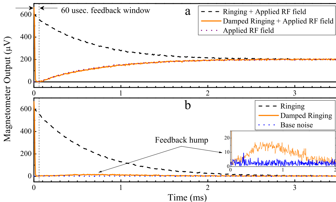
FIG. 6. (Color online) Plots (a) and (b) demonstrate the application of spin damping with the magnetometer initially in a perturbed state, a state created by a RF pulse of amplitude 1.13 pT applied for t \leq 0 . (a) The magnetometer response to a 0.37 pT RF signal, applied at t = 60 \mu\text{s} , is obscured by the transient ringing from the initial perturbed state (dashed line). Application of spin damping during a short window quickly eliminates the transient and permits the clear observation of the signal (solid line) as compared to when there is no initial perturbation (dotted line). (b) The ringing transient naturally decays with a time constant of T_2 = 0.7 ms (dashed line), but under damping, the transient decays in less than 60 \mu\text{s} (solid line). However, due to inhomogeneity in B_0 across the K cell, a small feedback hump arises after the damping field is turned off.
