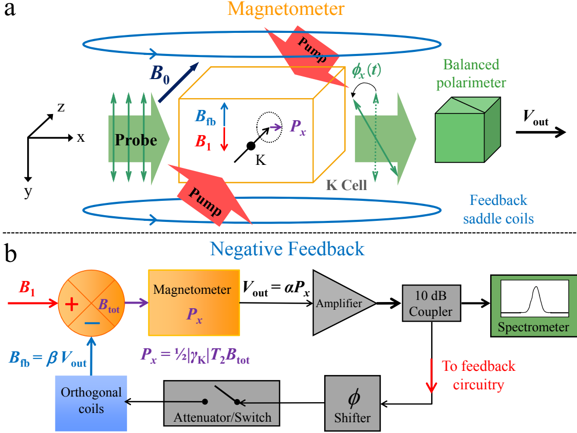
FIG. 1. (Color online) Experimental set-up (a) and schematic (b) of the spin-damping mechanism. A perturbing magnetic field B_1 sets the optically pumped K atoms precessing around B_0 . The resulting transverse atomic polarization P_x rotates the probe beam's polarization, which is detected and converted to an electrical signal V_{\text{out}} by a balanced polarimeter. Part of this electric signal is phase corrected and fed back through electromagnetic saddle coils to produce a damping field B_{\text{fb}} that is anti-parallel to B_1 , resulting in an active damping of the K transverse polarization. The strength of the damping is characterized by the open loop gain, D = \alpha\beta P_x \gamma_K / 2 .
