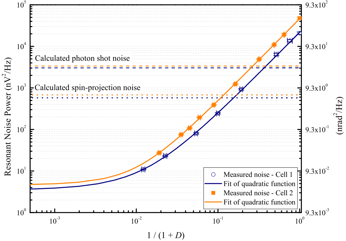
FIG. 4. (Color online) For cell 1 (open navy circles) and cell 2 (solid orange squares), the plot of resonant noise power A_n^2 as a function of suppression, fitted to a quadratic polynomial (solid lines). The values of all parameters for the two cells are given in Table I.
