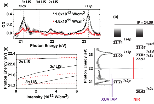
FIG. 3: (Color online) Experimental transient absorption spectra. (a) Line spectra at a pump-probe delay of -2.7 fs for intensities of 1.6 \times 10^{12} W/cm ^2 (black) and 4.8 \times 10^{11} W/cm ^2 (red). Error bars represent \pm\sigma . (b) Schematic energy level diagram for excitation of light induced states. Line absorption spectrum measured with overlapped NIR and IAP pulses is shown in black. Peaks in the absorption spectrum around 22 eV, 21.6 eV and 21.25 eV clearly do not result from excitation to dipole-allowed 1snp levels. LISS couple the ground state to 1sns and 1snd states via absorption of one XUV photon (purple) and absorption or emission of one NIR photon (red). (c) Calculated positions of 2s , 3d and 3s LIS versus NIR intensity for a delay of -2.7 fs. Full calculations (solid black lines) are compared to three-level model calculations (dashed red lines).
