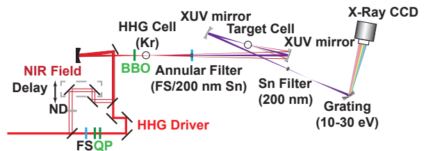
FIG. 1: (Color online) Experimental setup. Schematic of attosecond transient absorption instrument. ND: neutral density filters; FS: fused silica; QP: quartz plates. Optics for double optical gating are shown in green. IR beam paths are shown in red. IAP is shown in purple.
