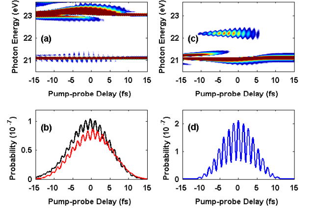
FIG. 4: (Color online) (a) Same as Fig. 2(b) but with the 1s2s , 1s3s and 1s3d states all subtracted out during the time propagation. (b) Calculated integrated absorption probability around the 22.2 eV LIS in Fig. 2(b) (black) and the final 2s population (red) versus the pump-probe delay. (c) Three level model of the response function \tilde{S}(\omega) near the 2s LIS with the 1s^2 , 1s2p and the 1s2s states included. The XUV and NIR pulses are the same as in the full calculations in Fig. 2(b). (d) 1s2s population at the end of the pulses in the three level model of part (c). Note that the units in (b) and (d) are the same, without any modification of the original data.
