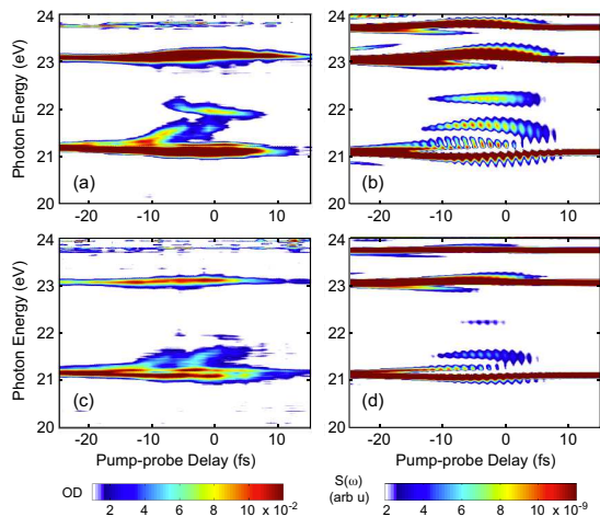
FIG. 2: (Color online) Experimental transient absorption spectra (left panels) and calculated single atom frequency-dependent response (right panels) as a function of pump-probe delay. Negative delays indicate that the NIR pulse follows the IAP. The peak NIR intensity is (a, b) 1.6 \times 10^{12} W/cm 2 , and (c, d) 4.8 \times 10^{11} W/cm 2 . The theoretical plots use a small, non-zero value of the minimum response to better mimic the experiment. The 1s2p resonance is at 21.21 eV and the 1s3p resonance is at 23.09 eV.
