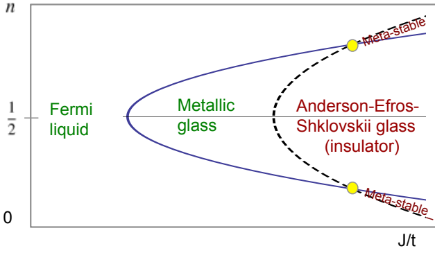
FIG. 2: (Color online) Schematic phase diagram of Eq. (1) for small effective onsite disorder ( \bar{W} = 0 ) as a function of fermion density n . Below the crossing point (yellow dot) of the metal-insulator transition (black-dashed line) and the glass transition (blue), the transition becomes first order. The Fermi liquid and the metallic glass may still exist (as long-lived metastable states) to the right of the dashed line.
