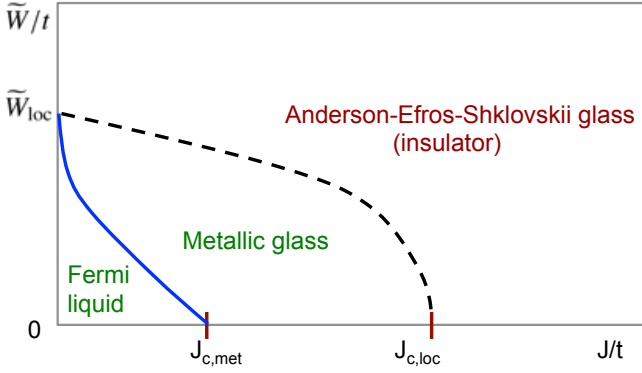
FIG. 1: (Color online) Schematic phase diagram of model (1) for moderate densities in the vicinity of half-filling n \approx 1/2 . J^2 is the variance of the long-range disorder V_{ij} , and \bar{W}^2 the variance of the effective onsite disorder, Eq. (26). The black, dashed line is the metal-insulator transition. The blue line is the glass transition. Quantitative computations in this paper are restricted to the \bar{W} = 0 axis, while the nature of the transition lines around the Anderson transition ( J = 0 ) are inferred from scaling considerations in Sec. VI. The localization transition from the metallic glass to the Anderson-Efros-Shklovskii glass and the signatures of this insulating glass phase are discussed in Sec. III. We describe the Fermi liquid to metallic glass transition and the properties of the metallic glass phase in Sec. V.
