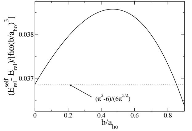
FIG. 2: For two opposite spin fermions interacting in 3D via a potential of short range b in an isotropic harmonic trap, the self-consistent equation (159), derived e.g. in [167], gives the eigenenergies with an error of order b^3 , due to the fact that it neglects the effect of the harmonic trap within the interaction range, see Appendix D. This is illustrated with the ground state relative energy for a square-well potential of infinite scattering length: The deviation (solid line) between the approximate energy E_{\text{rel}}^{\text{self}} [solving Eq. (159)] and the exact one E_{\text{rel}} (calculated as in [113]) vanishes as b^3 , with a coefficient given by Eq. (162) (dotted line). \mu is the reduced mass, \omega is the angular oscillation frequency in the trap and a_{\text{ho}} = [\hbar/(\mu\omega)]^{1/2} .
