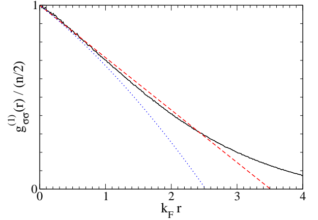
FIG. 4: (Color online) One-body density matrix g_{\sigma\sigma}^{(1)}(r) = \langle \hat{\psi}_{\sigma}^{\dagger}(\mathbf{r})\hat{\psi}_{\sigma}(\mathbf{0}) \rangle of the homogeneous non-polarized unitary gas at zero temperature: comparison between the fixed-node Monte Carlo results from Ref. [106] (black solid line) and the analytic expression (180) for the small- k_F r expansion of g_{\sigma\sigma}^{(1)} up to first order (red dashed straight line) and second order (blue dotted parabola) where we took the value \zeta = 0.95 extracted from the Monte Carlo data for g_{\uparrow\downarrow}^{(2)} , see Fig. 3.
